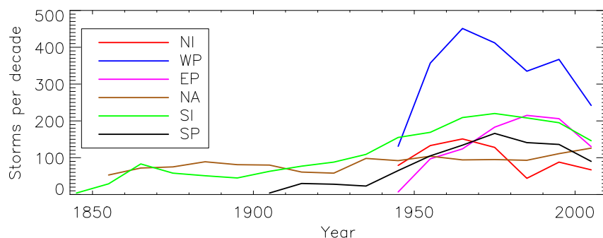
Figure 1 – IBTrACS inventory of tropical cyclones per decade sorted by genesis basin
