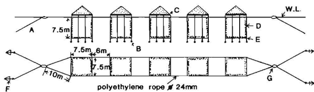
Figure 5.—Yellowtail mariculture facilities in embaymental farming ground. A, polyethylene rope, \phi 24 mm, n 3; B, stone, 7-8 kg; C, bamboo frame; D, polyethylene fiber, 400 d /40, 7 knot; E, frame line, \phi 10 mm; F, anchor 50 kg; G, styrol float, \phi 56 cm, length 90 cm, buoyancy 200 kg.
