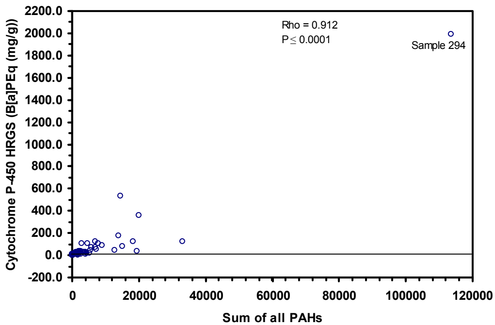
Figure 26. Relationship between cytochrome P450 HRGS response and the total of all polynuclear aromatic hydrocarbons in southern Puget Sound sediments sampled during 1999.
