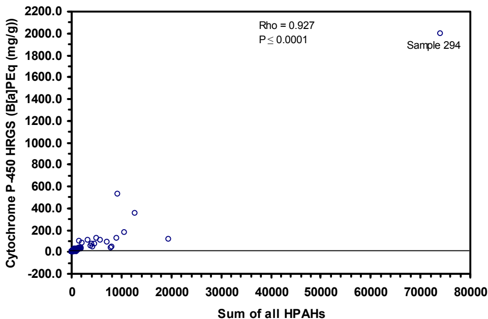
Figure 25. Relationship between cytochrome P450 HRGS response and the sum of all high molecular weight polynuclear aromatic hydrocarbons in southern Puget Sound sediments sampled during 1999.
