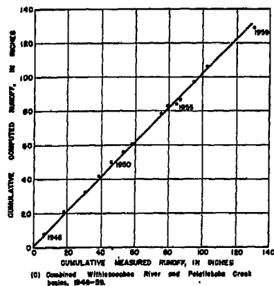
Figure 16. Double-mass curves of measured runoff versus computed runoff, Withlacoochee River and Palatka Creek basins.
