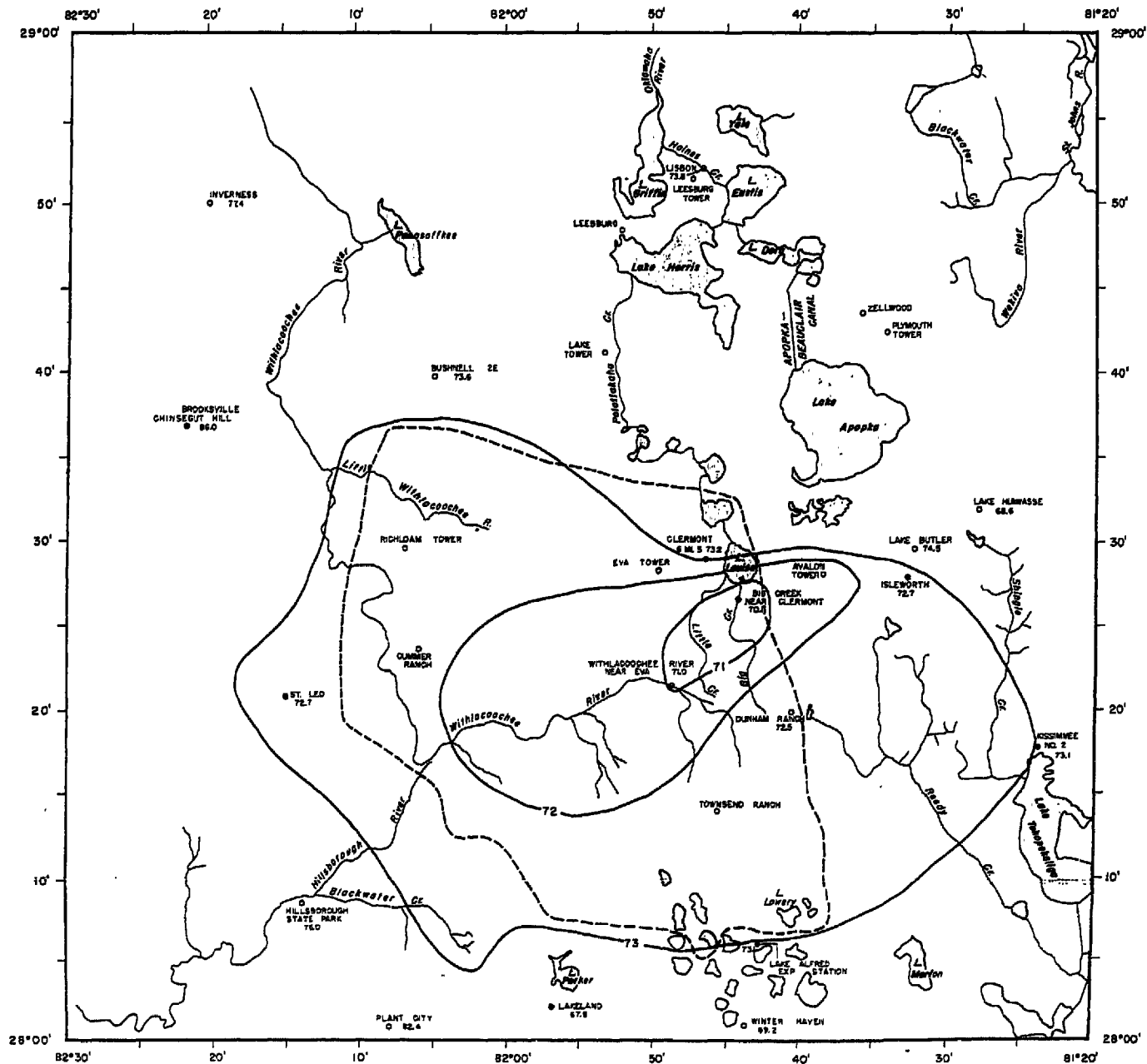
Figure 4. Map of Green Swamp area showing isohyets for 1959 water year and principal streams draining the area.
