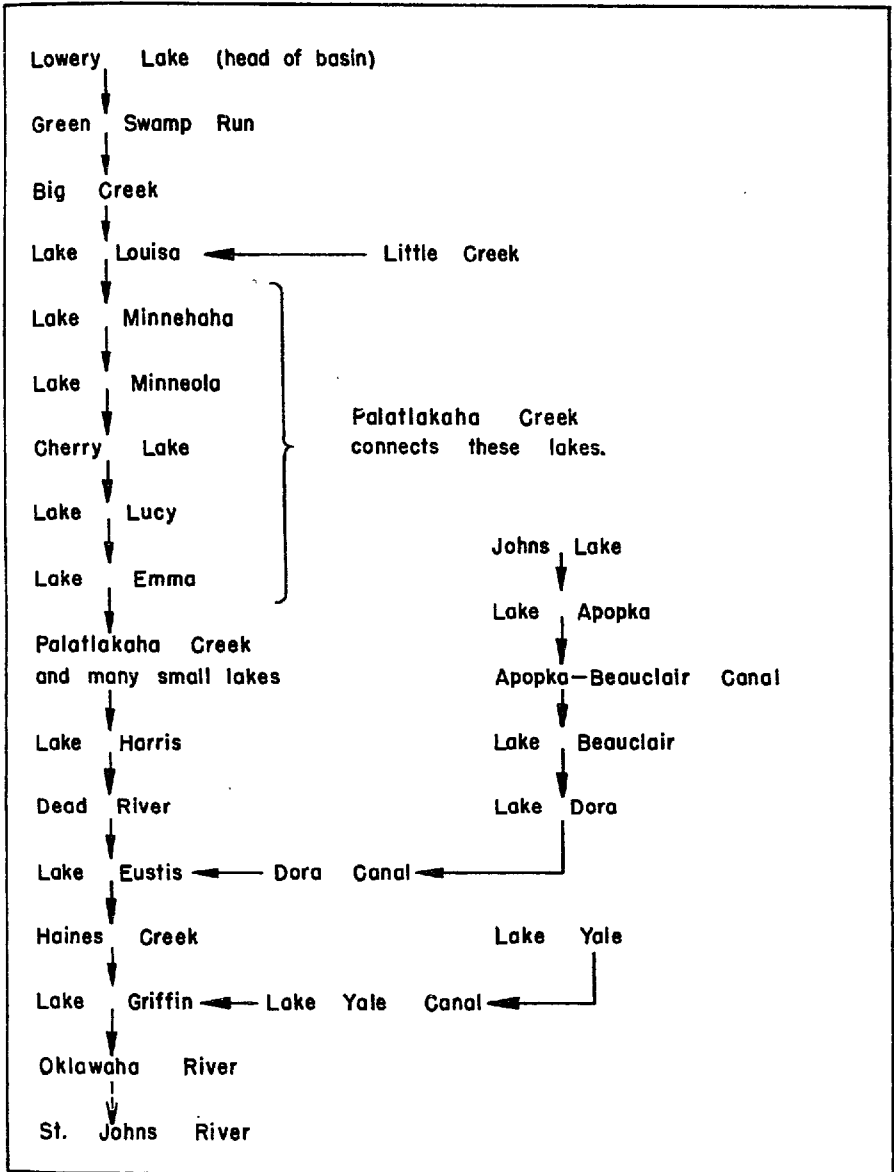
Figure 8. Flow diagram of the upper Oklawaha River.
