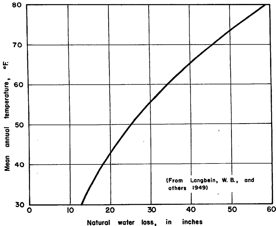
Figure 5. Relation of annual water loss in humid areas to temperature.
