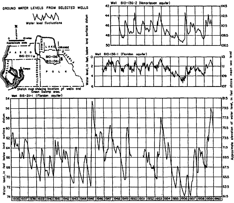
Figure 20. Hydrographs of long-term water-level records from wells near the Green Swamp area.
