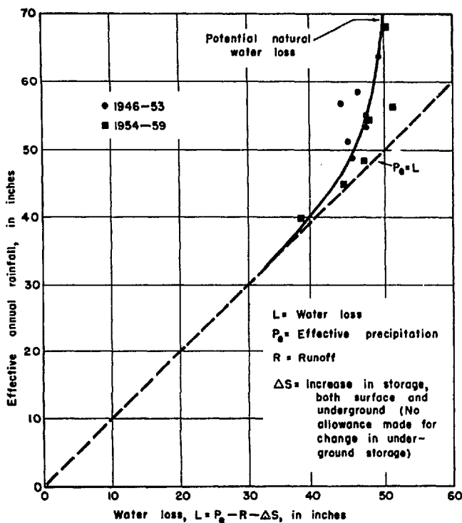
Figure 14. Relation of effective annual rainfall and annual water loss, Palatlahaha Creek above Mascotte, Florida, 1946-59.
