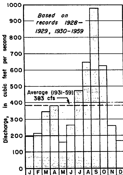
Figure 10. Average monthly discharge of Withlacoochee River at Trilby, Florida.
