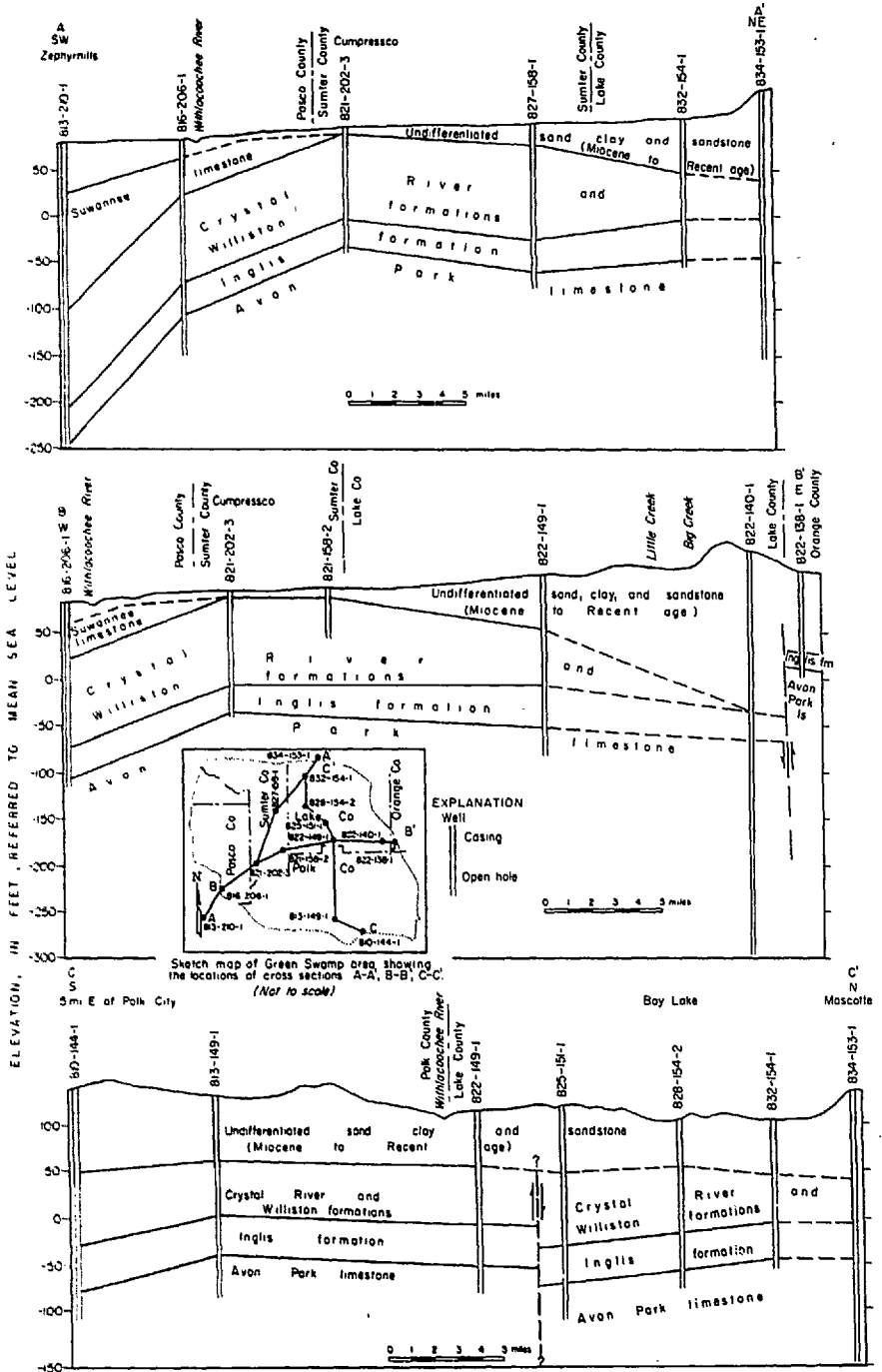
Figure 6. Generalized geologic cross sections across the Green Swamp area and their locations.
