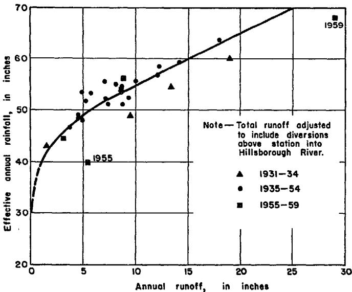
Figure 13. Relation of effective annual rainfall and annual runoff, Withlacoochee River at Trilby, Florida, 1931-59.
