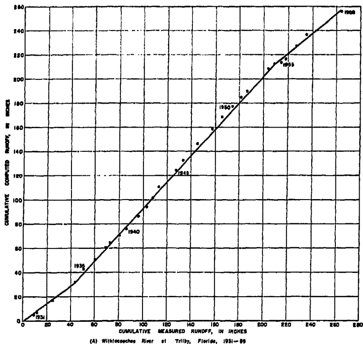
Figure 16. Double-mass curves of measured runoff versus computed runoff, Withlacoochee River and Palatka Creek basins.
