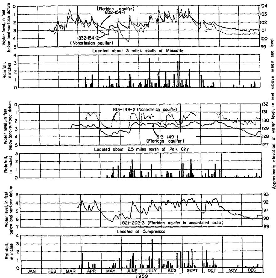
Figure 21. Hydrographs of water-level and rainfall records at wells in the Green Swamp area.
