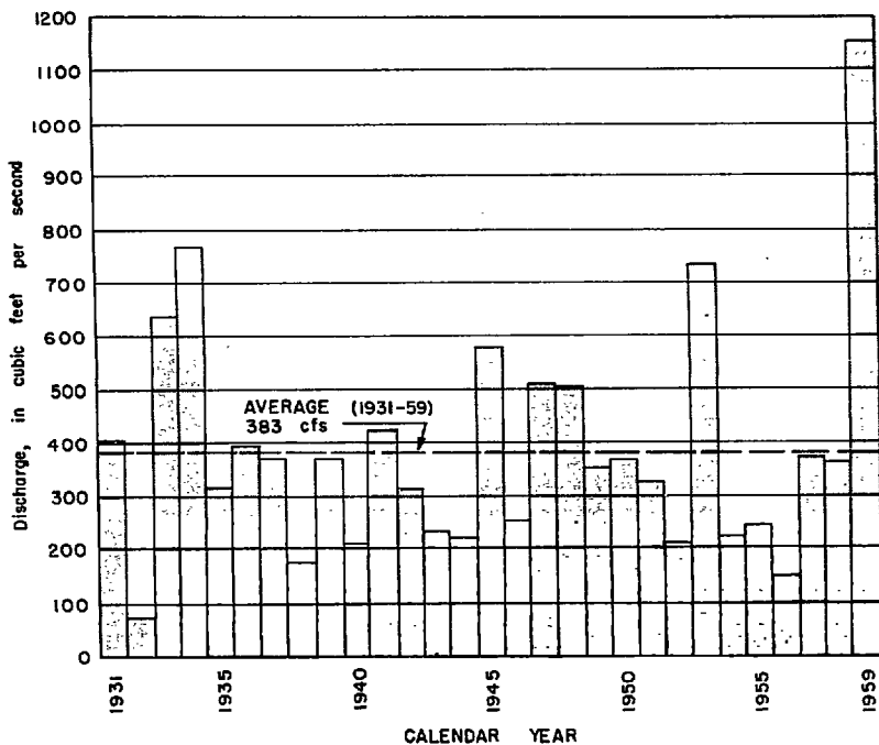
Figure 9. Annual discharge of Withlacoochee River at Trilby, Florida.
