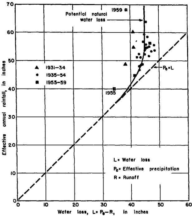
Figure 12. Relation of effective annual rainfall and annual water loss, Withlacoochee River at Trilby, Florida, 1931-59.
