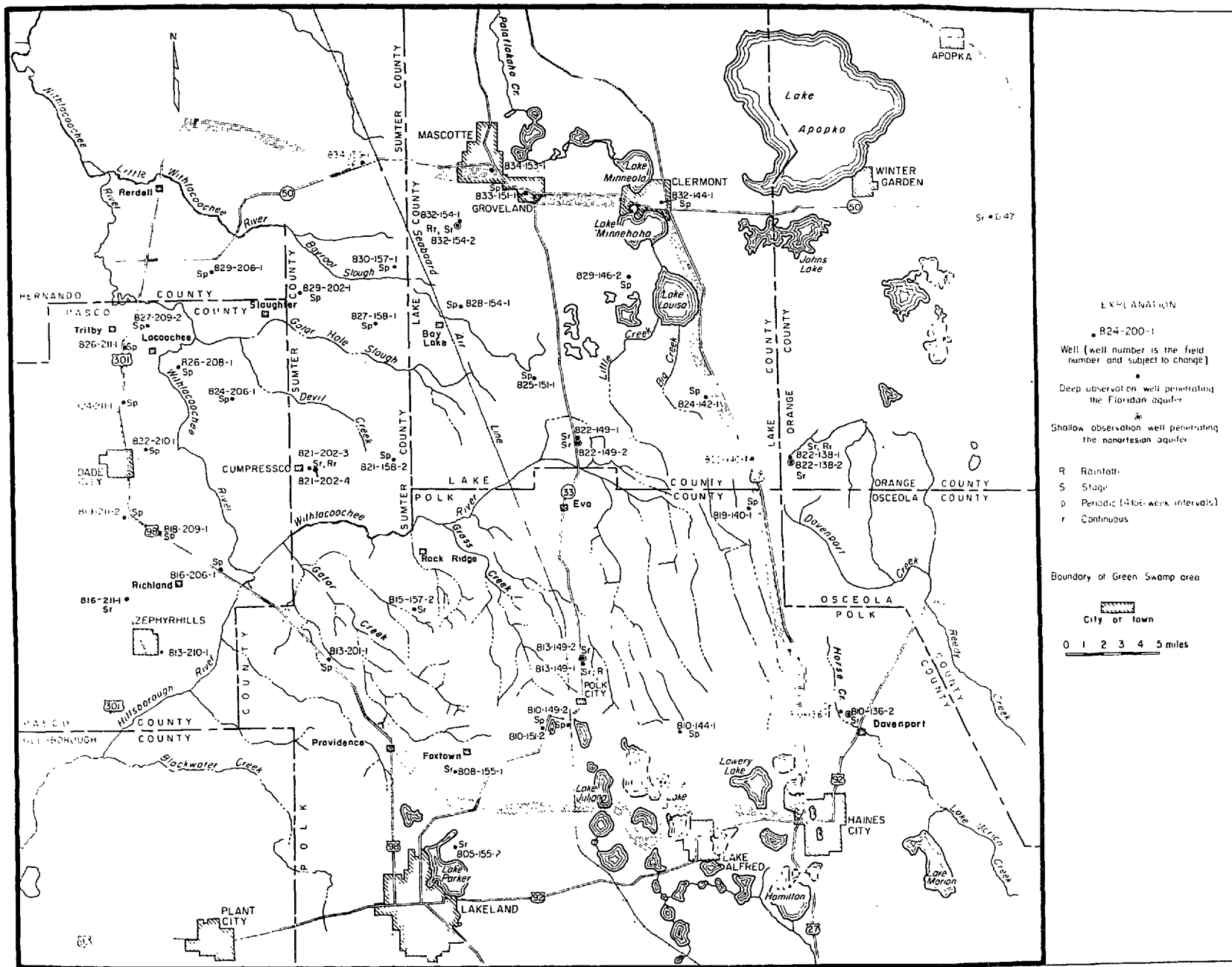
Figure 19. Map of Green Swamp area showing ground-water data-collection points.
