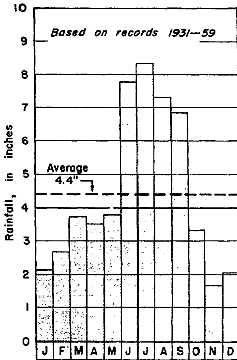
Figure 2. Average monthly rainfall of Green Swamp area.
