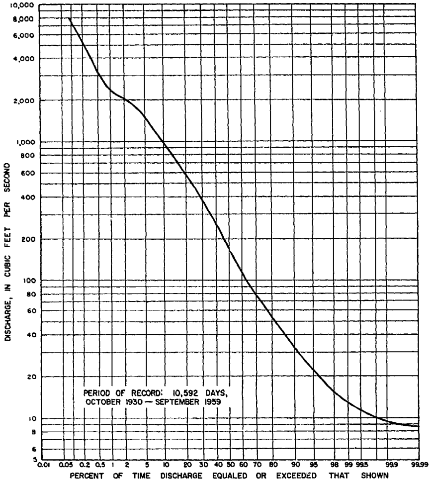
Figure 11. Flow-duration curve of Withlacoochee River at Trilby, Florida.
