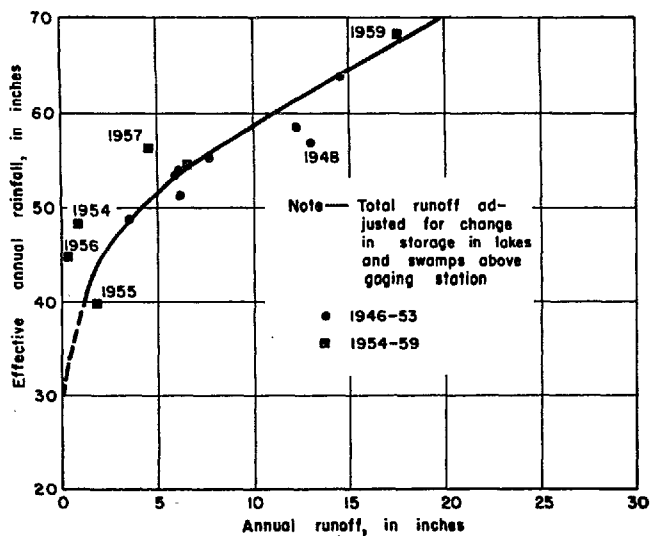
Figure 15. Relation of effective annual rainfall and annual runoff, Palatlahaha Creek above Mascotte, Florida, 1946-59.
