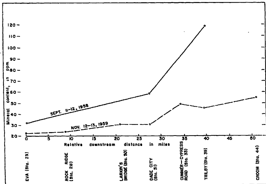
Figure 17. Mineral content in the Withlacoochee River.
