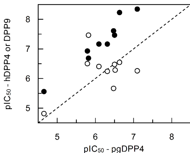
Figure 4: selectivity of the most potent compounds of the screening
