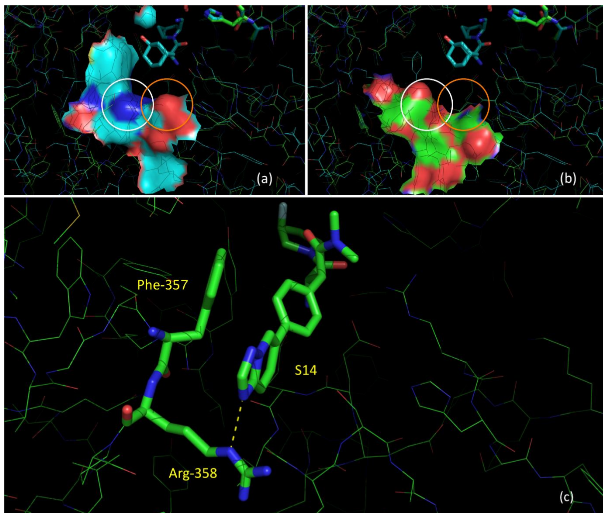
Figure 3: the S2 extensive pocket
