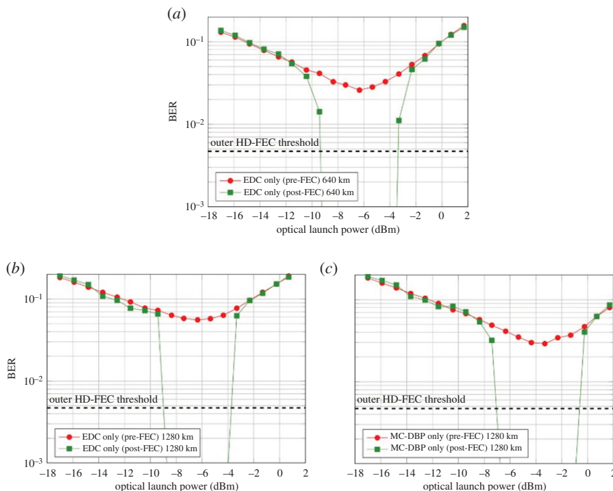
Figure 8. Pre- and post-FEC BER as functions of launch power for the central subchannel. (a) EDC only after 640 km of SSMF ( R_{SD} = 5/6 ), (b) EDC only after 1280 km of SSMF ( R_{SD} = 3/4 ) and (c) MC-DBP after 1280 km of SSMF ( R_{SD} = 5/6 ).
