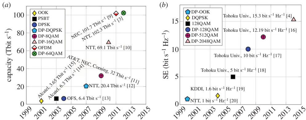
Figure 1. (a) Capacity and (b) SE growth demonstrated in state-of-the-art laboratory and research experiments around the world. It should be noted that figures for SE are difficult to compare as experiments are performed over different bandwidths but the trend is interesting nonetheless [3,4,9–20].
