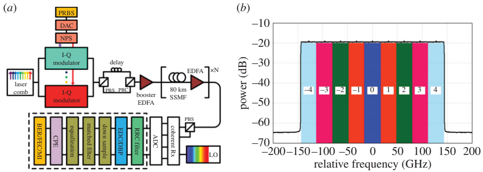
Figure 2. (a) Schematic of 9-channel DP-64QAM superchannel transmission system using the EDC or MC-DBP and (b) simulated transmission spectrum and the schematic of backpropagated bandwidth in the 9-channel DP-64QAM superchannel transmission system, where the frequency 0 Hz refers to the central frequency of the optical carrier (wavelength of 1550 nm). (PBS, polarization beam splitter; PBC, polarization beam combiner; NPS, Nyquist pulse shaping).
