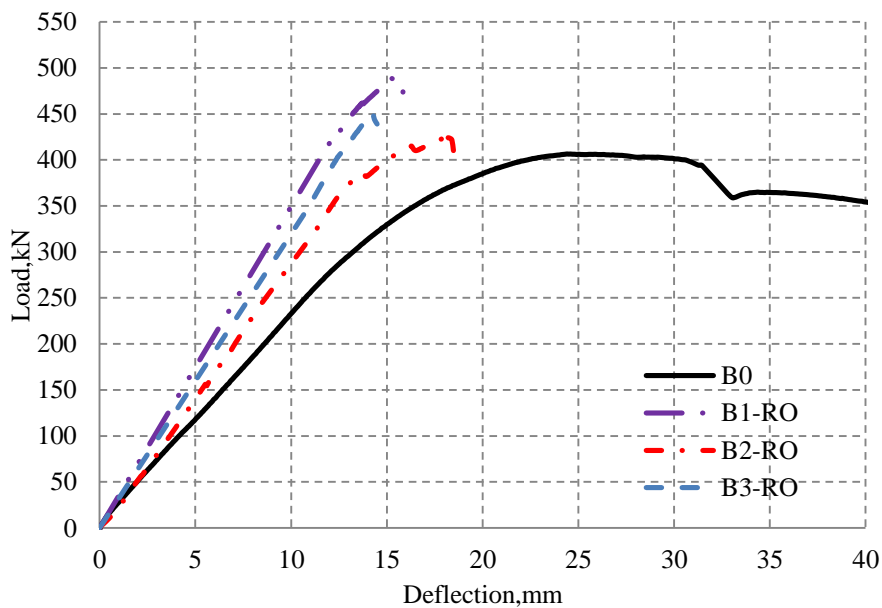
Figure 10 Load versus vertical displacement at mid-span for specimens B0 & B1-RO to B3-RO.
