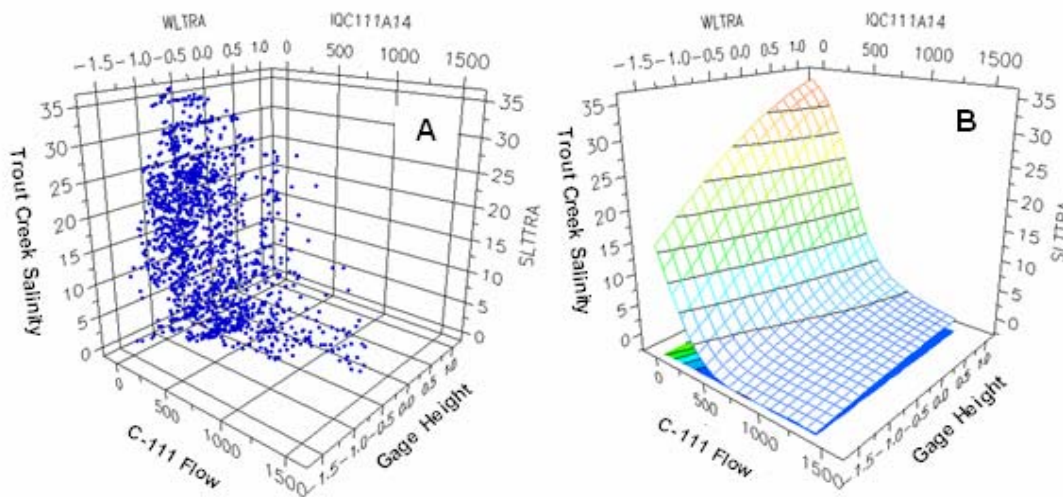
Figure 1. Three-dimensional scatter plot (A) of Canal 111 flow and Trout Creek gage height and salinity and three-dimensional response surface (B) generated by ANN model of the system.
