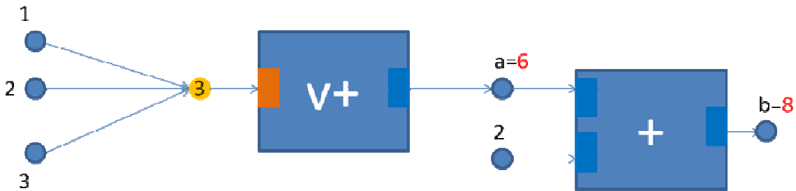
Figure 4.7: Graphical representation of the semantic graph of a simple closure chain
