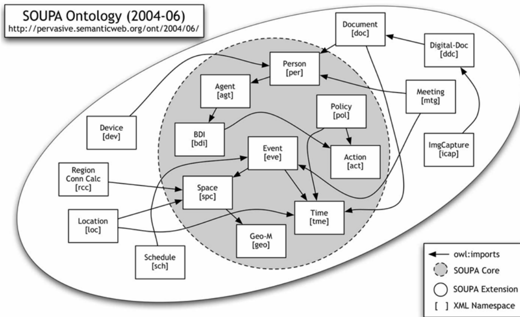
Figure 2.11: SOUPA ontology
