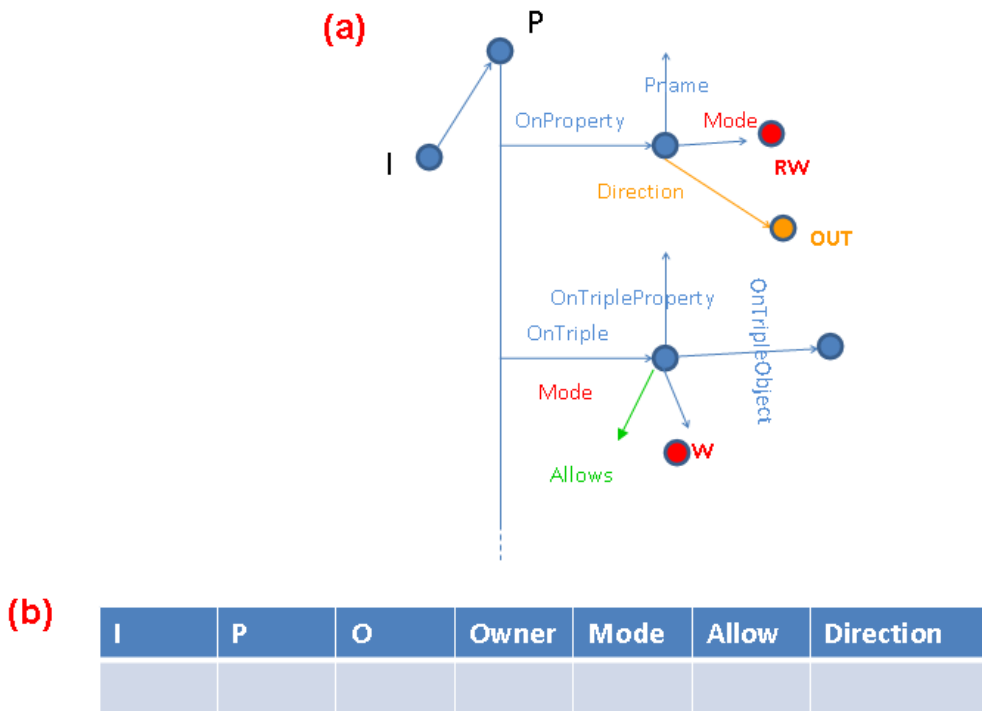
Figure 4.5: Proposed extension of the semantic model for access control (a) and LCT (b)
