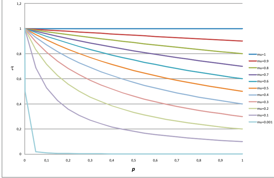
Figure 1: \tau as a function of p for various values to \mu (mu)
