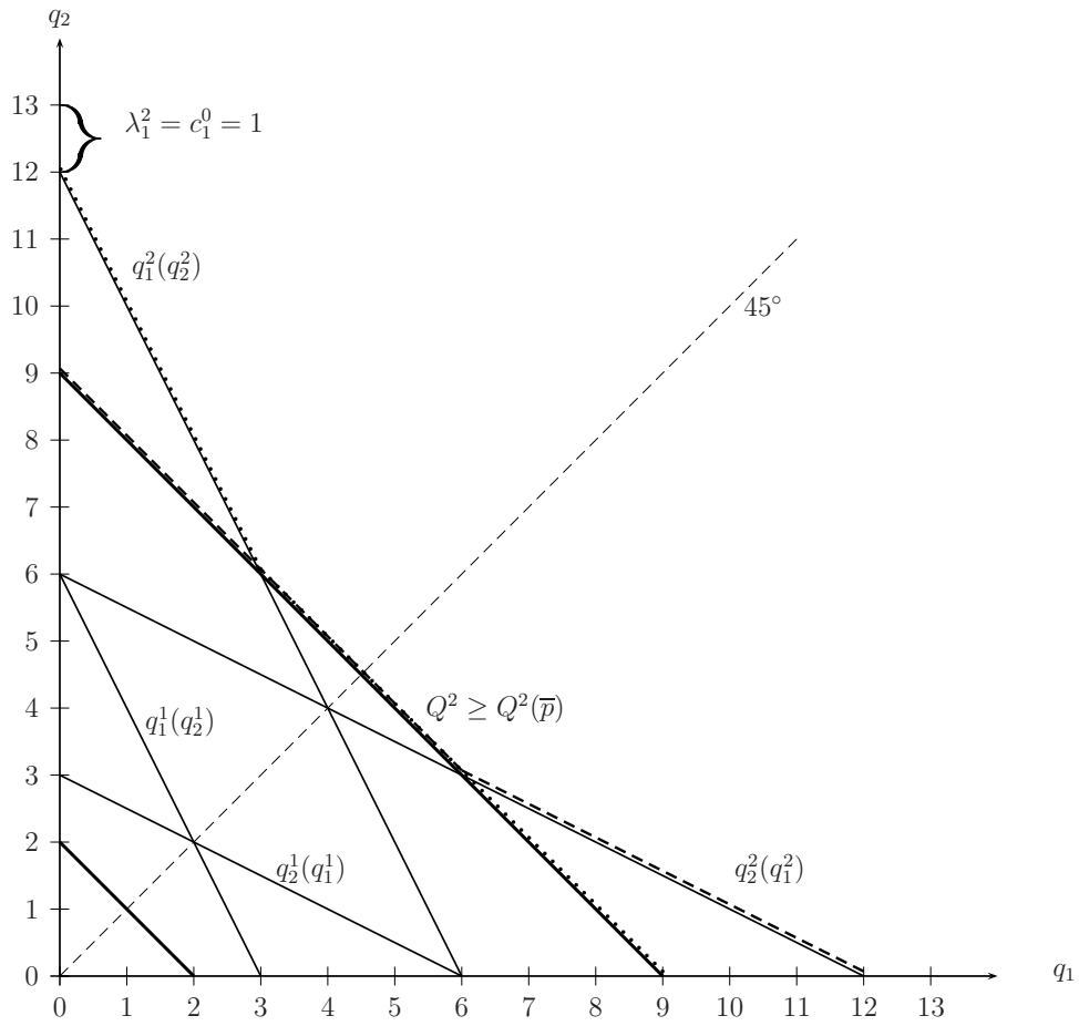
Figure 1: Best-response functions
