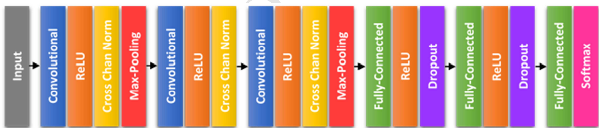
Figure 5: Layers of proposed CNN architecture.
