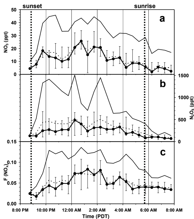
Fig. 4. Study average nocturnal variation in (a) NO 3 (b) N 2 O 5 and (c) F(NO x ) – partitioning of nitrogen reservoir species (see Eq. 2) Shown are the average (dotted line), median (solid point), 95th (solid line), 75th (top whisker) and 25th percentiles (bottom whisker) in each 30 min time bin.
