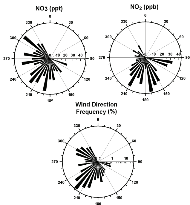
Fig. 6. Chemical and wind rose plots for (a) NO 3 mixing ratio (b) NO 2 mixing ratio and (c) frequency of winds, vs. wind direction. For all three plots, only data with coincident wind speeds >2 \text{ km h}^{-1} was included. For (a) and (b) radial direction represents the 95th percentile of the group of observations in each 10° bin. Note the log scale for panel (c).
