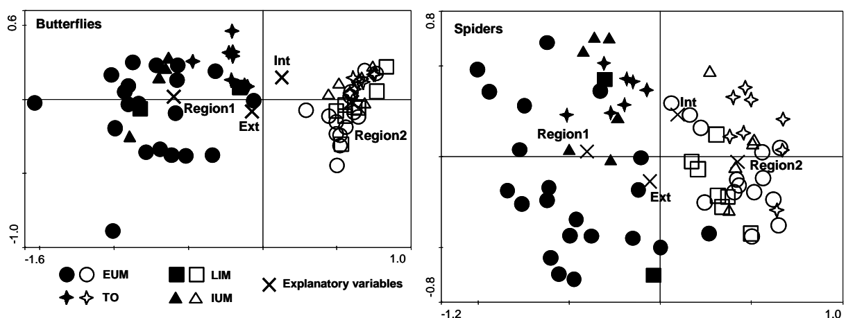
Figure 1. RDA ordination diagram of the sites based on butterfly and spider assemblages with management intensity and region variables displaying 21 % of the variance for spiders and 38 % for butterflies (first and second axes). Filled symbols: region 1; empty symbols: region 2. Ext = extensively used, Int = intensively used. See text for further explanation of meadow types.
