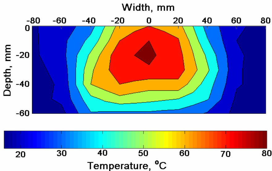
Figure 2. Soil temperatures from a cross-section across the groove, measured 40 sec. after treatment. The width is measured from centre of the treated band. Treated area: With -30 - +30 , depth 0 - 50 mm.
