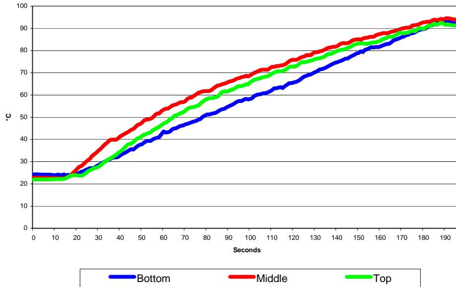
Figure 3. Soil temperatures measured at three levels in the soil during the steaming process
