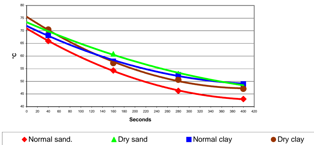
Figure 4. Temperatures in the steamed band from 40 to 400 s after the end of the steaming in four different soil types
