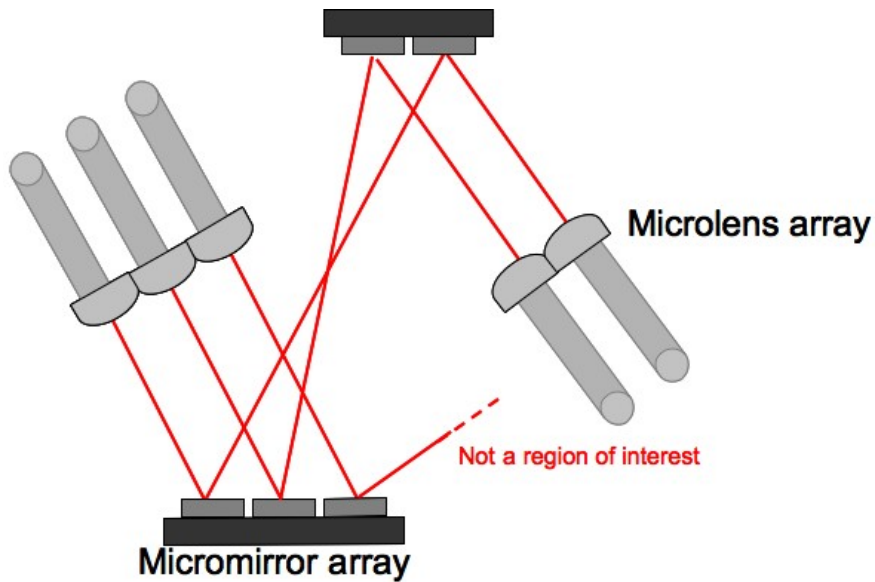
Figure 6.15: Simple switch using micromirror arrays
