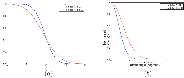
Figure 3.3: For a fibre with a core diameter of 100 \mu\text{m} and d_0 = 148.1\text{m}^{-1} if the wavelength is varied between \lambda = 450 - 700\text{nm} , for (a) a slow input angle of \theta = 10^\circ the output angle varies between 10.5 and 11.7, for (b) a slow input angle of \theta = 1^\circ the output angle varies between 4.1 and 6.4. Clearly the dependence with wavelength must be investigated at slow input angles.
