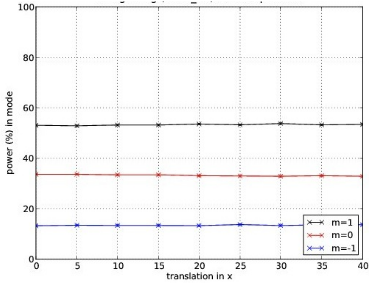
Figure 5.11: The homogeneity of Proto-1 was tested by creating a smaller aperture and testing the efficiency in each of the orders at different positions on the substrate. Errors on values are below 1%
