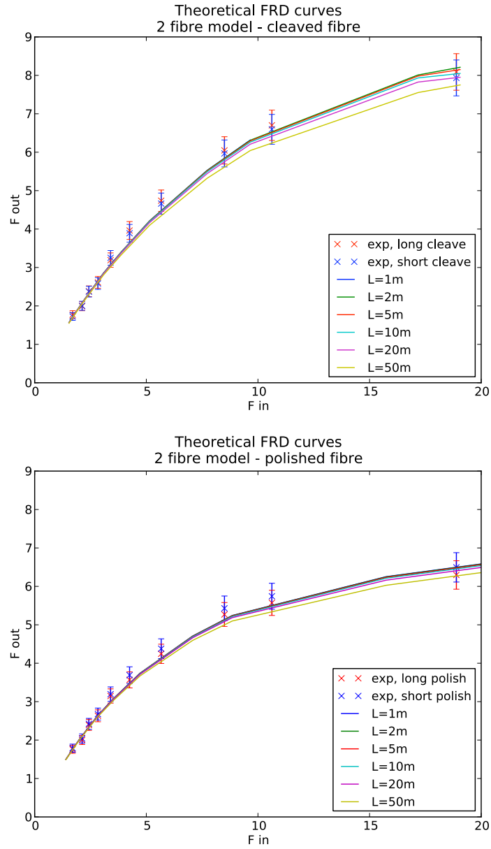
Figure 3.24: 2 fibre model results with d_{0,1} = 0.1 \text{ m}^{-1} and d_{0,2}L_2 = 25 for the cleaved fibre and d_{0,2}L_2 = 48 for the polished fibre. It is clear that within the errors the length dependence of the original model has been removed.
