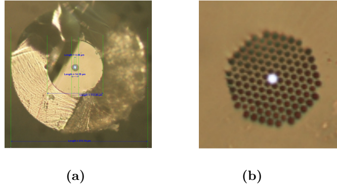
Figure 4.3: Results of cleaving a PCF. (a) a good finish can be achieved with a high level of skill (dimensions: holey region diameter = 14.9\mu\text{m} , cladding diameter = 121\mu\text{m} , buffer diameter = 277\mu\text{m} , (b) Microscope image of the end face shows that all of the holes are clear and undamaged, however the out of focus regions around the outer ring of holes shows that the end is not flat. The fibre was illuminated with diffuse white light at the input and is well guided at the output however it may not be aligned with the optical axis due to the end not being perpendicular to the length of the fibre.
