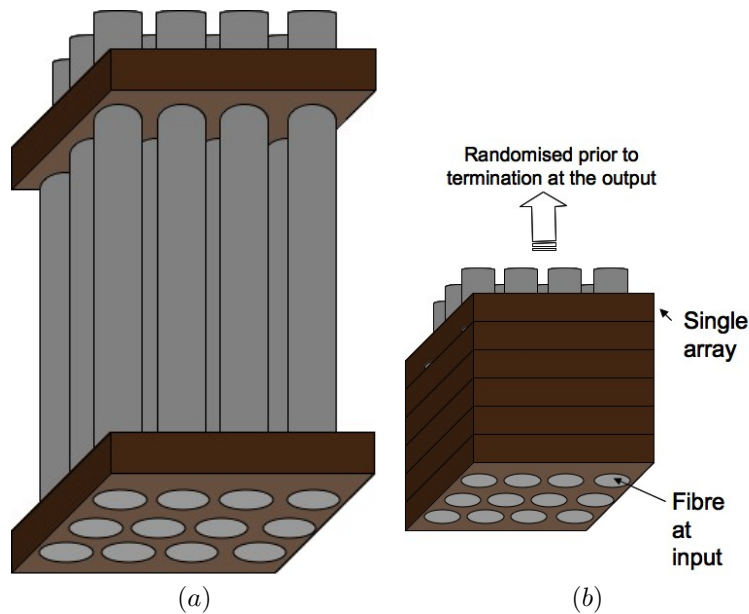
Figure 6.9: Due to the manufacturing methods, the arrays can only be made from relatively thin wafers of material and must be stacked in order to ensure that all fibres are able to be aligned to the optical axis.
