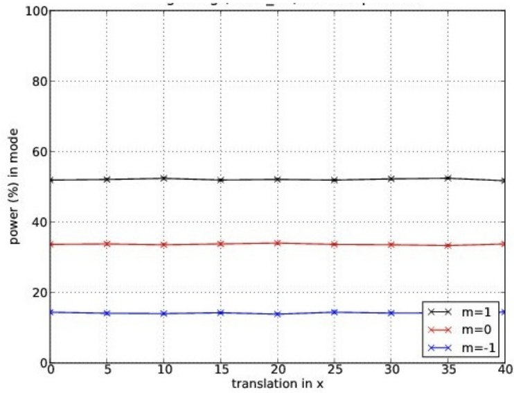
Figure 5.12: The homogeneity of Proto-2 was tested by creating a smaller aperture and testing the efficiency in each of the orders at different positions on the substrate. Errors on values are below 1%
