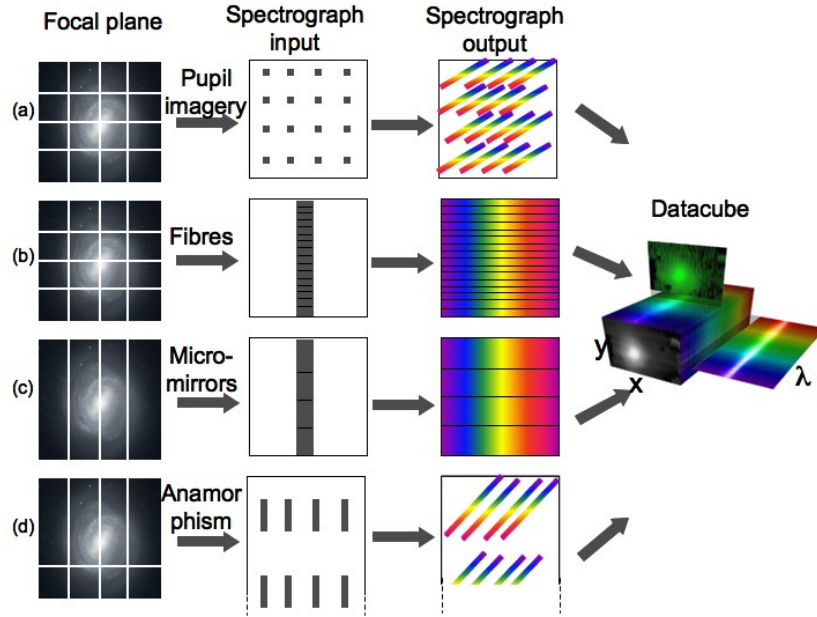
Figure 2.3: The main techniques of Integral Field Spectroscopy (image courtesy of Jeremy Allington-Smith [22])
