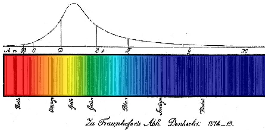
Figure 1.6: The first example of Quantitative Spectroscopy was made in 1814 when Joseph von Fraunhofer mapped 324 of the Solar Lines.
