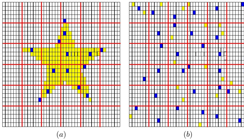
Figure 6.17: Illustration of how remapping affects the success of a switching network. Panel (a) shows the regions of interest in yellow where spaxels which will be successfully routed to the spectrograph are shown in blue, if M=1 with direct mapping. Panel (b) shows the improved success rate if M remains equal to 1 but the field is randomised prior to down-selection.
