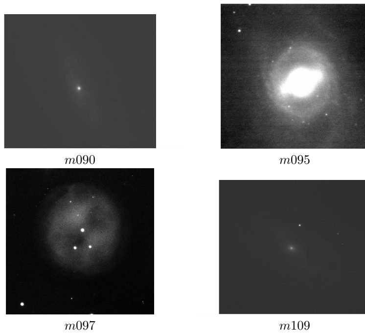
Figure 6.19: (Continued) The final four Messier objects with various amounts of clustering, used to test different remapping schemes.
