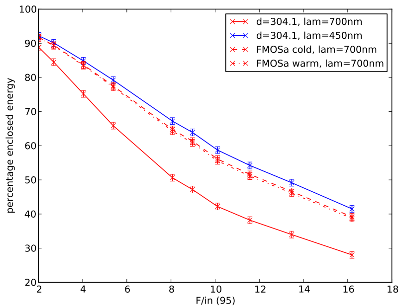
Figure 3.11: If the d_0 parameter is fit for the fibre at 450 nm a value of d_0 = 304.1 \text{ m}^{-1} is obtained. The solid red line shows the model predictions of the enclosed energy using the same parameters at \lambda = 700 \text{ nm} and the dashed lines show the actual enclosed energy obtained experimentally. Clearly, the model is predicting more FRD at longer wavelengths than is experimentally observed.
