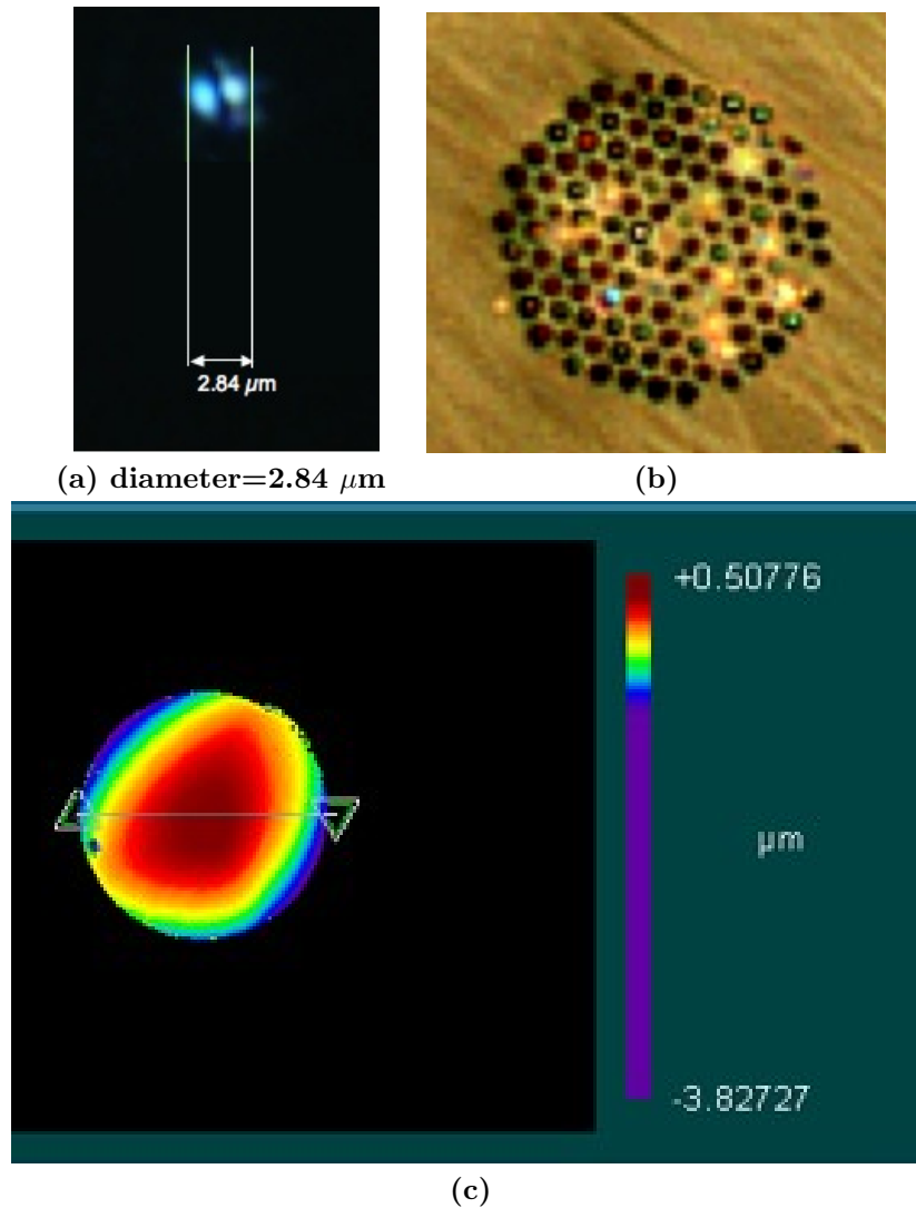
Figure 4.2: Results of polishing a PCF. (a) Output distribution when uniform white light is incident on the input end of the fibre. As a result of air holes becoming blocked during the polishing process, the light is not guided 'cleanly' and the output is not a smooth Gaussian spot. (b) Microscope image of the end of the fibre. Black holes are holes which are free of debris, coloured holes are those which are filled with liquid, and holes which are the same colour as the solid silica cladding are those which are blocked with debris, (c) Map of surface height of the end of the fibre showing a slightly concave end face due to differential hardness over the surface. Although the difference is only a few microns this may be important for some applications.
