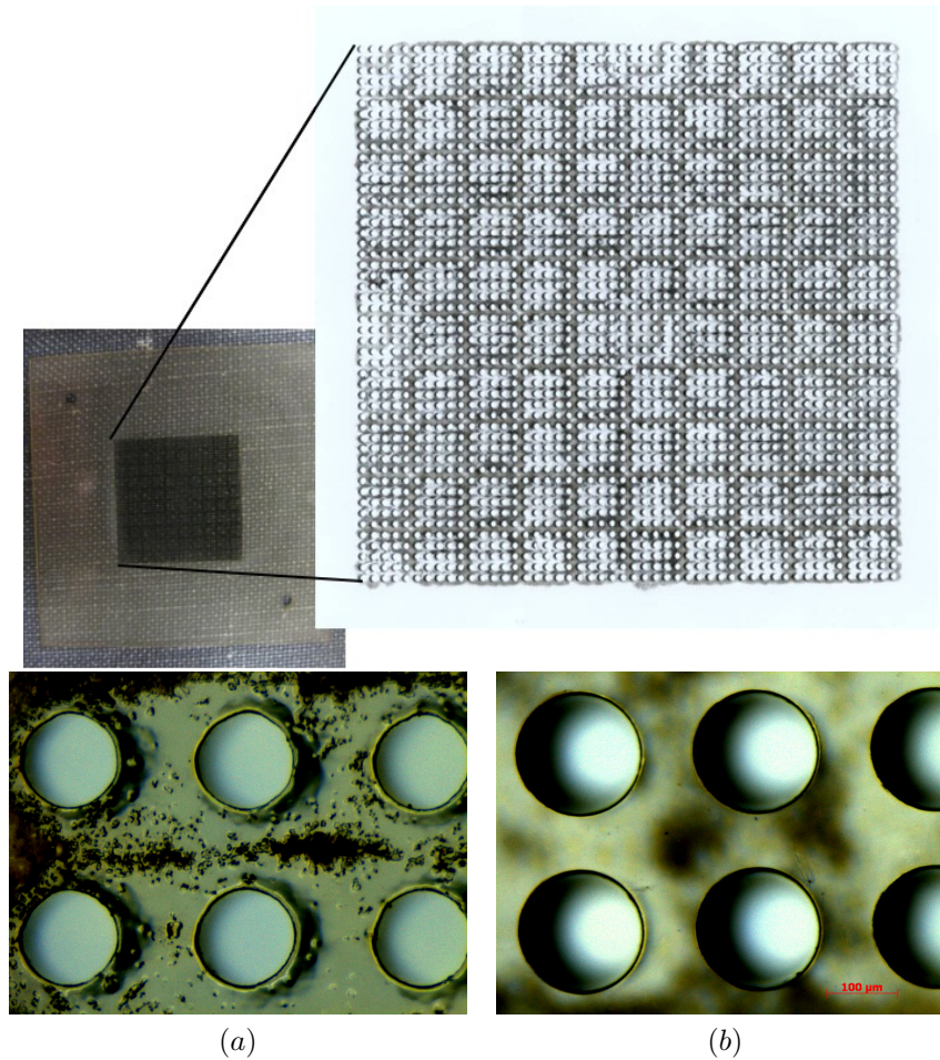
Figure 6.4: Images of the Cirlex array. The top panel shows a stitched view of the entire array with a \times 8 magnification. Bottom panels show alternate sides of the array with \times 100 magnification (design diameter is 142 \mu\text{m} ).
