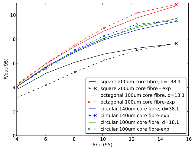
Figure 3.7: Comparison of theoretical modelled curves (solid lines) with experimental performed results (dashed lines) where the output focal ratio is displayed as a function of input focal ratio. The parameter d_0 which characterizes the affect of microbending is displayed for each theoretical curve.
