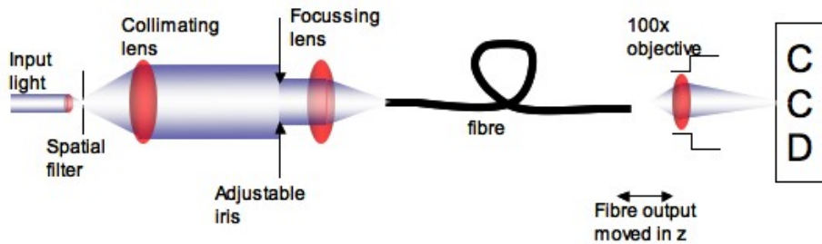
Figure 4.5: Experimental set-up to view the near to far-field transition of the output of the fibre
