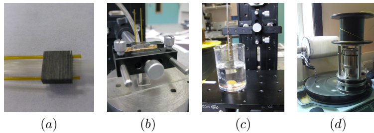
Figure 6.10: The process of building a fibre bundle. In (a) the wafers are stacked using the guiding pins and the fibres are inserted. In (b) the ends of the fibres are glued to ensure that they remain in place before being enclosed in the housing and (c) potted in epoxy which is allowed to wick up into the bundle. Finally the entire bundle is polished as shown in (d).
