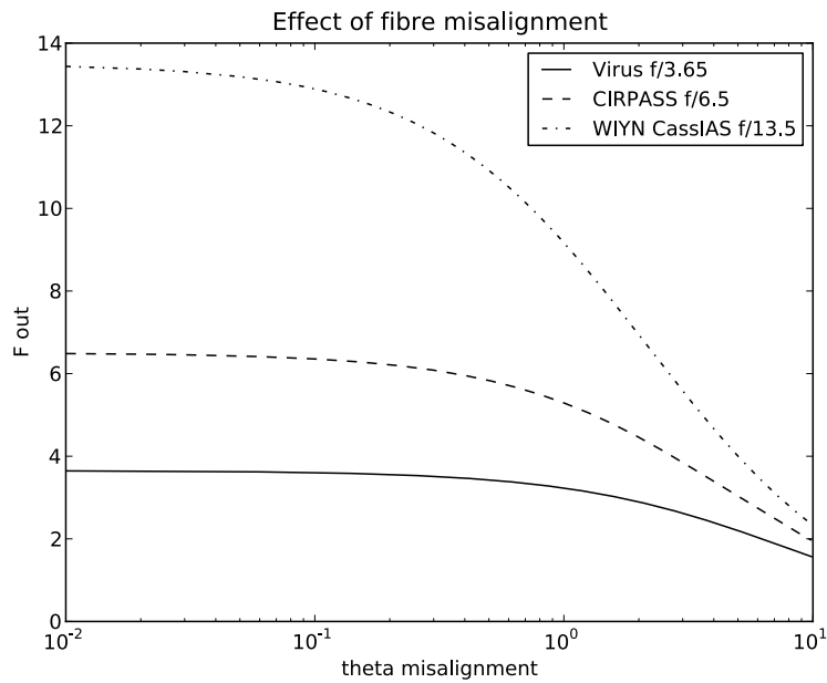
Figure 6.8: FRD that occurs due to varying amounts of fibre misalignment with respect to the optical axis for instruments that are fed at different focal ratios.
