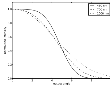
(b) FRD is worse at long wavelengths
