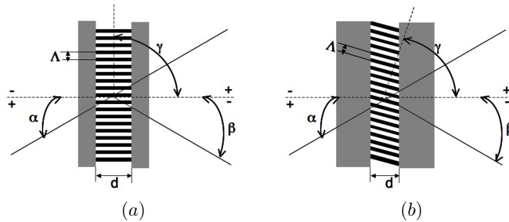
Figure 5.1: Some possible VPH grating configurations showing Bragg condition diffraction. (a) Transmission grating with fringes perpendicular ( \gamma = 90 degrees) to the grating surface (unslanted fringes). In this case the magnitude of \alpha equals that of \beta for the Bragg condition. (b) Transmission grating with tilted fringes may reduce ghost images [132].
