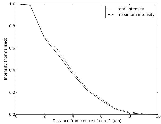
Figure 4.17: Graph to show how the amount of guided light decreases as the input spot is moved away from an arbitrary core. The dashed line shows the normalised peak intensity and the solid line shows the total number of counts. This clearly shows that light is being lost, into the cladding, or by reflection or scattering.
