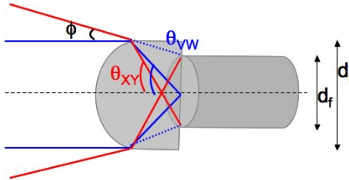
Figure 2.4: Geometric FRD induced by square lenslets.
