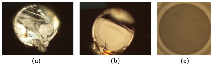
Figure 3.18: Results of different methods of end-preparation for a typical fibre with a diameter of 100 \mu\text{m} (a) unprepared (b) after cleaving (c) after polishing. In panel (b) the defect from scoring the fibre is clearly visible
