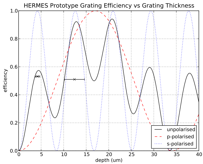
Figure 5.4: Theoretical efficiency of the prototype gratings with points to show the highest efficiency which was measured with the prototype gratings. The experimental results are presented in section 5.5.3.
