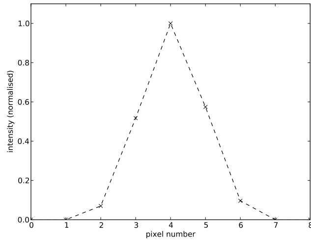
Figure 4.16: Plot through the centre of the image if a 5 \mu\text{m} spot is injected into a core. The spot shows a distinct maximum spot and no crosstalk is observed in any other part of the image
