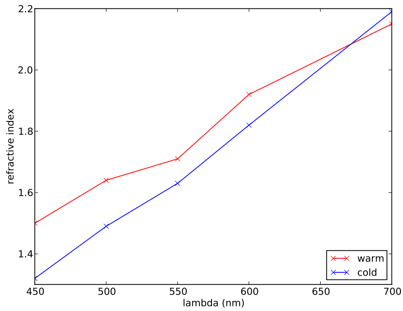
Figure 3.13: Variation of refractive index needed to maintain a constant d_0 for the FMOSa fibre
