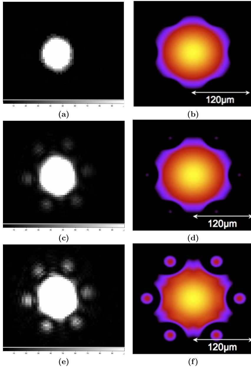
Figure 4.18: Experimental far-field intensity distribution as the CCD is translated away from the focal plane by (a) 1\mu\text{m} , (c) 5\mu\text{m} , (e) 9\mu\text{m} . Theoretical far-field intensity distribution as the CCD is translated away from the focal plane by (b) 1\mu\text{m} , (d) 5\mu\text{m} , (f) 9\mu\text{m} . a value of \gamma = 0.5 was empirically fit.
