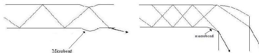
Figure 2.13: Microbending and macrobending are a major source of FRD
