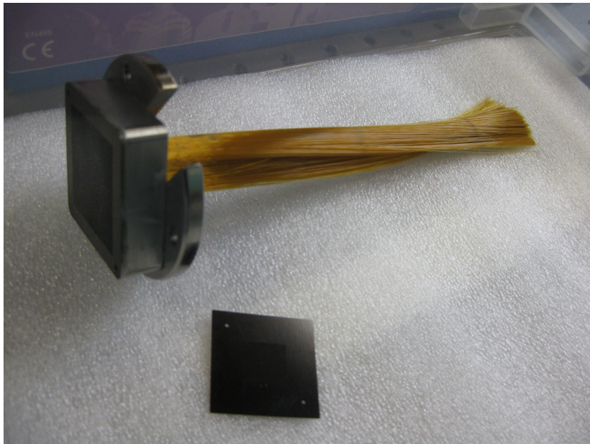
Figure 6.11: A 2304 bundle which has been built and polished. The bundle is built using fibres with a core size of 100 \mu\text{m} in diameter and a pitch of 200 \pm 5 \mu\text{m} .
