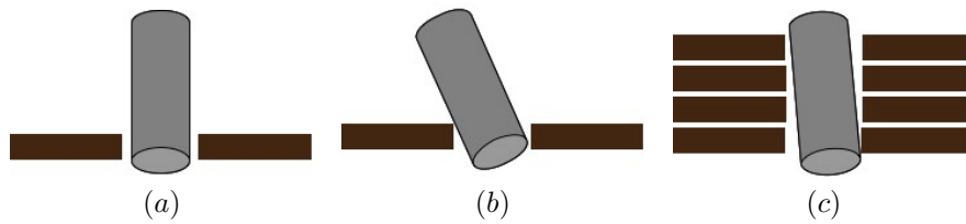
Figure 6.7: If the fibre is only constrained by a guide which is a few mm thick, the fibres may not be parallel to the optical axis. Panel (a) shows the ideal case, panel (b) shows the extreme case of a thin stack and panel (c) shows how a thicker array can constrain the angle of the fibre with respect to the optical axis.
