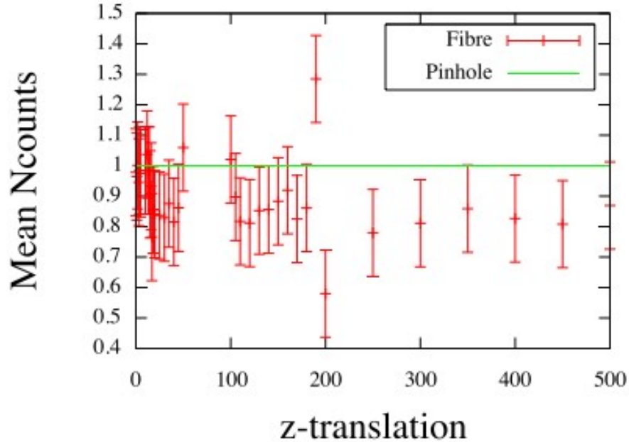
Figure 4.6: 89\% \pm 2\% of the incident light was guided by the fibre. Since \sim 4\% will be lost at each air-glass interface, this shows that only \sim 3\% of the incident light was lost within the fibre.
