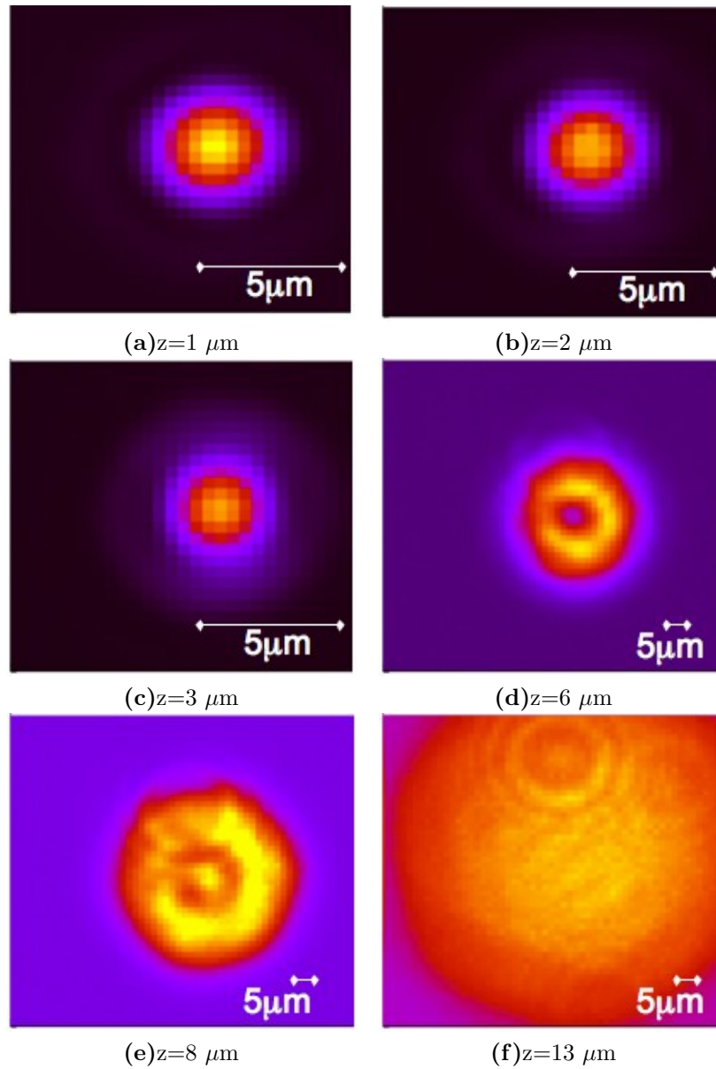
Figure 4.7: Experimental intensity distribution as the fibre is translated away from the focal plane. (a) to (b) In the extreme near-field the mode is circular with a Gaussian profile, (c) an airy disk develops as the diffraction limit is approached, (d) and (e) air holes modify the overall Gaussian distribution sufficiently to produce higher order spots, (f) the distribution returns to a smooth, circular Gaussian in the far-field.
