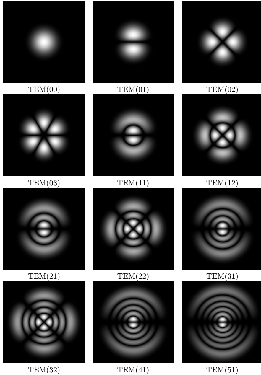
Figure 2.7: Electric field amplitude profiles for the cylindrical Transverse Mode Patterns TEM(pl). In general, light launched into a multimode fibre will excite a superposition of different modes.
