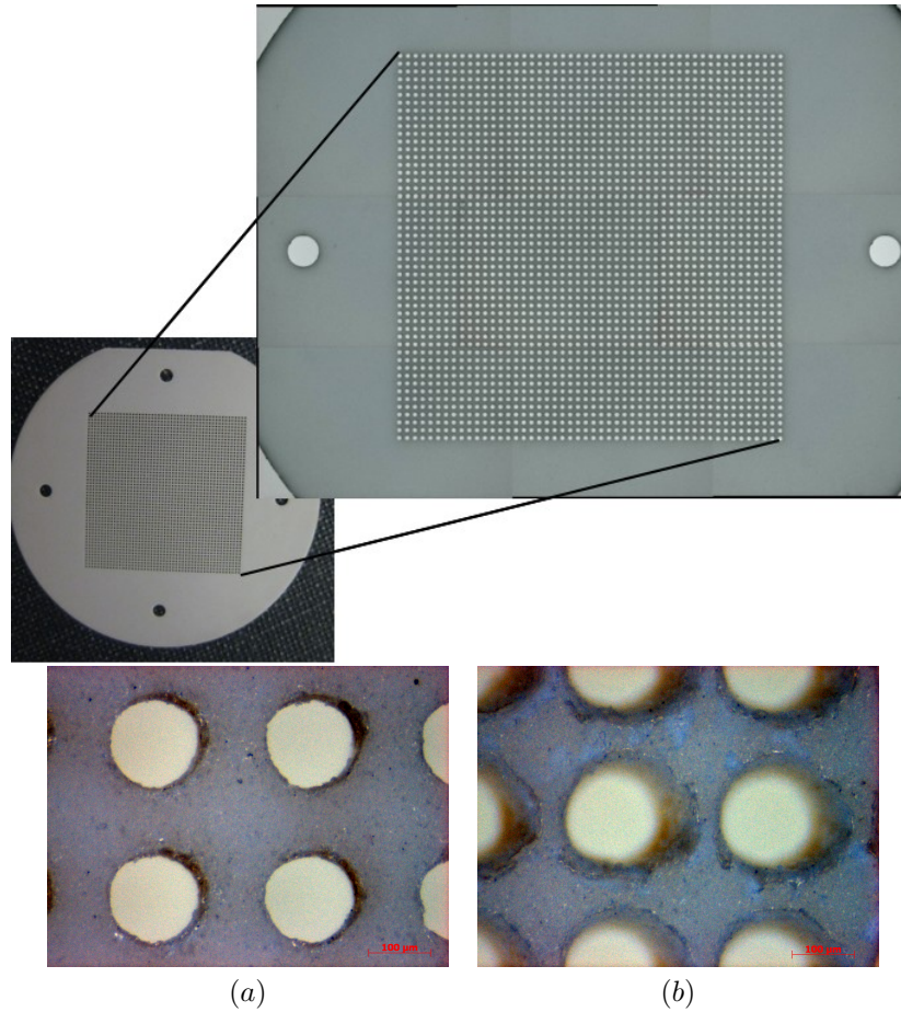
Figure 6.6: Images of the Ceramic array. The top panel shows a stitched view of the entire array with a \times 8 magnification. Bottom panels show alternate sides of the array with \times 100 magnification (design diameter is 142 \mu\text{m} ).
