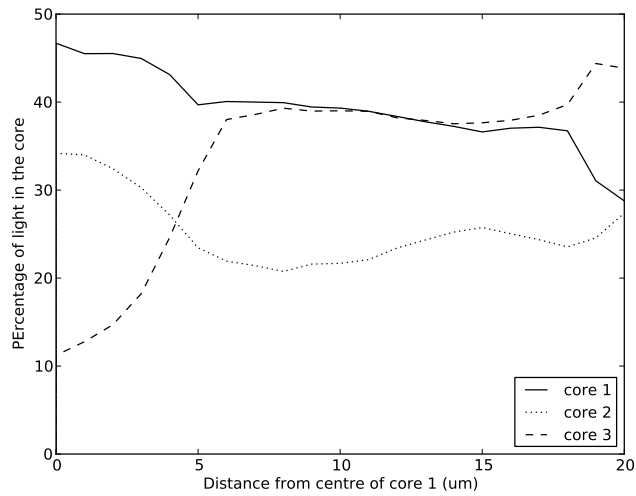
Figure 4.15: If a spot larger than the mode field diameter is injected into a single core, crosstalk is observed in neighbouring cores. As the input spot is moved, the percentage of light in the 'main' core decreases as the spot is translated away from its centre.
