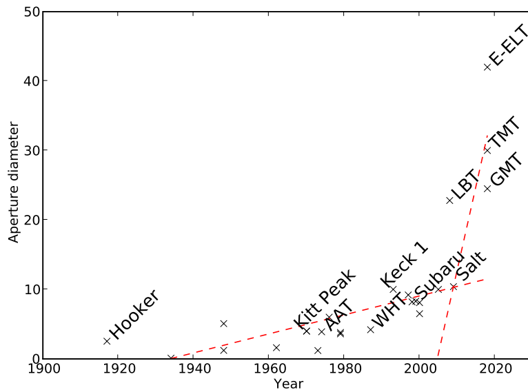
Figure 1.3: The diameter of the aperture of telescopes has increased substantially over the last 100 years. Linear fits show the increased rate at which telescope size is predicted to develop over the next 10 years.
