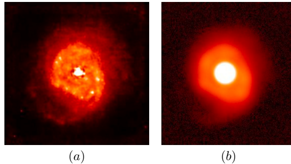
Figure 1.5: Image of NGC7469 (a starburst galaxy) taken on PUEO at the CFHT with (a) Adaptive Optics module turned on and (b) no Adaptive Optics. The field of view is 10 \times 10'' , with a resolution of \sim 0.13'' , courtesy of CFHT.
