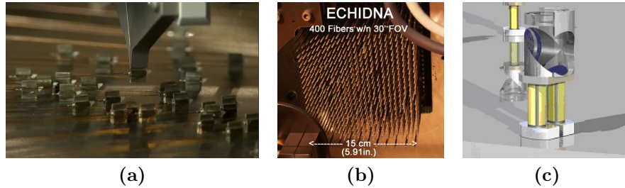
Figure 2.2: 2dF, ECHIDNA, and starbugs show the evolution of fibre positioning systems for Multi-Object Spectroscopy.
