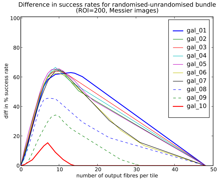
Figure 6.21: The improvements that can be made by randomising prior to down selection for the Messier objects
