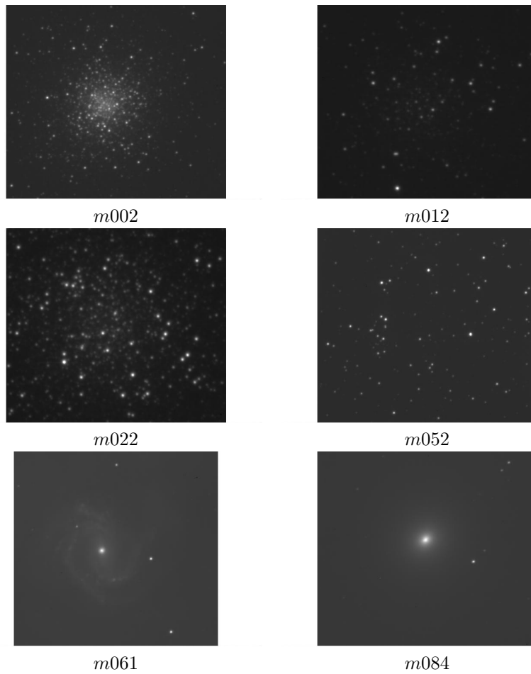
Figure 6.19: The first 6 Messier objects with various amounts of clustering, used to test different remapping schemes.
