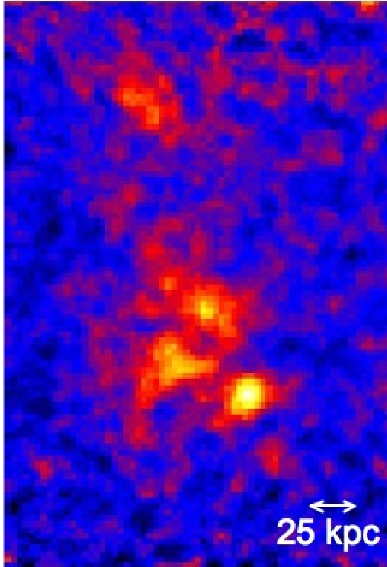
Figure 2.5: Continuum-subtracted \text{Ly}\alpha emission region LAB1 in the SSA 22 protocluster region at z = 3.09 [43]. This image was obtained by collapsing the SAURON spectra over a narrow wavelength range centred on the emission line. These objects are not easily observed since the earth's atmosphere is very effective at filtering out UV photons so \text{Ly}\alpha photons must be highly red-shifted in order to be transmitted through the atmosphere. It is expected that this is the kind of faint object which will be readily accessible to ELTs (Image courtesy of Weijmans 2009)
