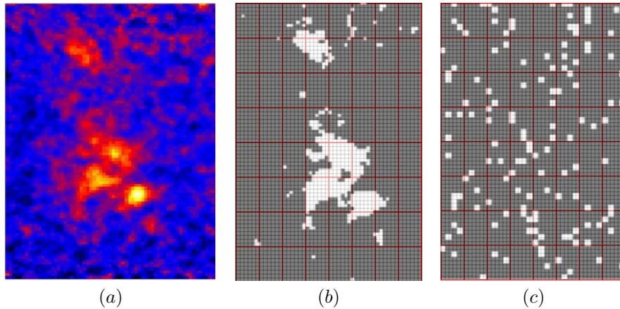
Figure 6.18: Process to calculate the success rate of random mapping strategies. In (b) the image is binned into 48 \times 48 spaxels arranged into N_C = 48 cells each of N = 6 \times 8 = 48 spaxels, of which M may be routed to the output. Spaxels are defined to contain unit value if the intensity exceeded a specified threshold or zero otherwise in order to identify the 200 brightest spaxels. Due to the switch architecture, down-selection is limited within tiles, so if there are no ROIs within a cell, the switches cannot be reallocated to another cell. Hence, the field is randomised, as shown in panel (c) so as to redistribute the ROIs over the entire field.
