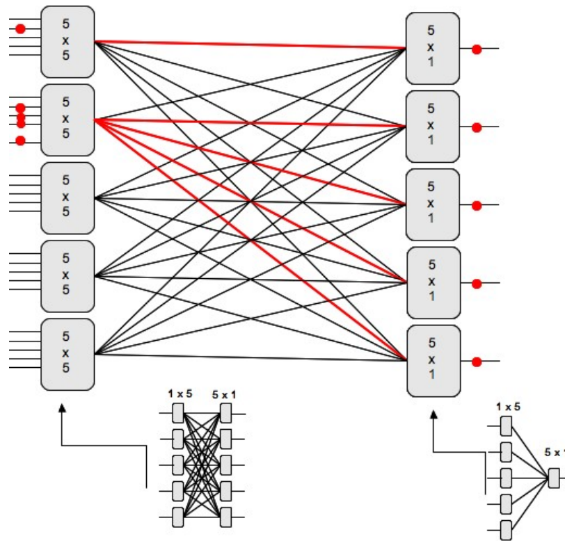
Figure 6.12: 2 layer switching used to create a N \times M switch where N is the number of inputs, M is the number of outputs, and M = \sqrt{N} .
