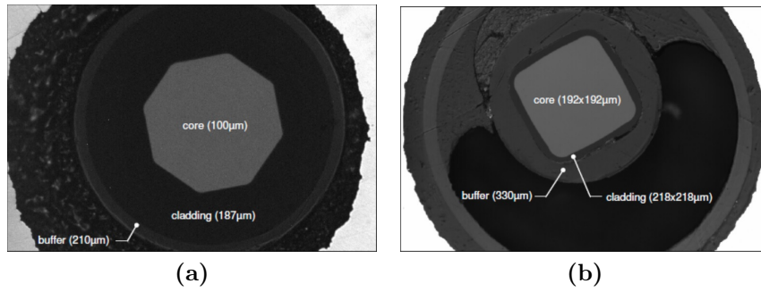
Figure 3.6: Image of the octagonal and square fibres after they had been hand polished to 3 \mu\text{m} .
