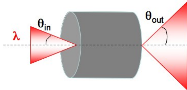
Figure 2.10: Focal Ratio Degradation occurs when \theta_{in} \lesssim \theta_{out} .
