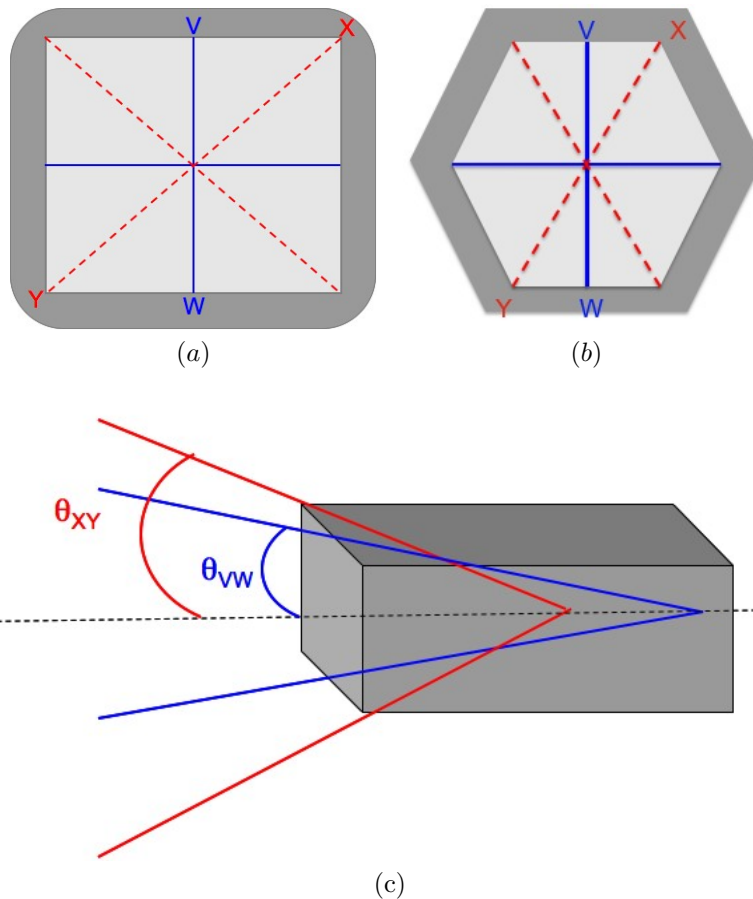
Figure 3.8: Geometric FRD of non-circular core fibres. As shown in (a) and (b) for square and hexagonal core fibres respectively, light entering from the VW axis will have a smaller angle than light entering from the XY axis.
