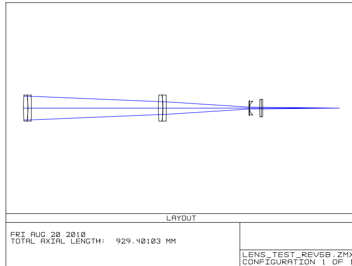
Figure 5.16: Layout of the 4 lens telescope system
