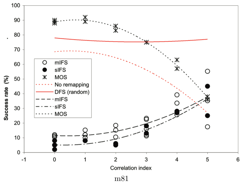
Figure 6.25: Plot of success rate (i.e. occupancy) against correlation index for different types of remapping and without remapping (control). Data points for different realizations are shown together with trend lines (dashed curves).
