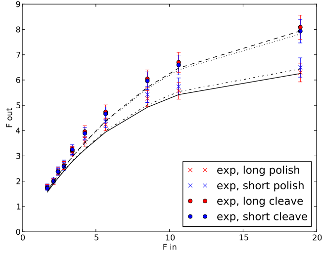
Figure 3.19: FRD curves where experimental results are shown by crosses and theoretical results produced by the original one-fibre model are given by a smooth line
