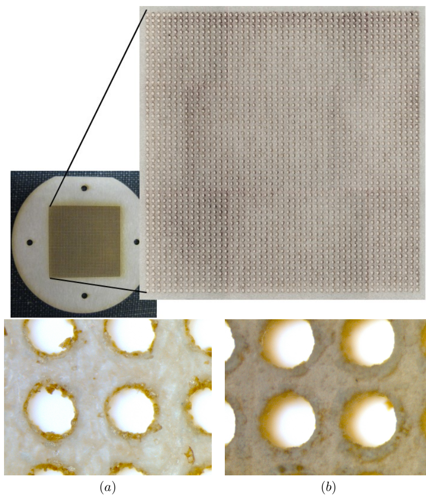
Figure 6.5: Images of the Paper array. The top panel shows a stitched view of the entire array with a \times 8 magnification. Bottom panels show alternate sides of the array with \times 100 magnification (design diameter is 142 \mu\text{m} ).
