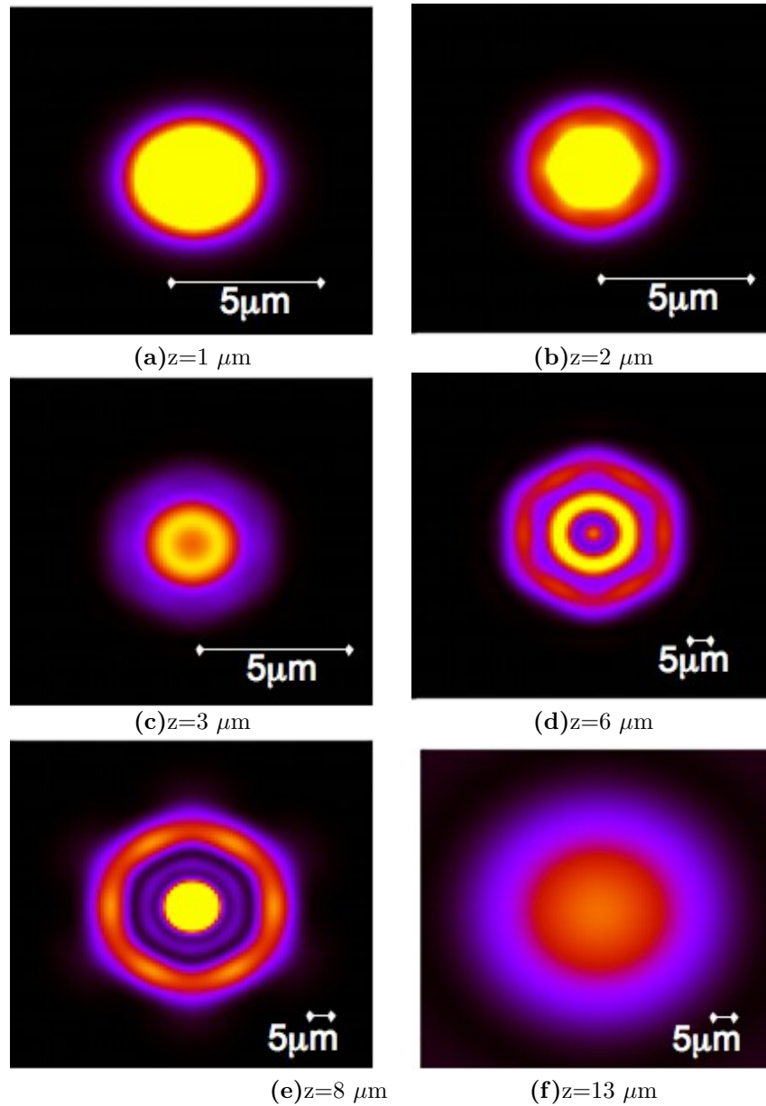
Figure 4.8: Theoretical intensity distribution as the fibre is translated away from the focal plane. In the extreme near-field the mode is circular with a Gaussian profile, an airy disk develops as the diffraction limit is approached, the mode transforms to hexagonal intensity distribution, air holes modify the overall Gaussian distribution sufficiently to produce higher order spots, and finally the distribution returns to a smooth, circular Gaussian in the far-field.
