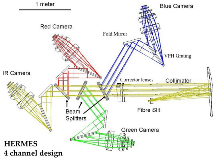
Figure 5.3: Optical configuration of the HERMES instrument ( image courtesy of Luke Gers )
