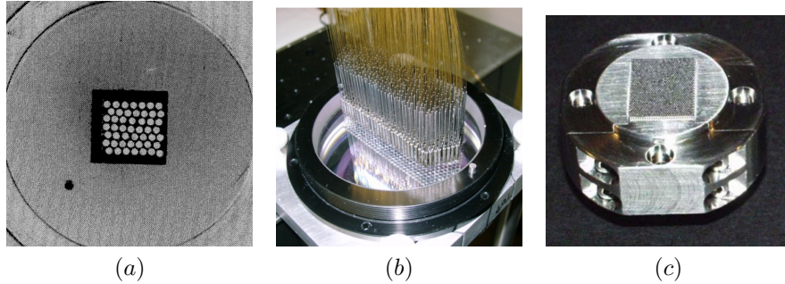
Figure 6.2: The development of building fibre bundles has progressed from a simple fibre design (a - DensePak) to a larger bundle which includes microlenses (b - CIRPASS) to a massive bundle of 1000 fibres (c - GMOS).
