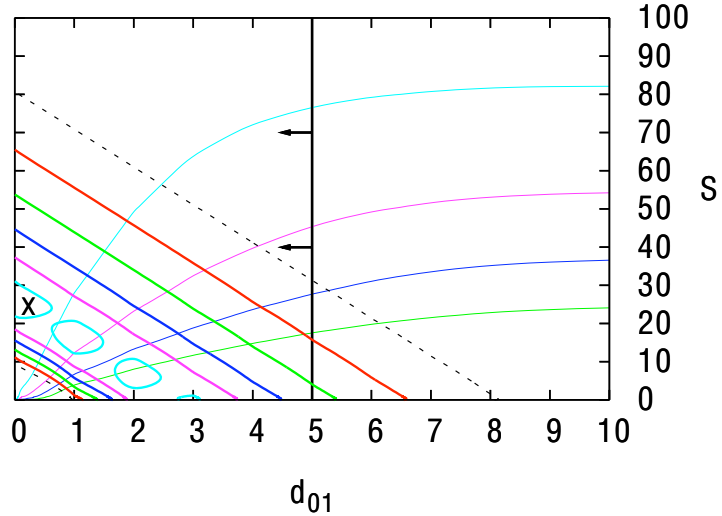
Figure 3.23: The two fibre model was run for various combinations of d_{0,1} and S (where S = d_{0,2}L_2 ). Panel (c) shows how these graphs can be combined to find a single solution, marked by the large cross, for d_{0,1} and S which satisfies experimental data. The black vertical line in panel (c) shows the d_{0,1} parameter predicted by the one fibre model for the cleaved fibre.
