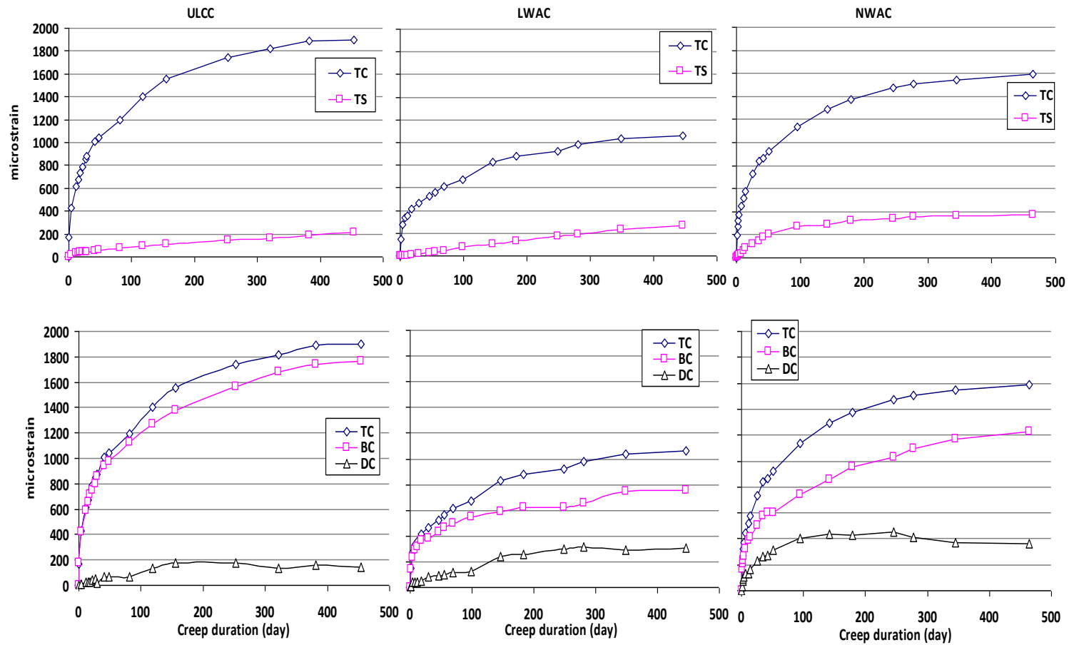
Fig. 3: Development of creep and shrinkage strains, (TC – total creep, TS – total shrinkage, BC – basic creep, DC – drying creep)
