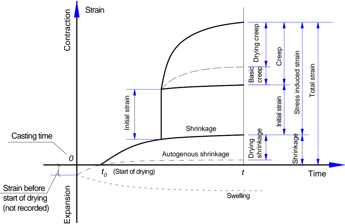
Fig. 1: Relationship between various measured and derived strains – concrete undergoes autogenous shrinkage (before drying) and drying shrinkage. Upon loading, drying creep and basic creep (creep without drying effect) occurs (ACI 209, 2005)
