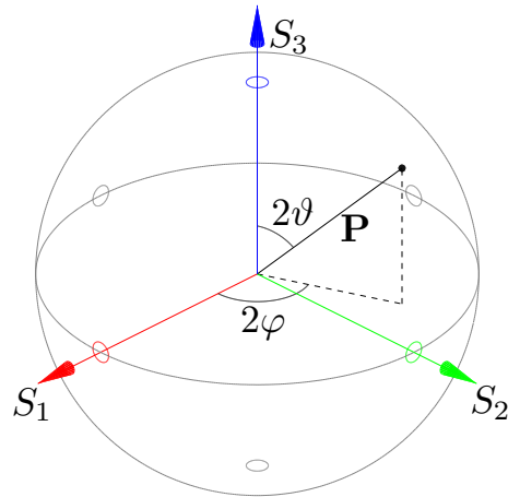
Figure I.1: Illustration of the Poincaré sphere
