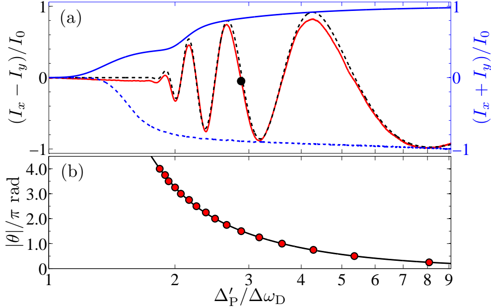
Figure 9.4: (a) Probe signal produced by scanning the probe versus red detuning, \Delta'_P , from the D_1 ^{87}\text{Rb} F_g = 2 \rightarrow F_e = 1 transition in units of Doppler width \Delta\omega_D = 2\pi(571 \text{ MHz}) . On the left axis, the red and dashed black curves show, respectively, the measured and theoretical differencing signal. On the right axis, the solid blue curve shows the theoretical total transmission through the cell in the presence of the magnetic field, whilst the dashed blue curve shows the measured total transmission in the absence of the magnetic field (flipped vertically for clarity). (b) The measured rotation angle (data points) and theoretical rotation (curve). The temperature of the cell is 115^\circ\text{C} and the applied magnetic field is 204 G.
