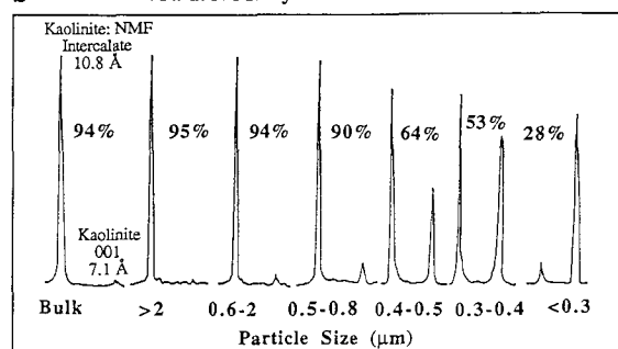
Figure 4. Two examples of XRD profiles obtained on kaolinite : NMF intercalates for: a) Weipa and b) Georgia KGa-1 samples. The relative intensities of the intercalate peak and the kaolinite (001) peak indicate the percentage yield of intercalated product for each bulk and size-separated sample.
