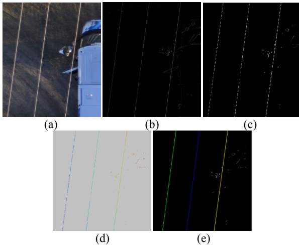
Figure 3. Linear feature detection result. (a) original image; (b) ridge points; (c)-(d) connected components and their colour representation; (e) detected power lines
