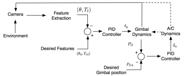
Figure 5. High level control architecture for the active guidance. Sub-index d denotes desired values and \delta are the commanded values.
