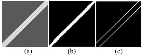
Figure 6. Illustration of ridge-based and edge-based line detection on a synthetic image
