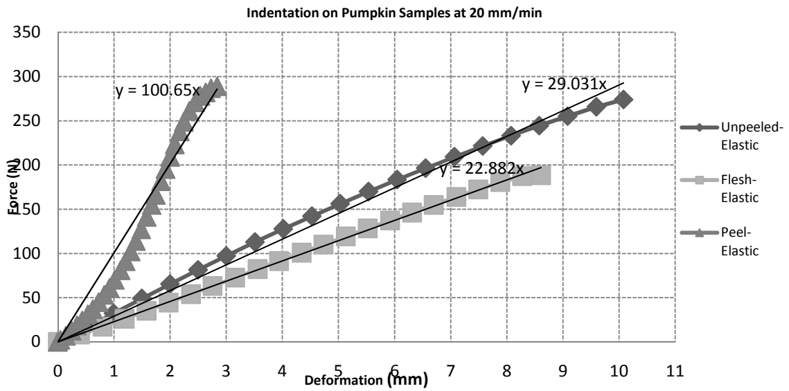
FIGURE 4 : Force deformation curve of skin, flesh and unpeeled samples in compressive loading.
