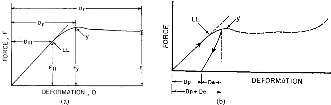
FIGURE 2 : (a) Force deformation curve for agricultural products – (b) Degree of elasticity from the loading-unloading curve. D_e = elastic or recoverable deformation; D_p =plastic or residual deformation; D_e/(D_p+D_e) . [9].
