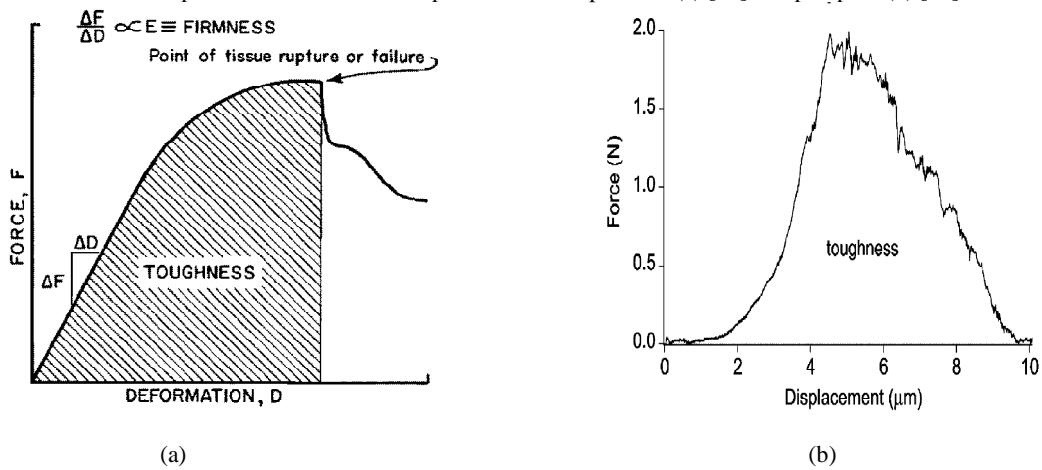
FIGURE 8. : (a) Firmness and toughness from force deformation details of food particles under compressive loading [16], (b) Toughness of a raisin sample using force deformation curve[19].
