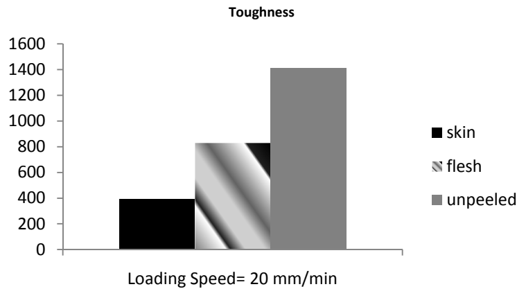
FIGURE 9: Toughness of flesh and unpeeled samples in 20 mm/min loading rate.
