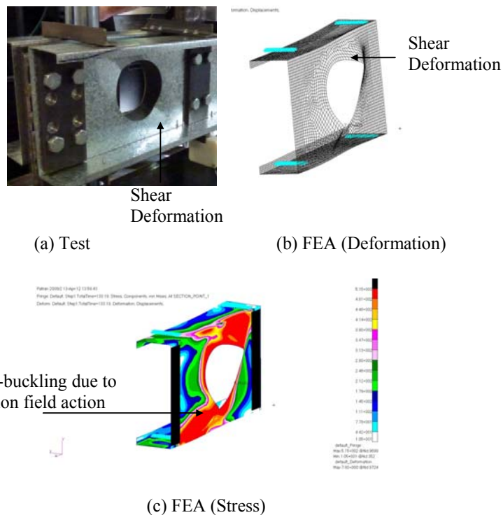
Figure 6: Failure Mode of 200x75x15x1.9 LCB with 125 mm Web Openings (Aspect Ratio = 1.5)
