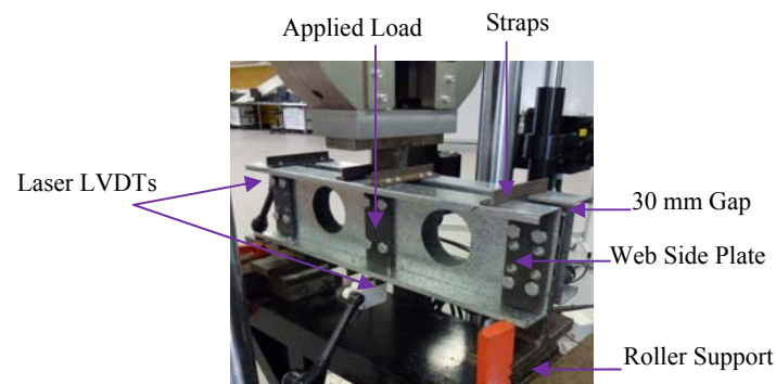
Figure 2: Experimental set-up
