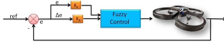
Fig. 2. Schematic diagram of the control Loop.
