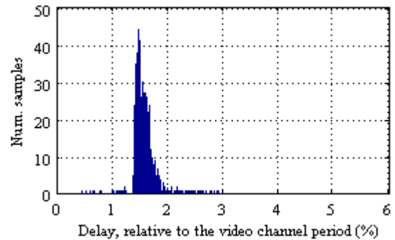
Fig. 4. Distribution of the delays introduced in the video channel by the framework. The relative delays are percentages of the average video channel period, i.e. 66.67 ms. The highest sample is 2.9%, but the horizontal scale is set as in Fig. 3 for easy comparison.
