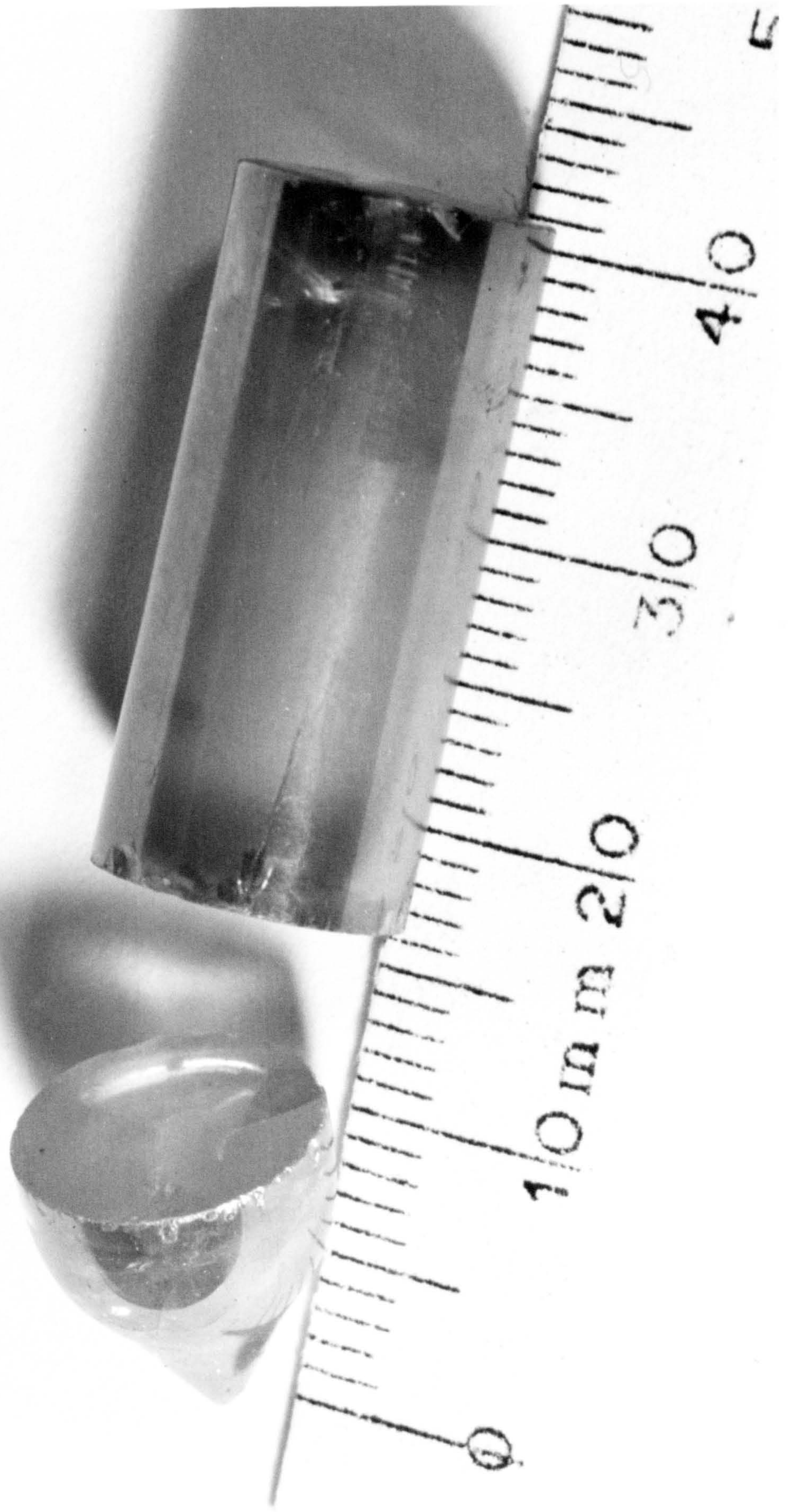
FIGURE 3.5 A CdS(Te) boule grown with Clark-Woods technique (37)
