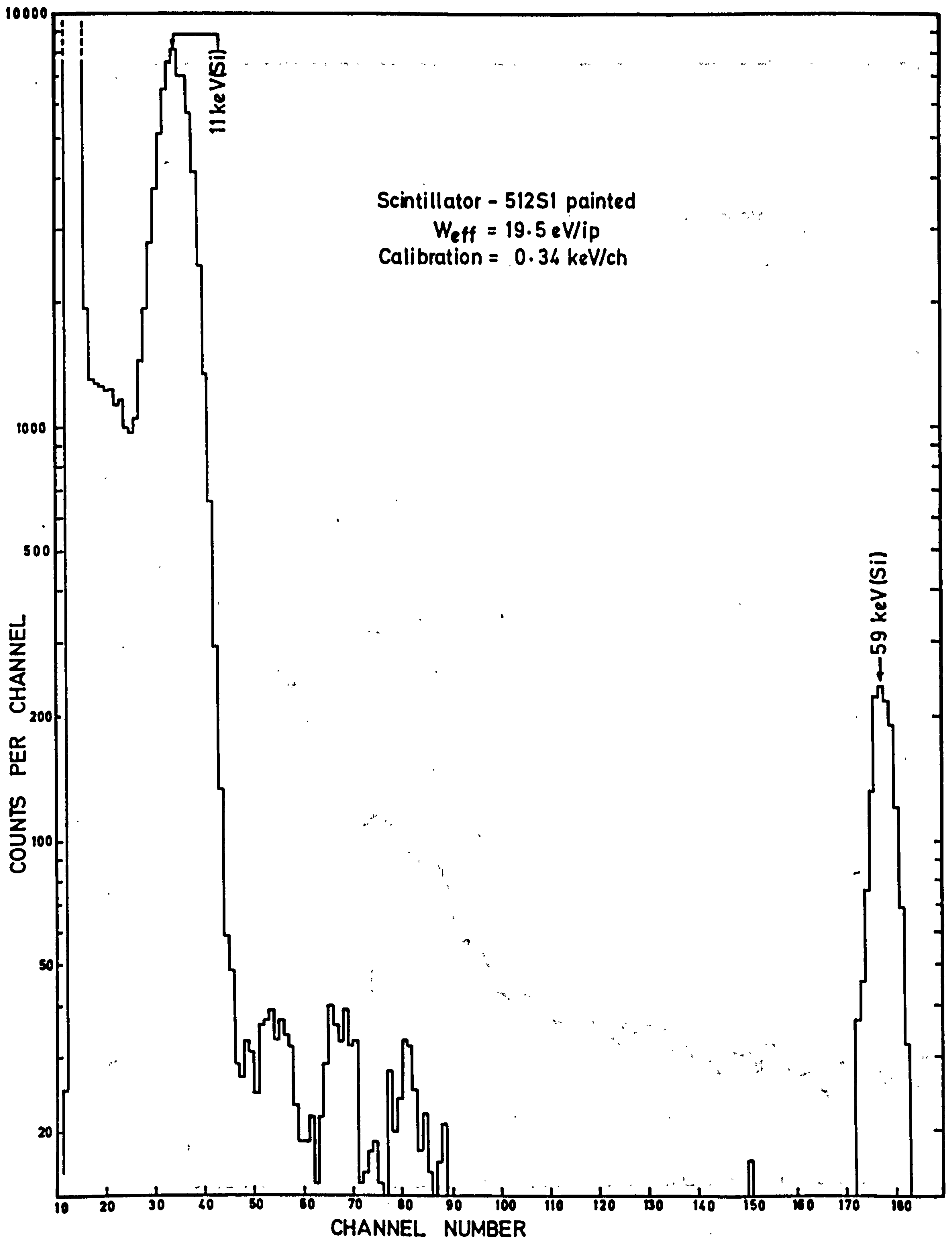
Figure 6.5 ^{241}\text{Am} gamma-ray spectrum taken with the \text{CdS}(\text{Te}) -photodiode detector cooled at 110 K (source is well collimated on the crystal)
