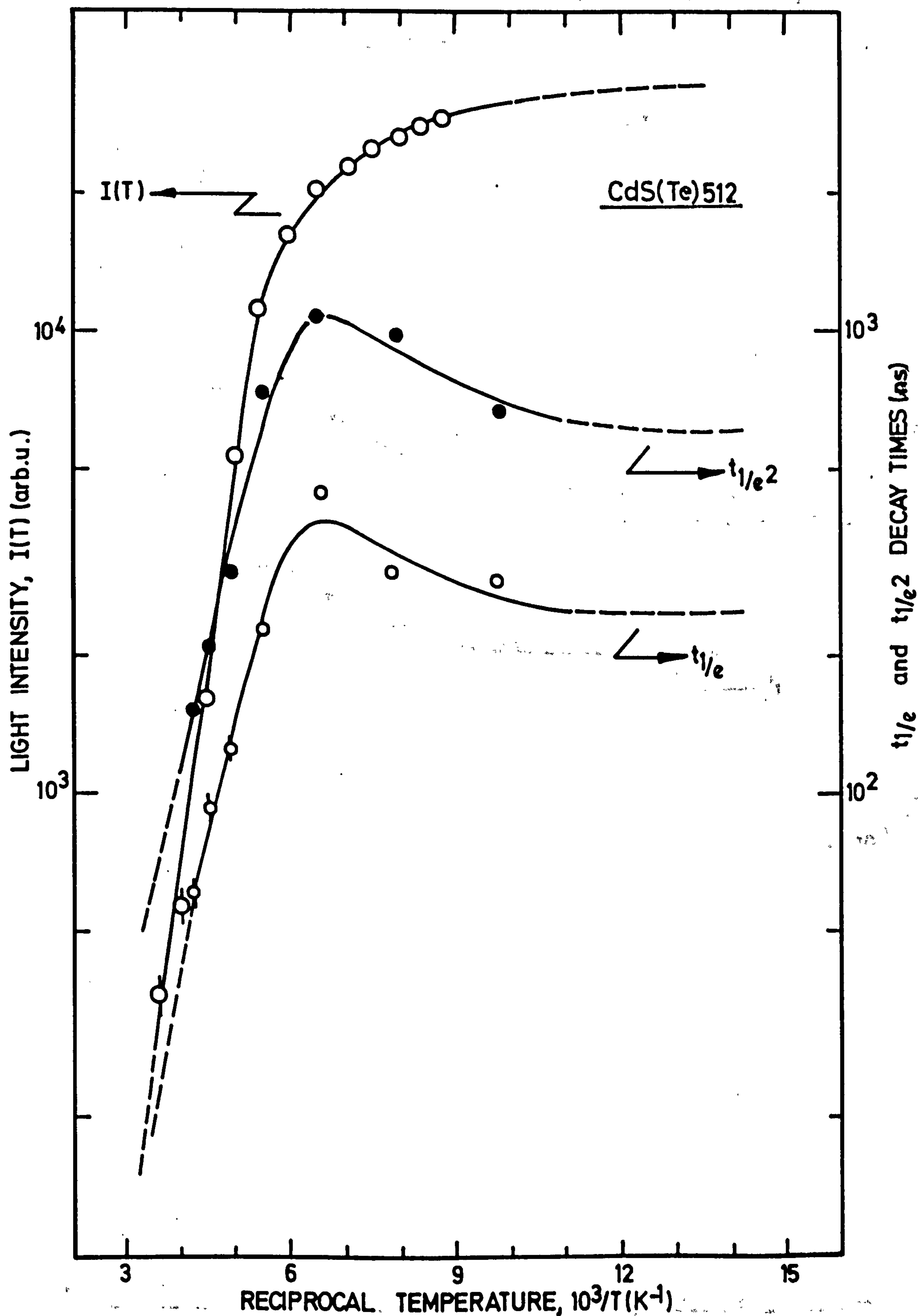
FIGURE 5J2 Variation of the intensity and decay times of the beta-induced luminescence with temperature in CdS (Te) 512S1.
