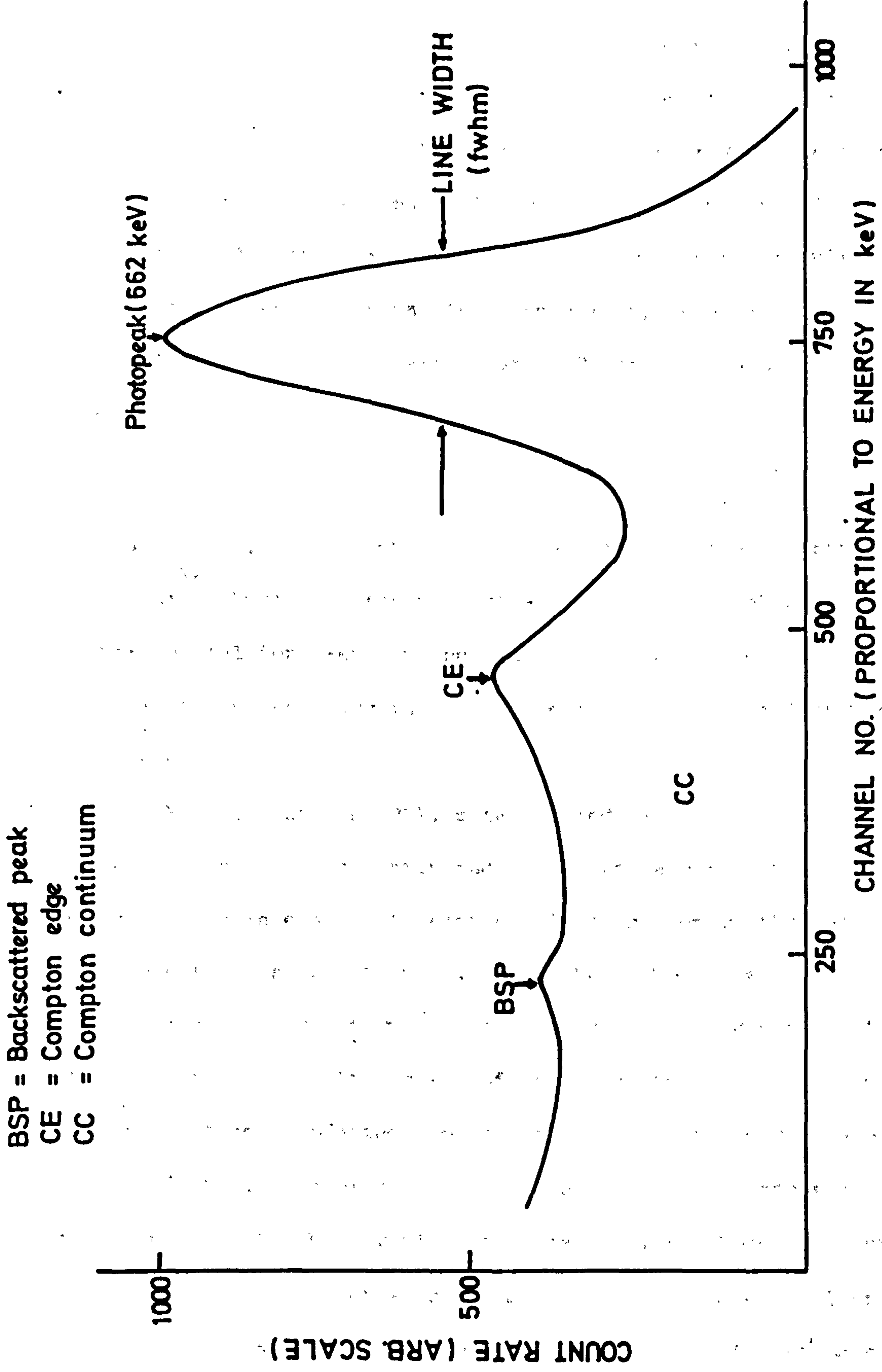
FIGURE 1.2 A gamma radiation spectrum ( 137 Cs).
