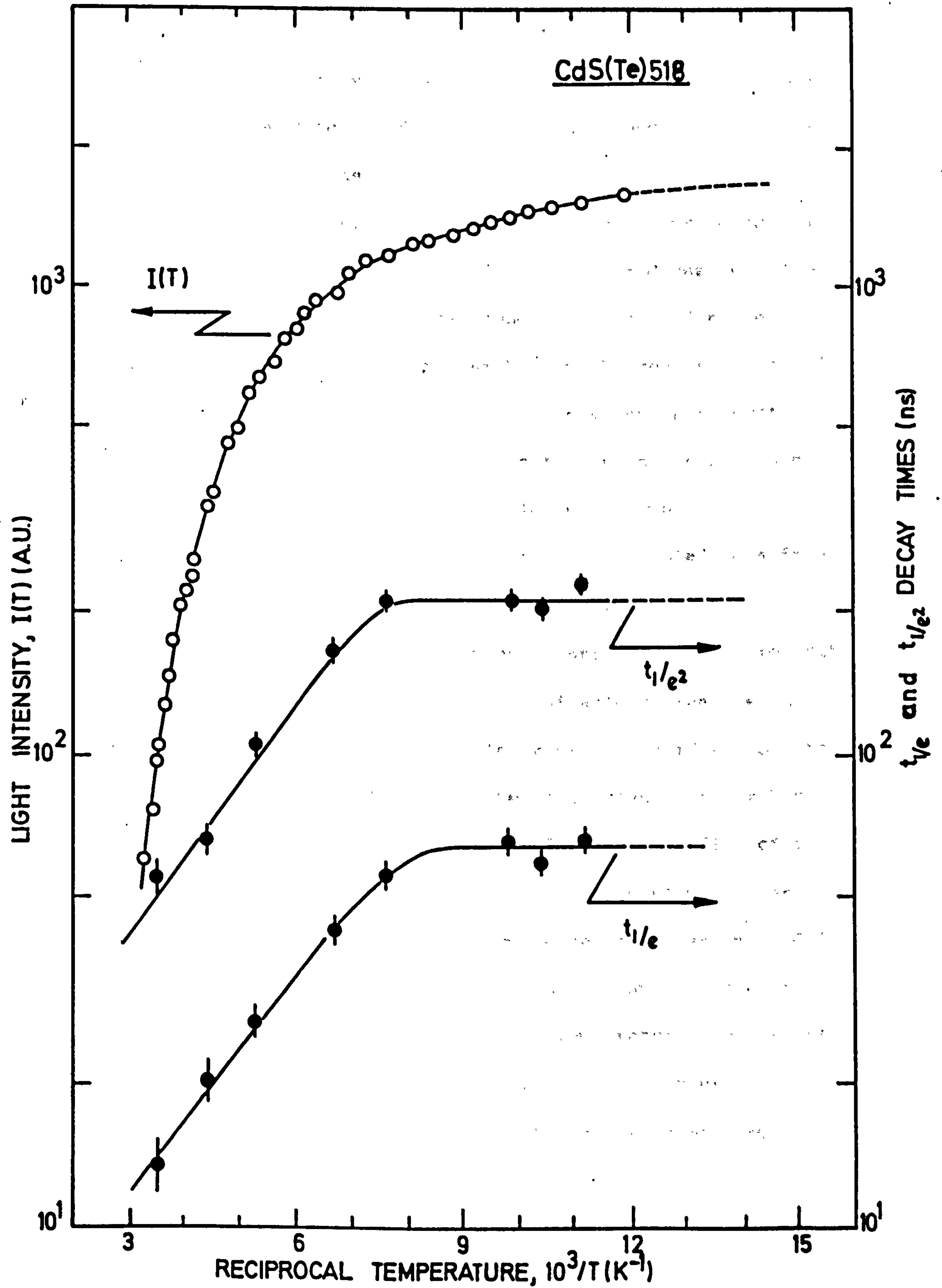
FIGURE 5.8 Variations of intensity and decay times of alpha-induced luminescence with temperature in CdS(Te) 518S1.
