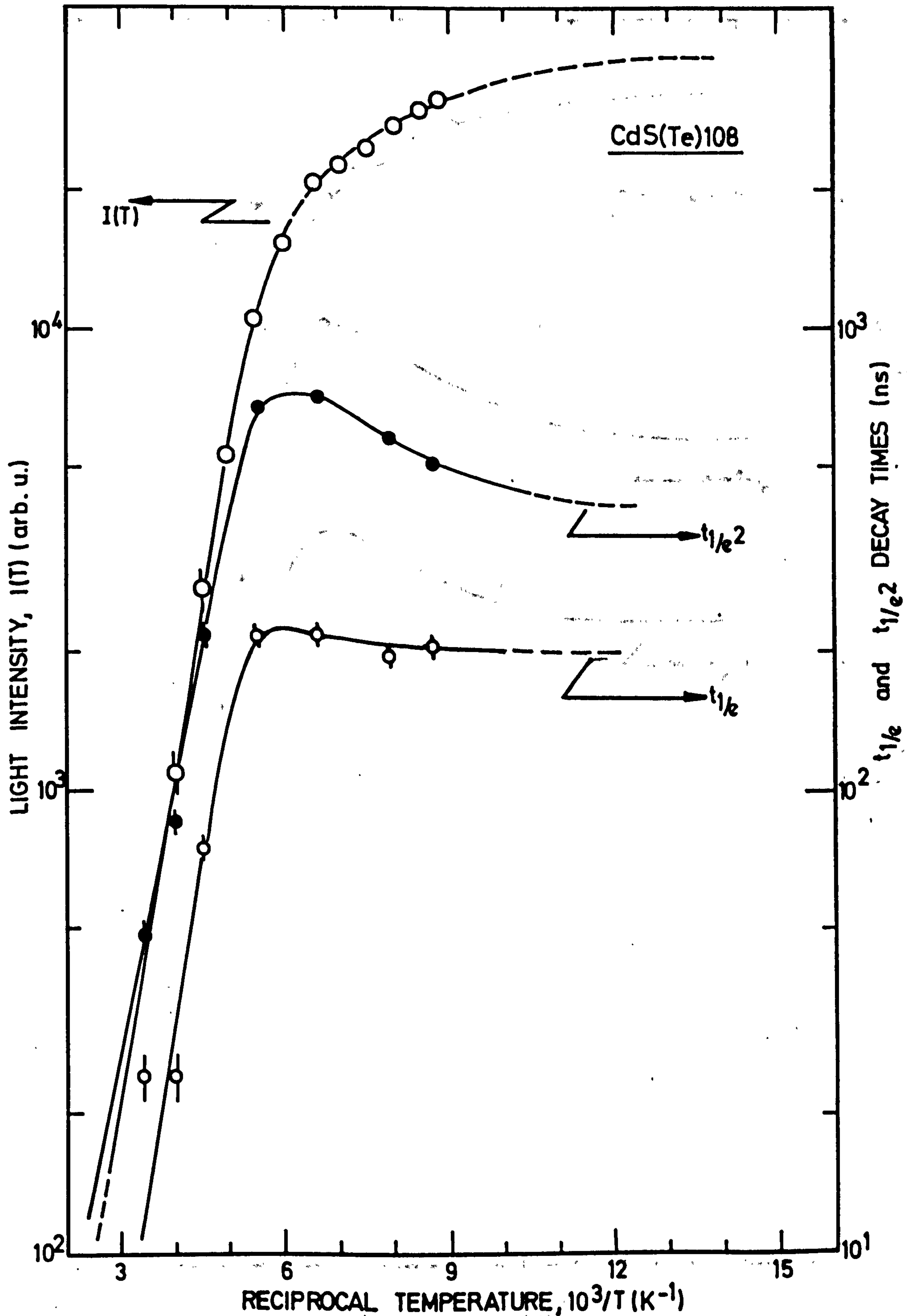
FIGURE 5.11 Variation of intensity and decay times of the beta-induced luminescence in CdS(Te)108S10.
