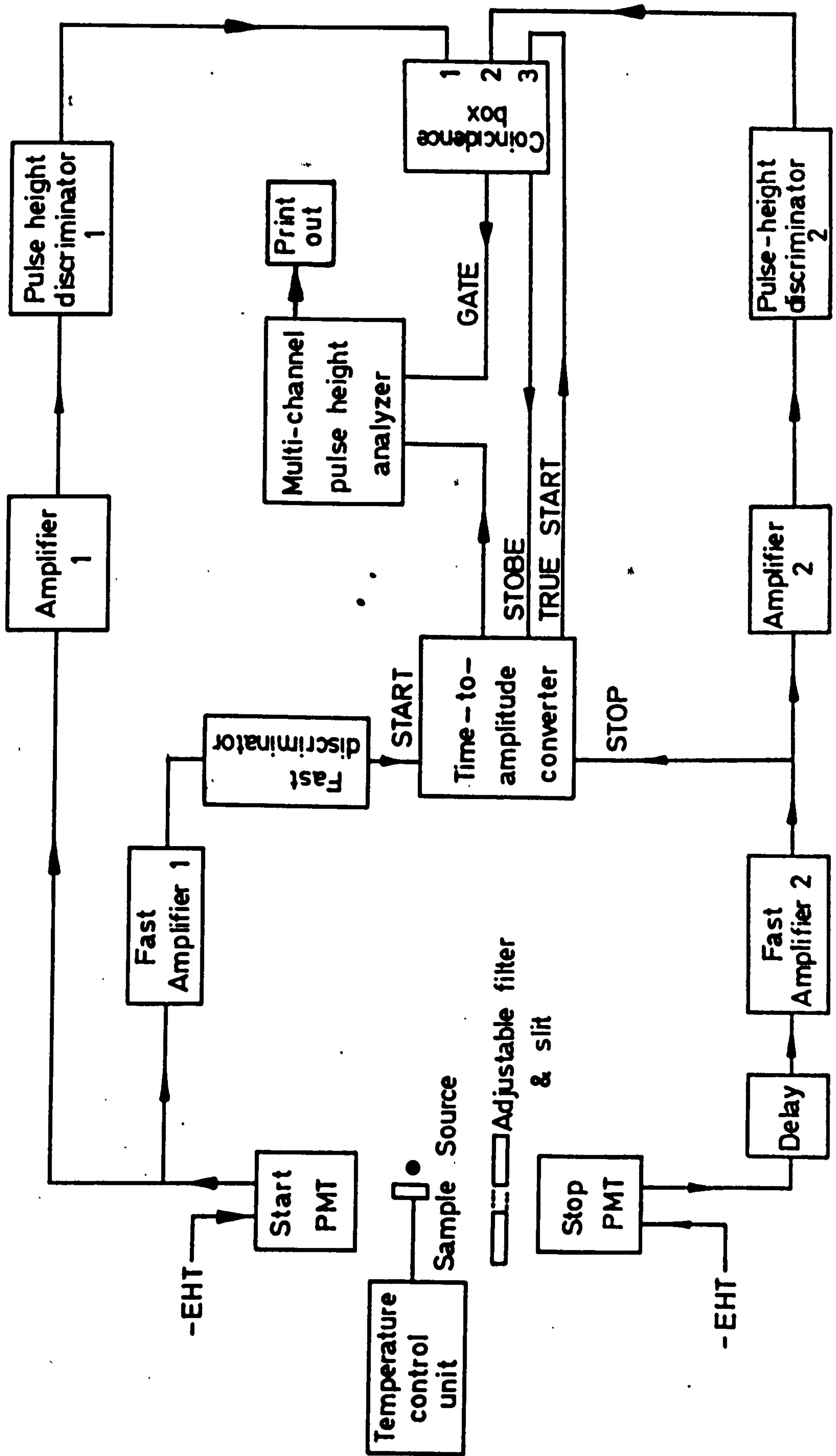
FIGURE 4.1 Schematic diagram of the experimental arrangement used for the measurement of scintillation decay time.
