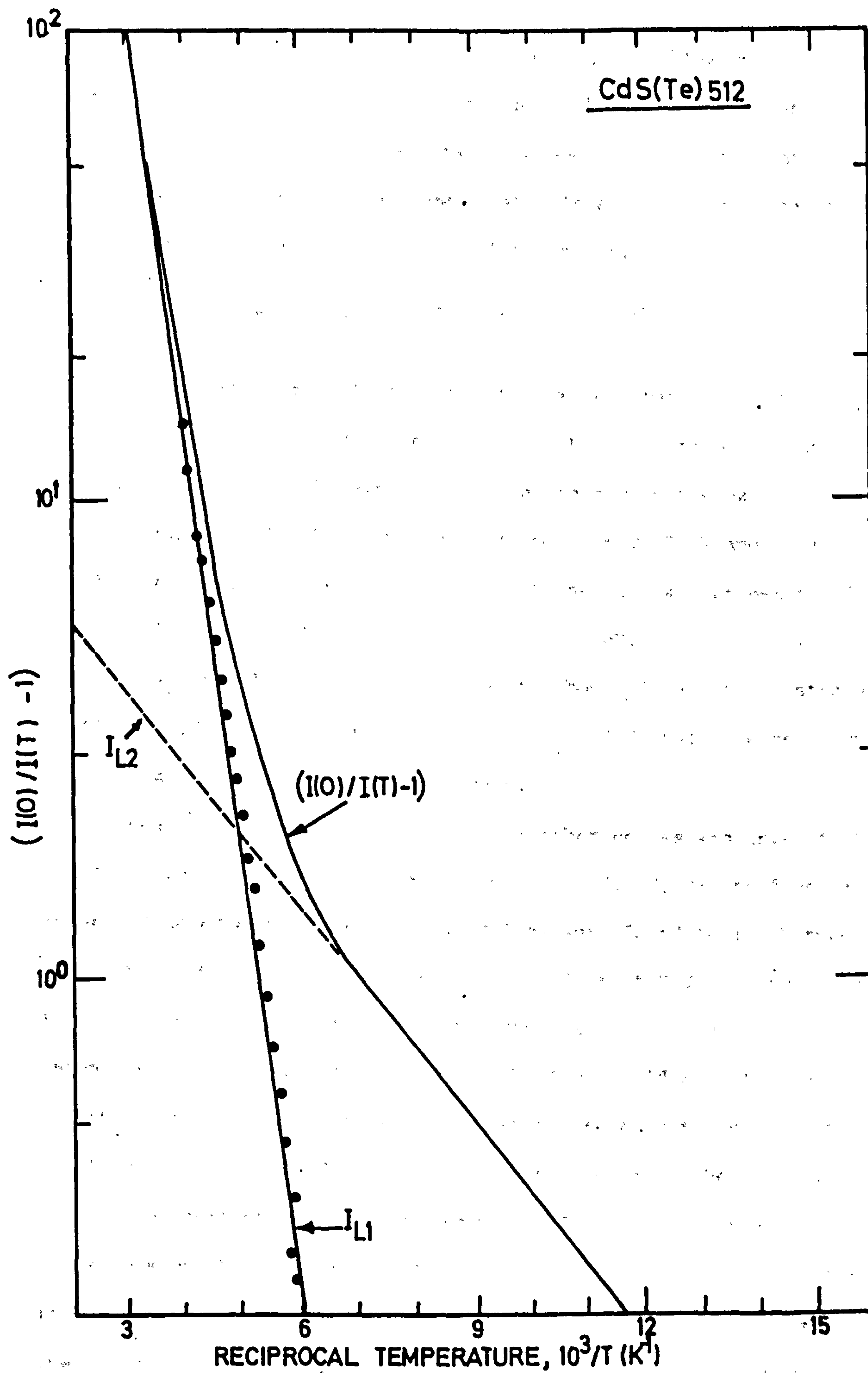
FIGURE 5.9 Graphical analysis of the thermal quenching curve I(T) of CdS(Te) 512S1.
