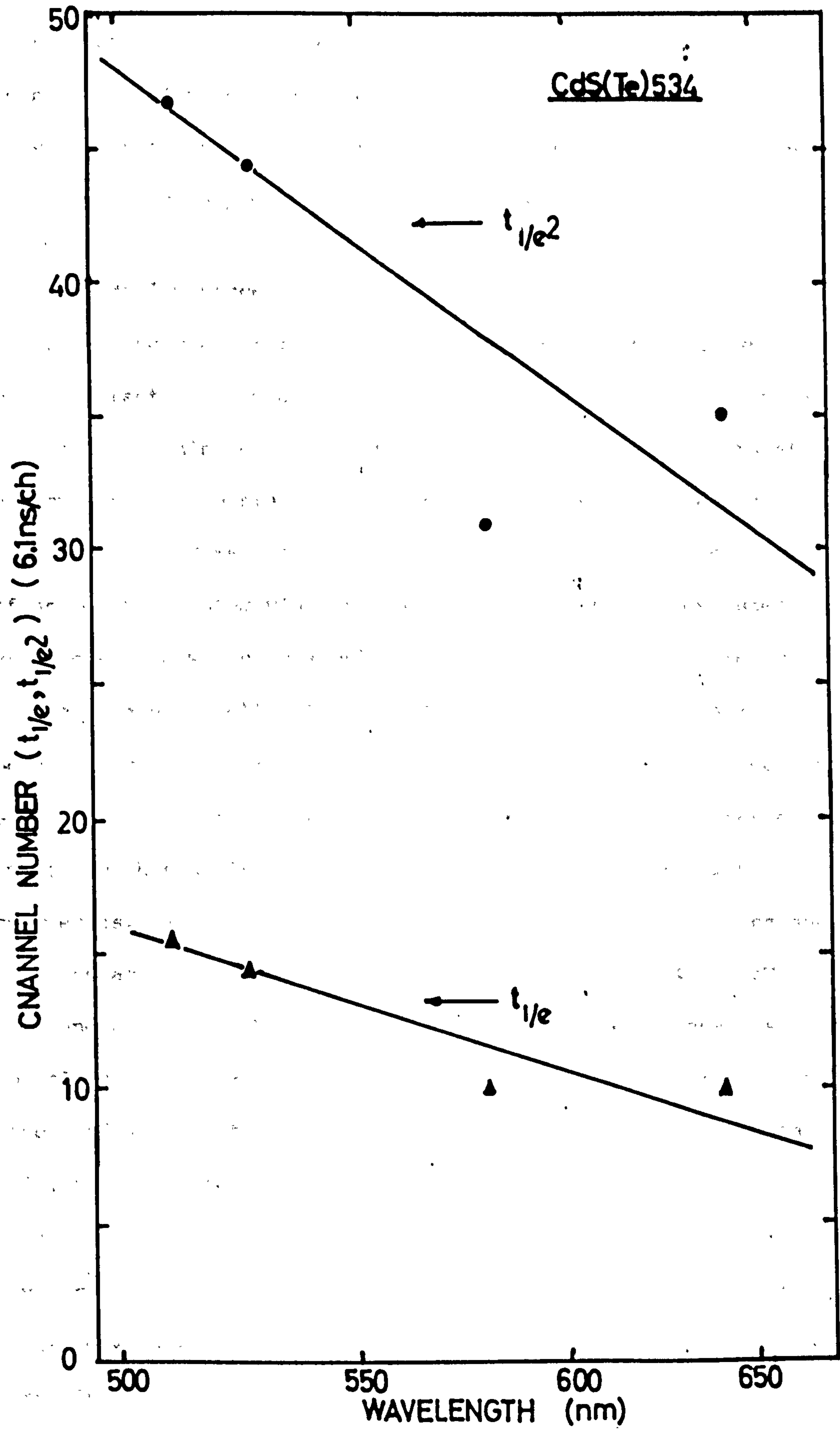
FIGURE 7.14 Decay time variations with the wavelength of emission when boule 534 is stimulated by \alpha -particles at 95K (69)...
