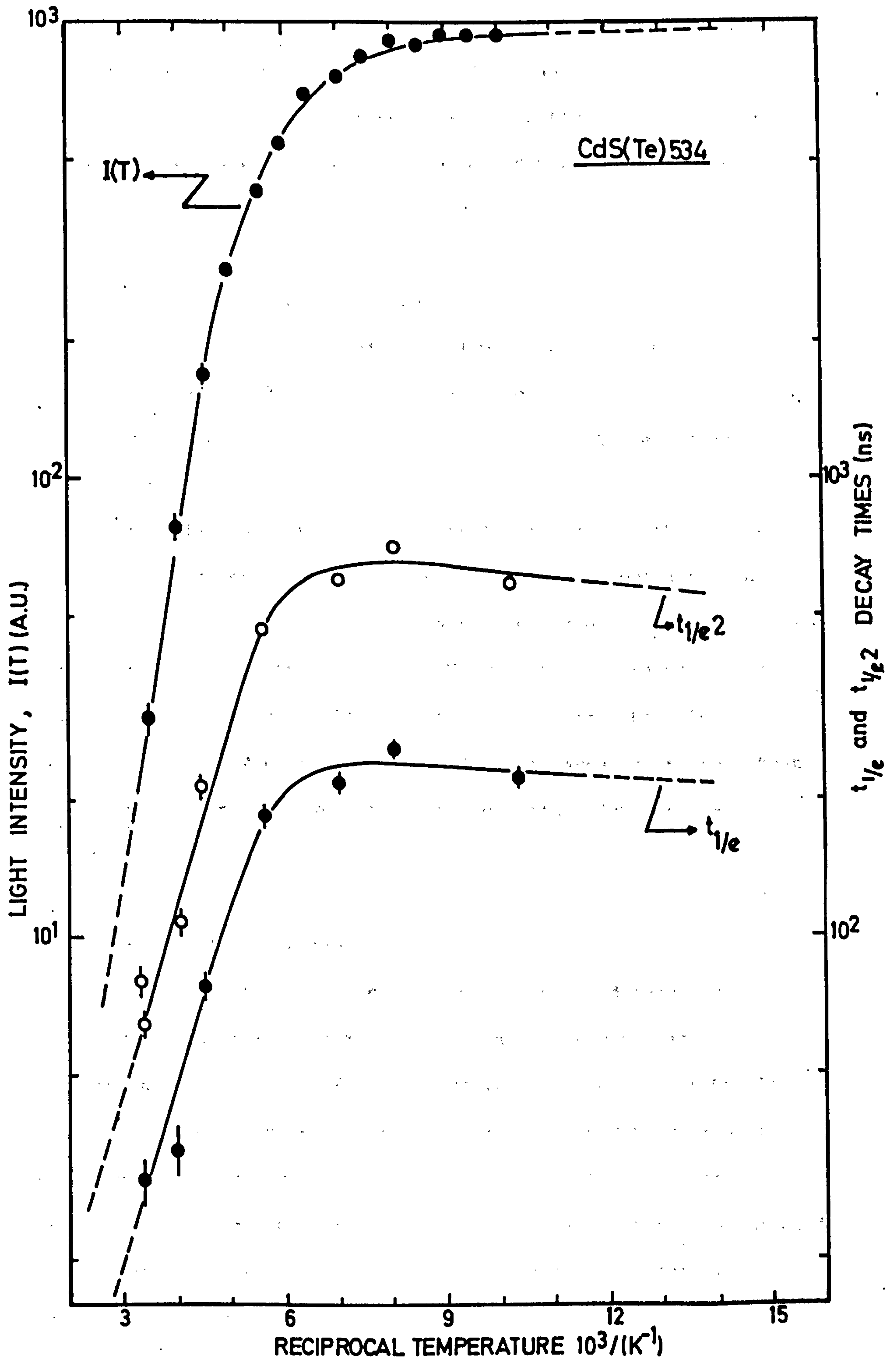
FIGURE 5.14 Variations of decay times and intensity of beta-induced luminescence with temperature in CdS(Te)534Si.
