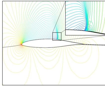
Fig. 2. Baseline at 45%c transition.
