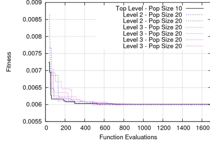
Fig. 3. Convergence at 0% c transition. Fig. 4. Convergence at 45% c transition.
