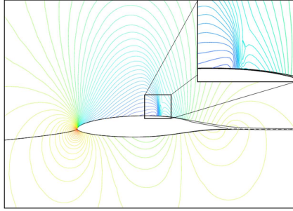
Fig. 5. C_p contour obtained by optimal SCB at 0% trans.
