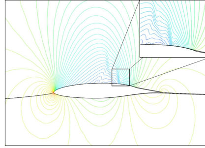
Fig. 6. C_p contour obtained by optimal SCB at 45% trans.
