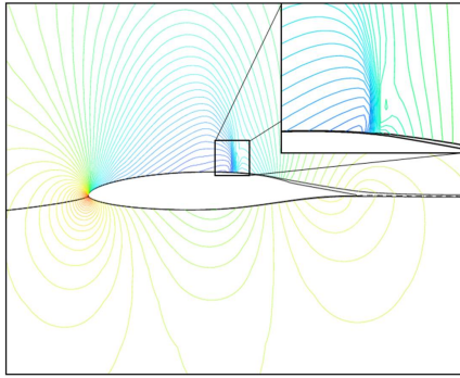
Fig. 1. Baseline at 0%c transition.
