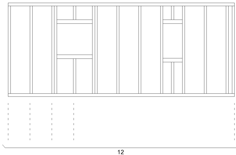
Figure 1. Perspective for building a timber wall
