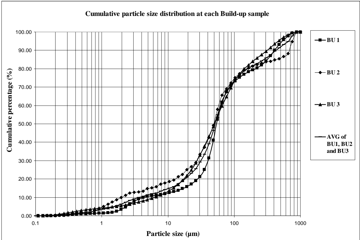
Fig 5. Cumulative particle size distribution of each build-up sample.
