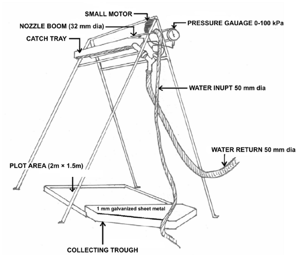
Fig 2. Schematic diagram of the rainfall simulator used for the study ,Adapted from Herngren et al.
