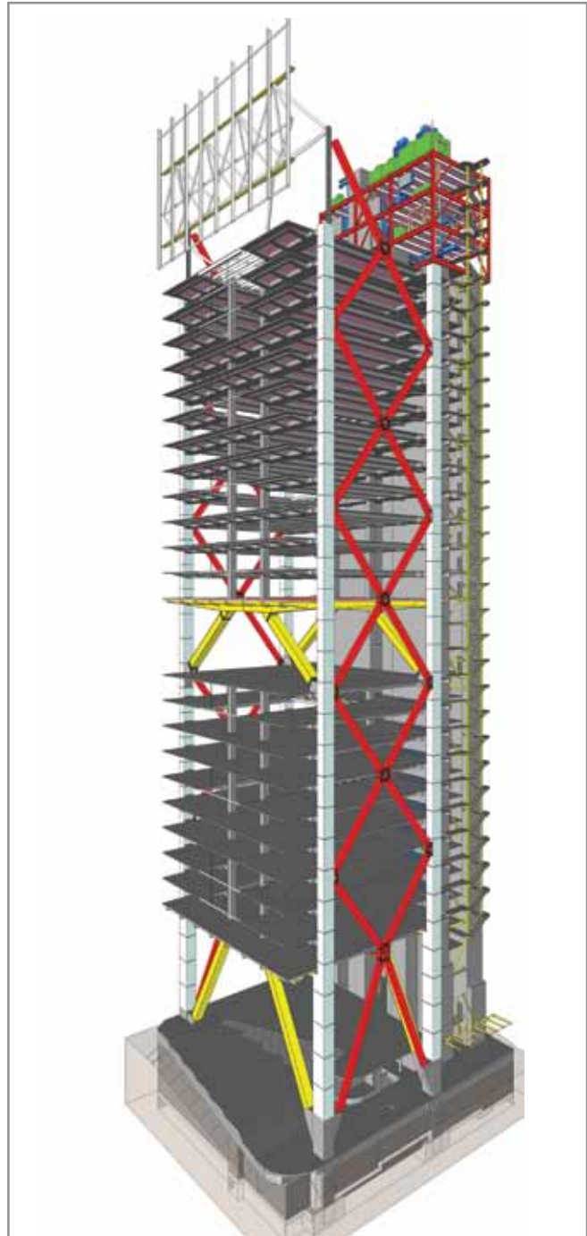
Figure 3.5 Structural model of 8 Chifley Square
