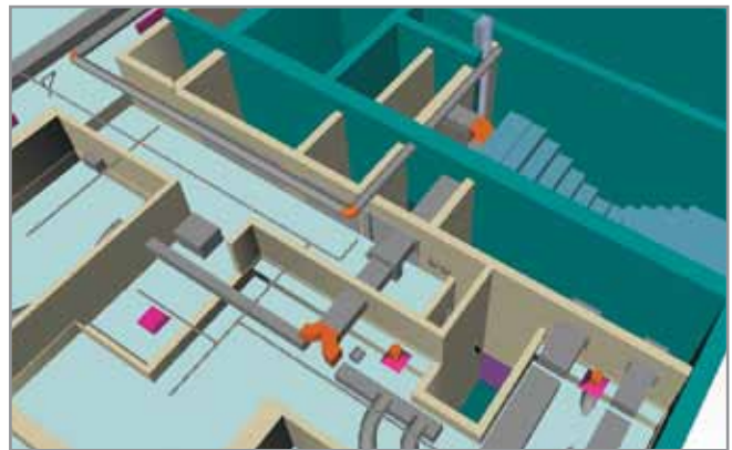
Fig: A1.7 Services modelling example
