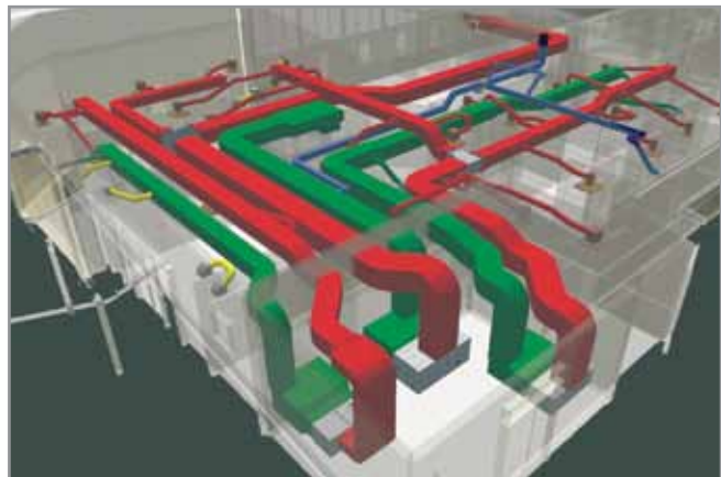
Figure 3.8 Northlakes Police Station detailed HVAC model
