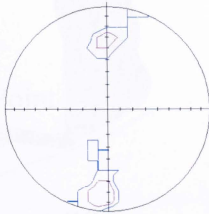
Contouring of poles to principal faults
