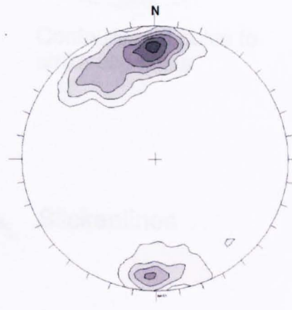
Contouring of poles to faults
