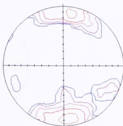
Contouring of poles to vein
