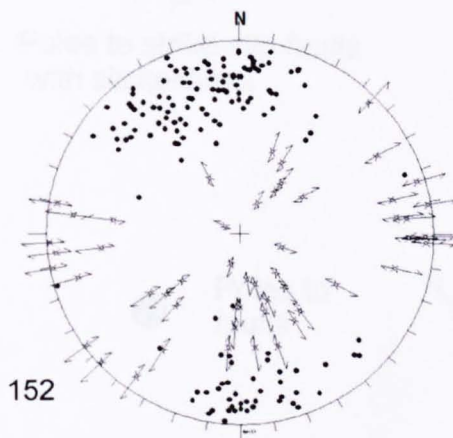
Poles to faults and slickenlines
