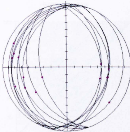
Reverse shear planes and slickenlines
