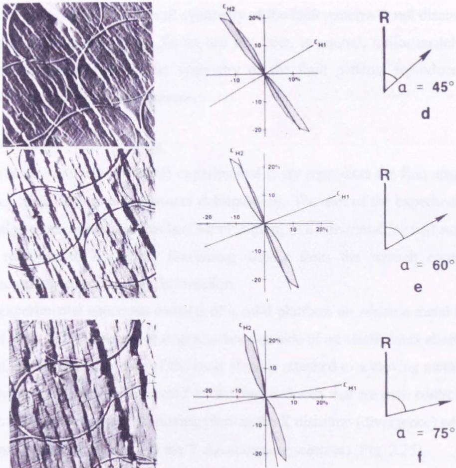
Figure 2.24: d-e-f) Photograph of the clay surface and corresponding rose diagrams of fault trends for the extension-dominated transtension, 30^\circ < \alpha < 90^\circ (after Withjack and Jamison, 1986).
