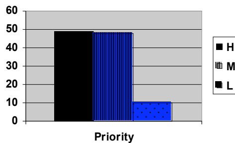
Figure 3. A standard histogram of the “Priority” attribute.
