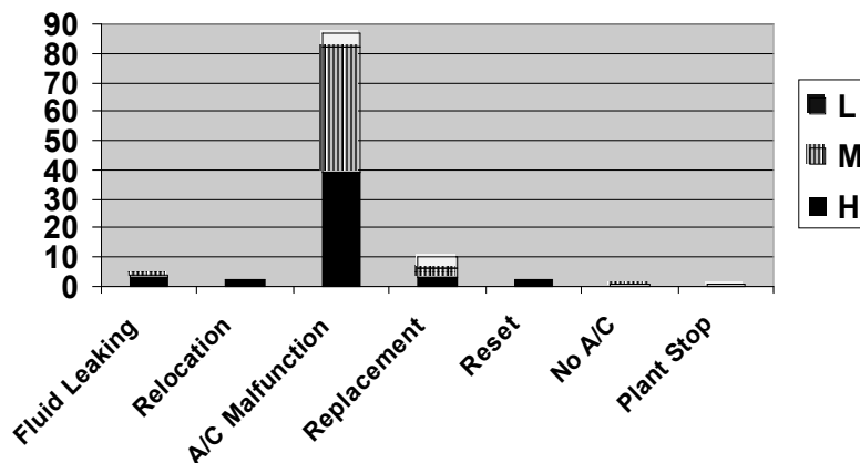
Figure 4. A stacked histogram of correlation between “Priority” and “Cause-of-repair”.
