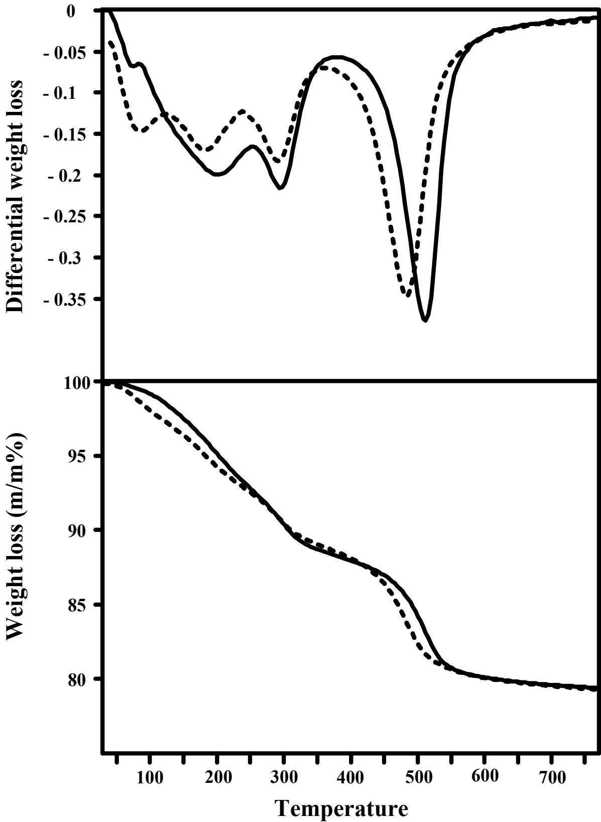
Fig 4b. Thermogravimetric analysis of the Szeg kaolinite mechanochemically activated 3 h and intercalated with 100% formamide (----non-aged, ——aged six months).
