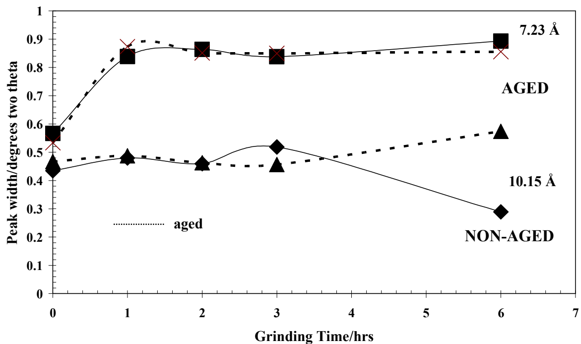
Figure 3a Variation of the relative intensity of the d(001) peaks with grinding time after 1 year of ageing.
