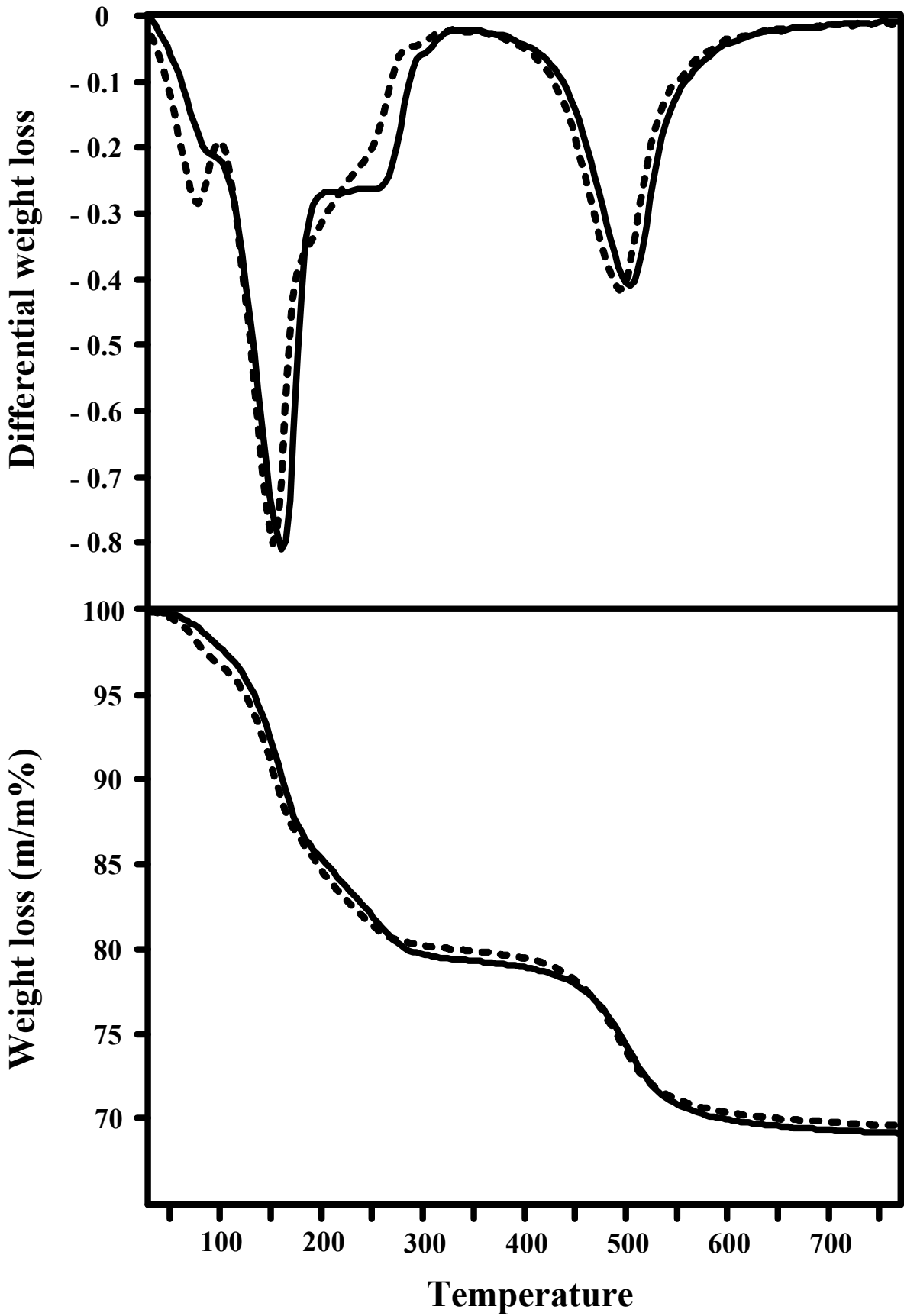
Fig 4a. Thermogravimetric analysis of the Szeg kaolinite mechanochemically activated 0 h and intercalated with 100% formamide (----non-aged, ——aged six months)
