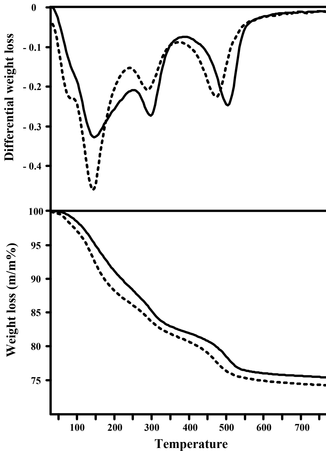
Fig 4c. Thermogravimetric analysis of the Szeg kaolinite mechanochemically activated 6 h and intercalated with 100% formamide (----non-aged, ——aged six months).
