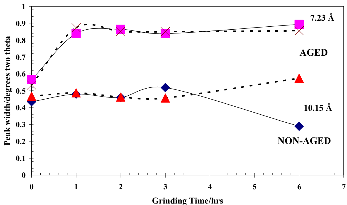
Figure 3b Variation of peak width of the d(001) peaks with grinding time after 1 year of ageing.
