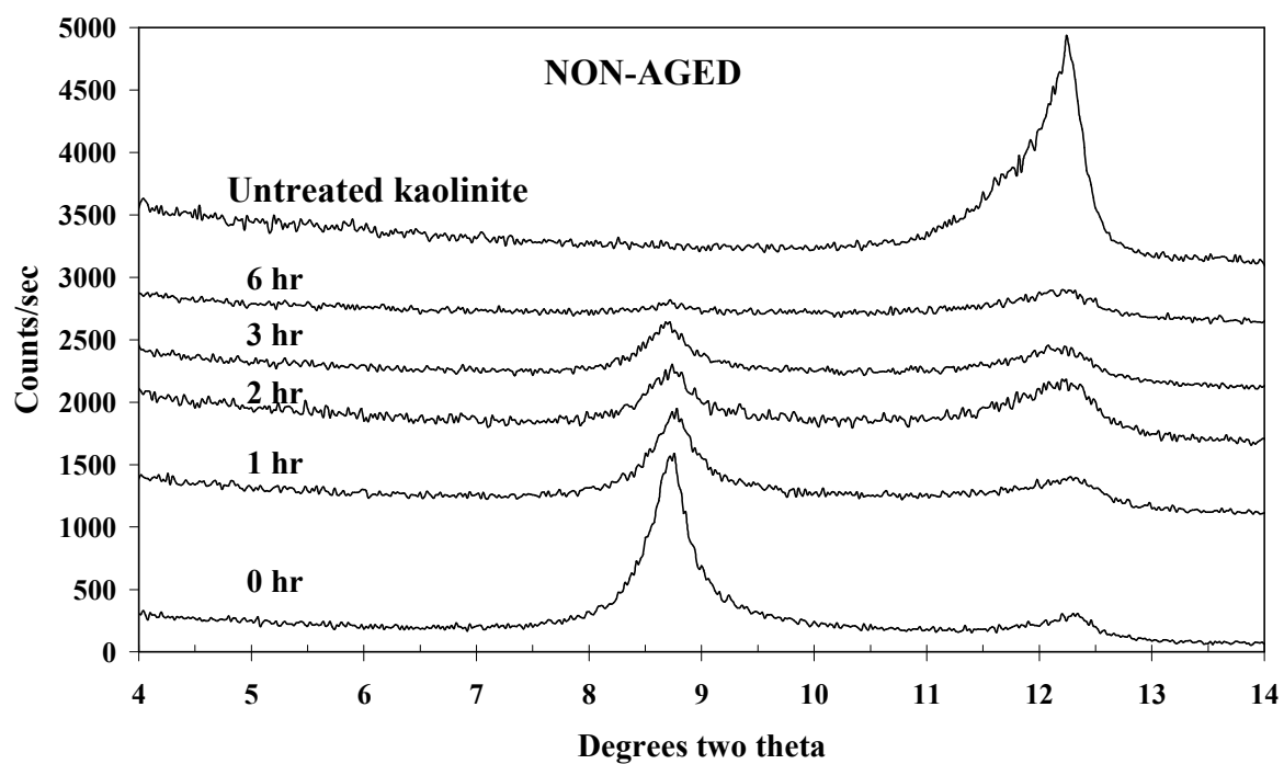
Figure 2 X-ray diffraction of kaolinite mechanochemically activated and intercalated with formamide (a) non-aged (b) aged.
