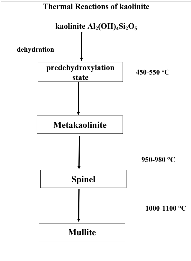
Figure 1 Summary of the thermal transformations of kaolinite
