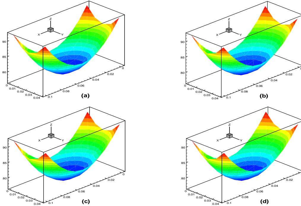
Fig. 3. Results on mesh (iii) for an isotropic case, k_{xx} = k_{yy} = 1.2 , h = 10 . (a) Exact Solution, (b) LSPR, (c) LSF, (d) LSGR.
