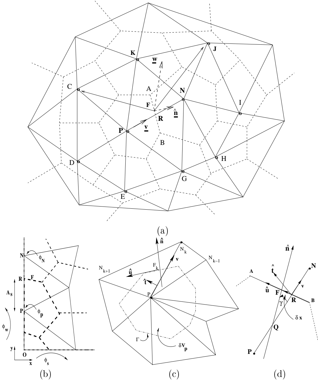
Fig. 1. (a) An example of a cluster of points used for the least square approximation methods, (b) a boundary control volume, (c) a typical control volume and (d) a control volume face
