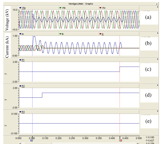
Fig. 8. System response to a SLG fault.
