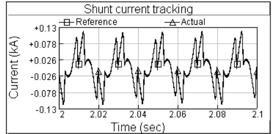
Fig. 13 Shunt current tracking characteristics of phase-a.
