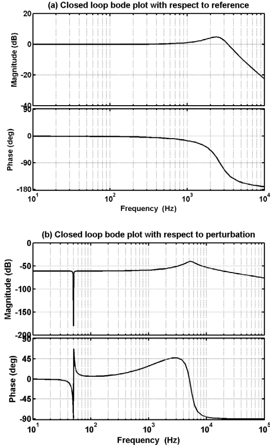
Fig. 9 Closed loop Bode plot (a) with respect to reference shunt current, (b) with respect to the perturbation at PCC.
