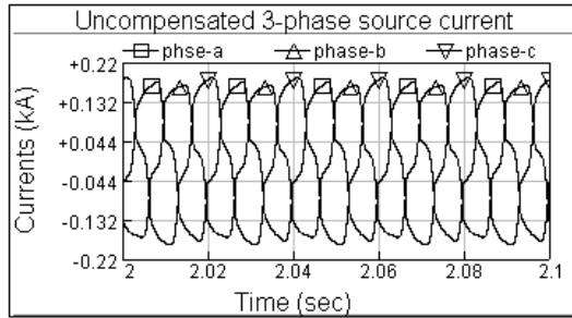
Fig. 10 Three phase source currents for uncompensated distribution system.
