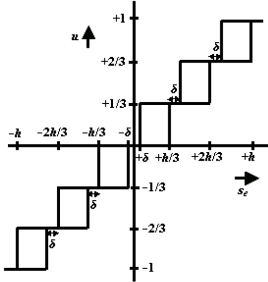
Fig. 3 Seven-level hysteresis modulation.
