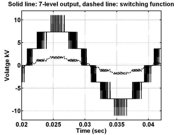
Fig. 5 7-level inverter output voltage v_{oa} and switching function s_{ea} \times 200 .
