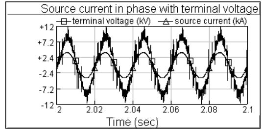
Fig. 12 In-phase source current with terminal voltage for phase-a.
