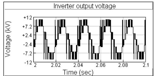
Fig. 14 Inverter output voltage for phase-a.
