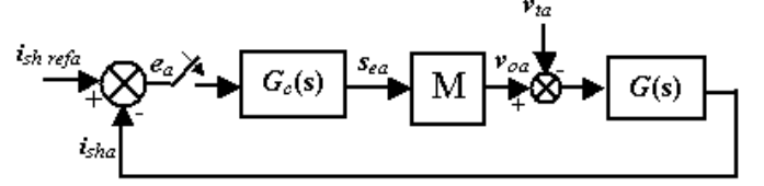
Fig. 7 Current control loop of the DSTATCOM.
