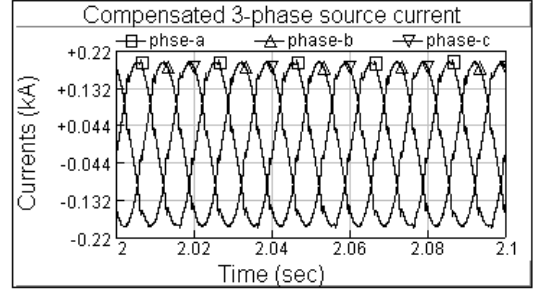
Fig. 11 Three phase source currents for compensated distribution system.
