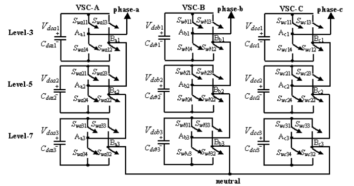
Fig. 4 Cascaded configuration of three-phase seven-level VSC's.
