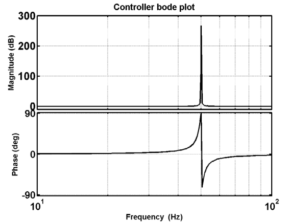
Fig. 8 Bode plot of the proportional plus resonant controller.
