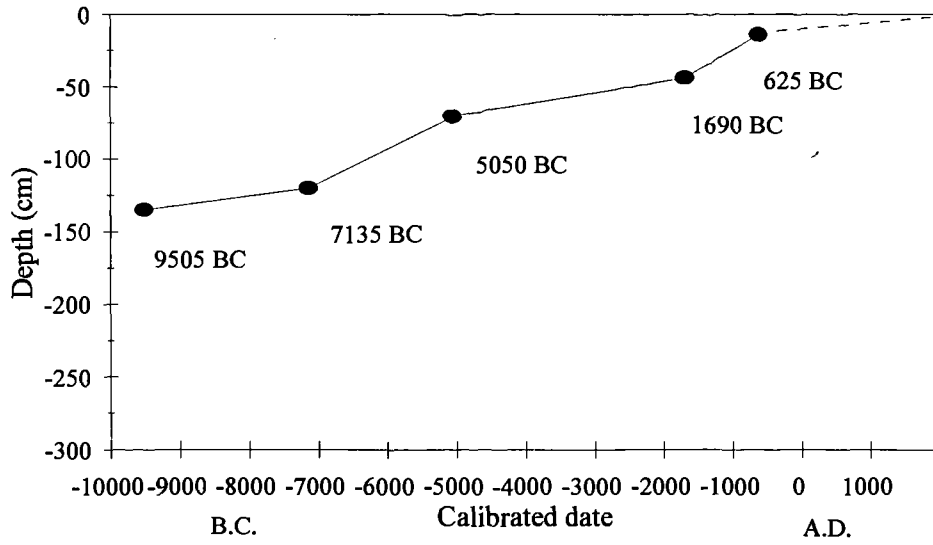
Age-depth curve for Tinkler's Sike
