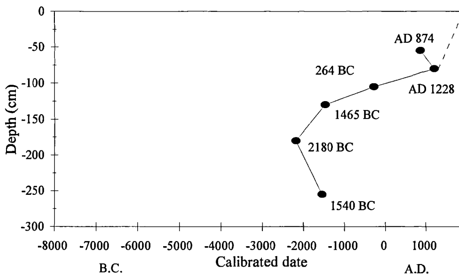
Age-depth curve for Blackpool Moss
