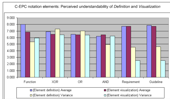
Figure 4: Perceived understandability of C-EPC notation constructs: Results
