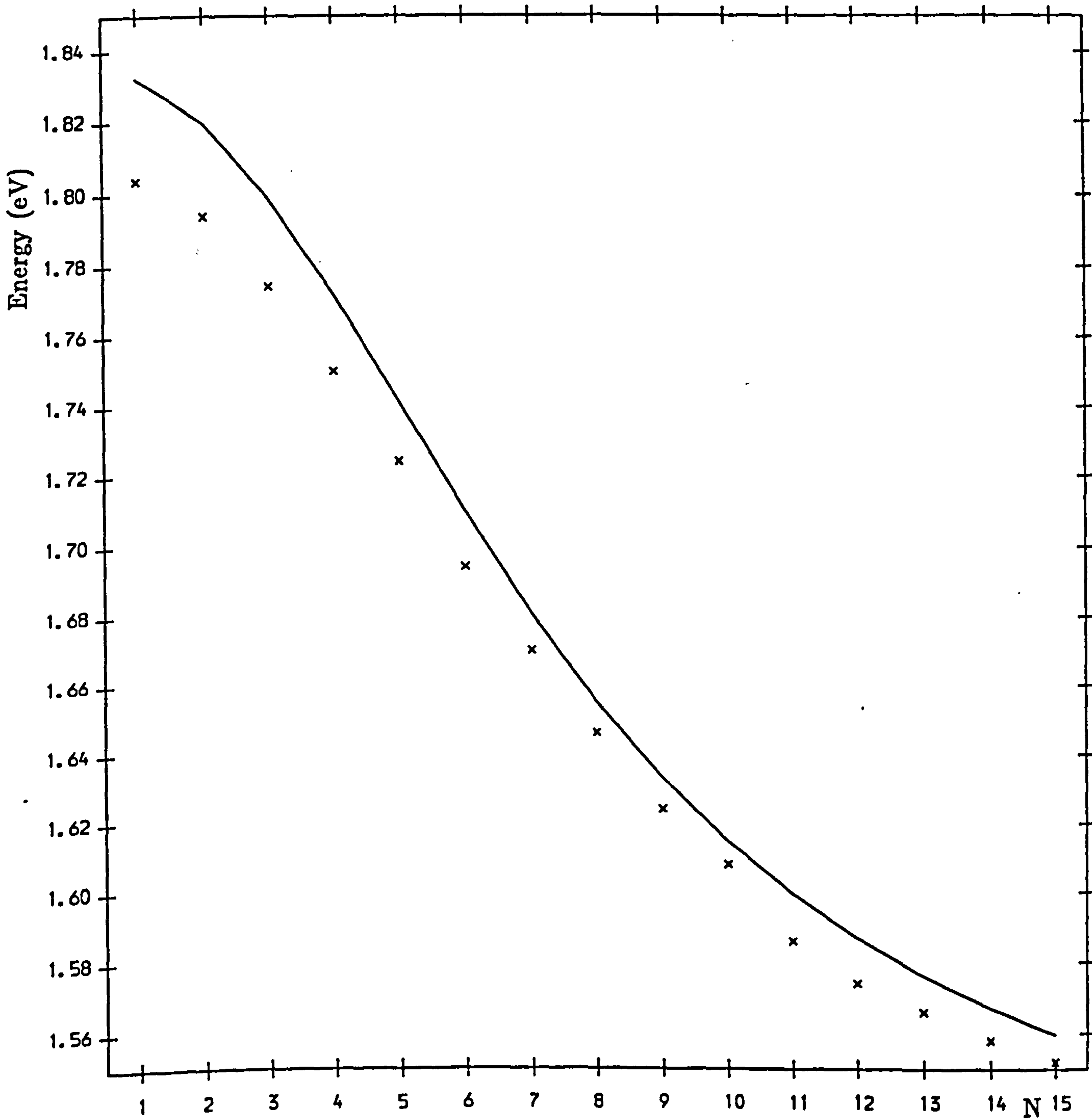
Figure 5.4, Energy levels of the lowest conduction band subband at \bar{\Gamma} of the (\text{CdTe})_N - (\text{ZnTe})_N superlattice with \Delta E_V = +0.060 eV, matching at a plane through the centre of a bond; N varies between 1 and 15. Kronig-Penney results are marked by a full line; pseudopotential results are marked by crosses.
