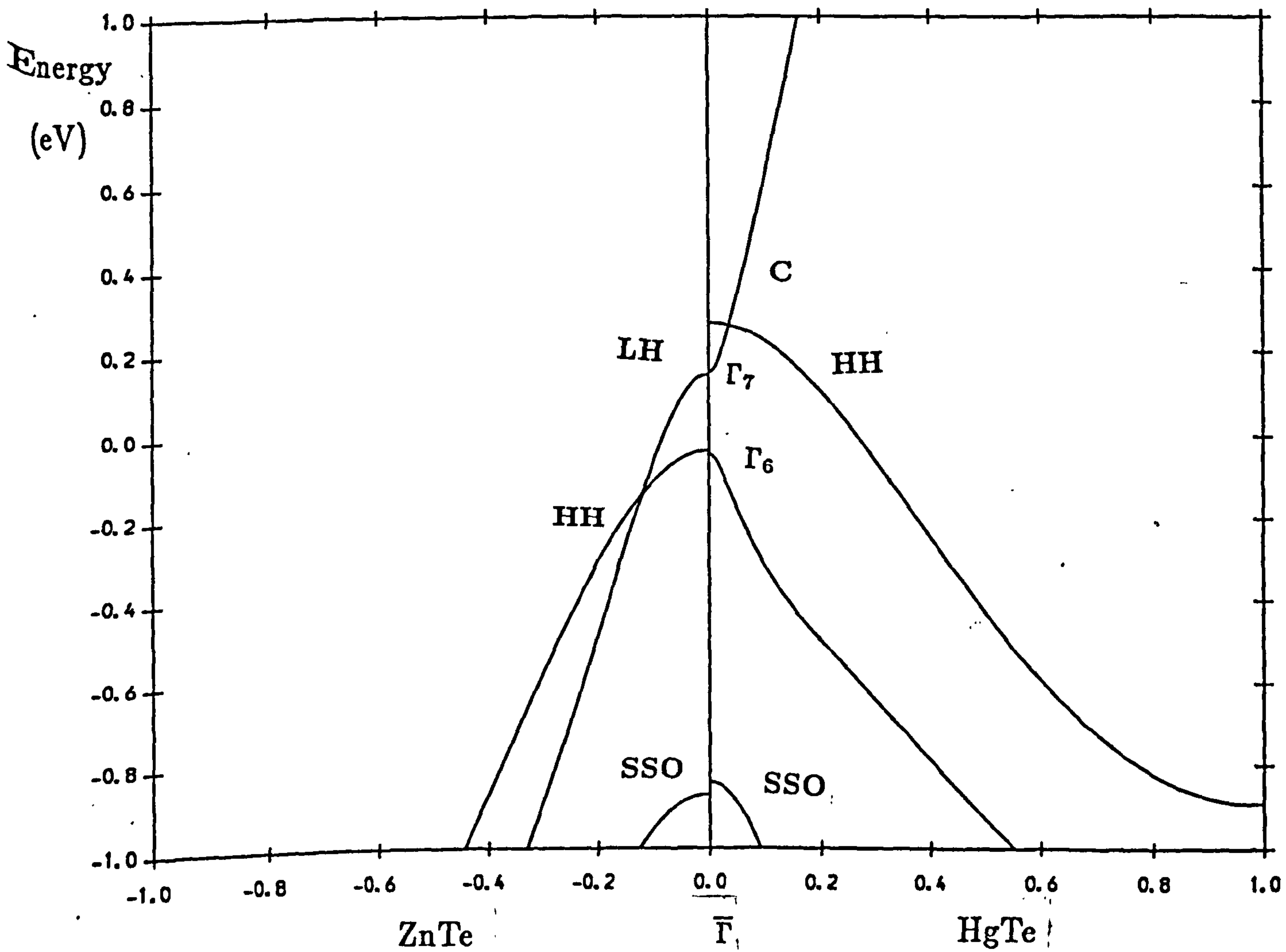
Figure 6.2. Bulk strained bandstructures of HgTe and ZnTe along [100] between E = -1.0 eV and 1.0 eV, with \Delta E_V (HgTe/ZnTe) = 0.25.
