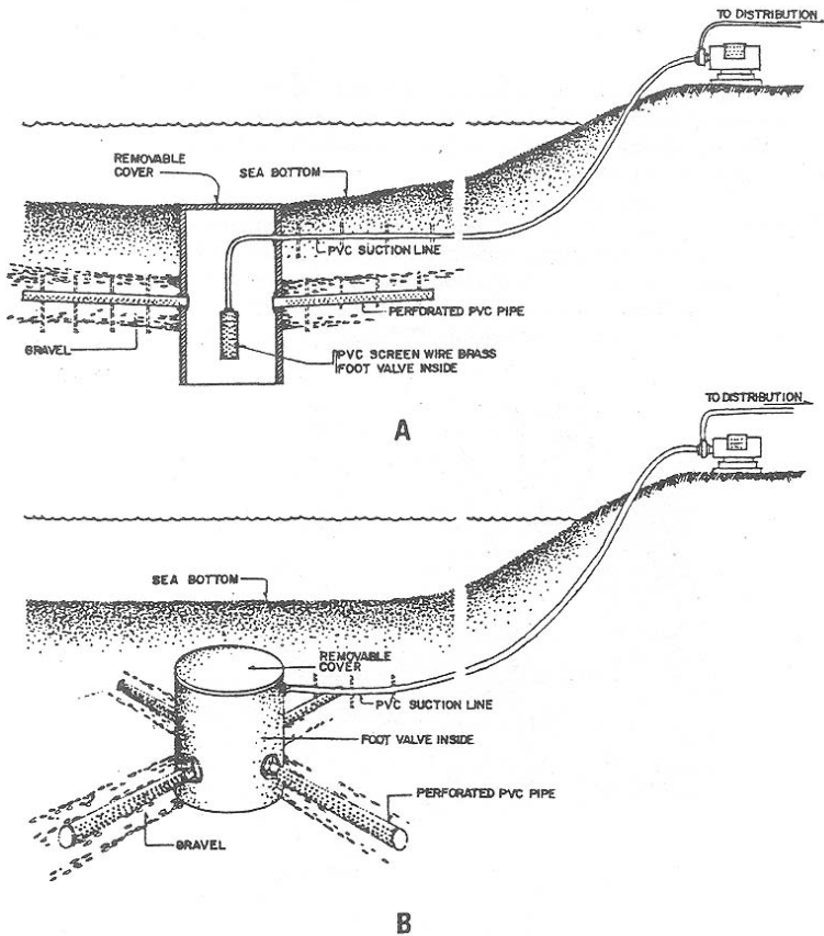
Fig. 9. Commonly used prefiltration systems: graded gravel (A) or concrete suction chamber with perforated PVC pipes (B).
