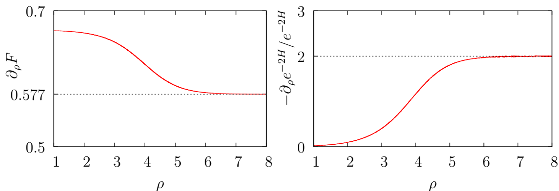
Figure 5.4: Holographic RG flow from the 6D spacetime (5.21) to the \varphi^2 = 0.45 AdS solution. F = \rho , \beta = 0 throughout this flow.
