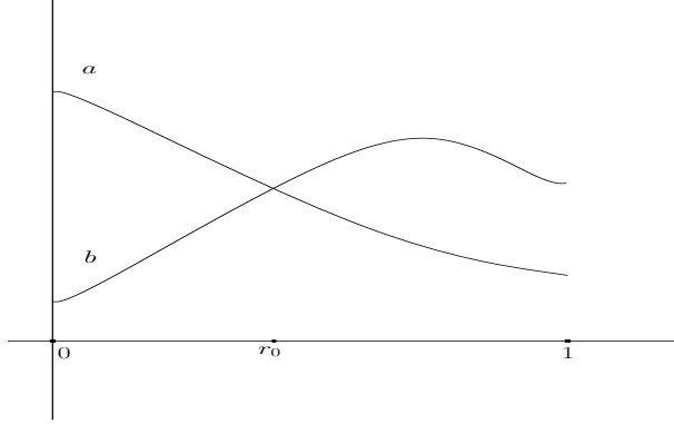
Figure 1: The graphs of a, b .
