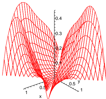
FIGURE 1. Plot of \Phi for r = 3 .
