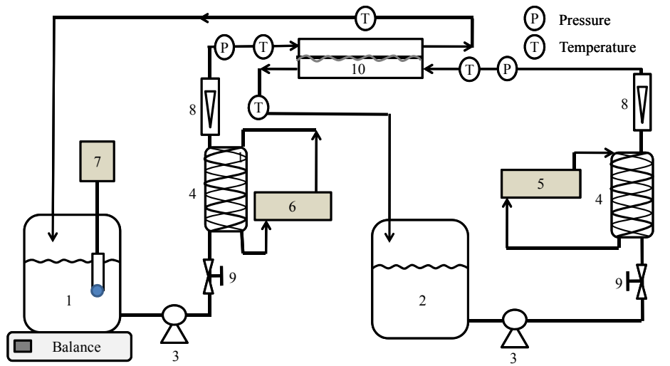
1. Permeate tank, 2. Feed tank, 3. Pump, 4. Heat Exchanger, 5. Heater, 6. Chiller, 7. Conductivity meter, 8. Flow meter, 9. Flow controller, 10. Membrane
