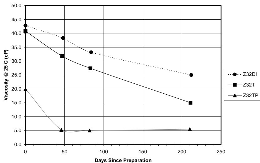
Figure 1: Effect of ageing Zetac 32 solutions on solution viscosity. (DI= de-ionised water, T = tap water, TP = tap water with 2.5% w/v pine-o-clean).
