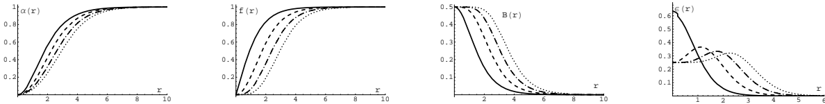
Figure 1. Plots of the field profiles l(r) (a) and f(r) (b); the magnetic field B(r) (c), and the energy density \epsilon(r) for self-dual vortices with l=1 (solid line), l=2 (dashed line), l=3 (broken-dashed line) and l=4 (dotted line).
