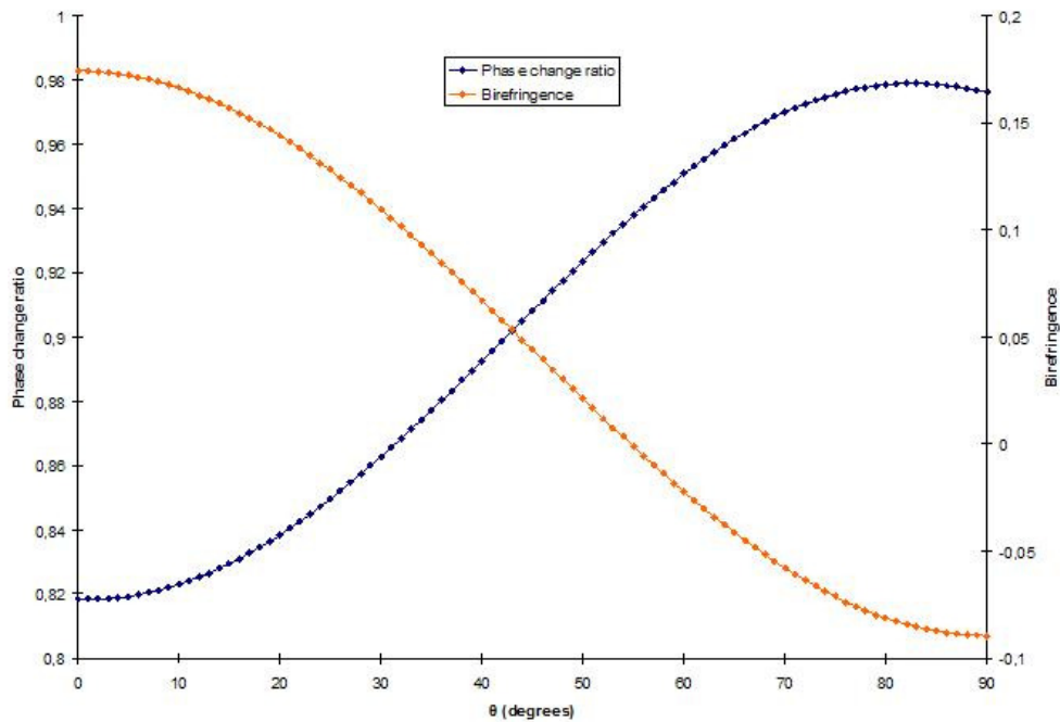
Figure 3.11 – Simulation of the evolution of the phase change ratio according to the polar angle (blue curve), and birefringence determined from Figure 3.10 for comparison (orange curve).
