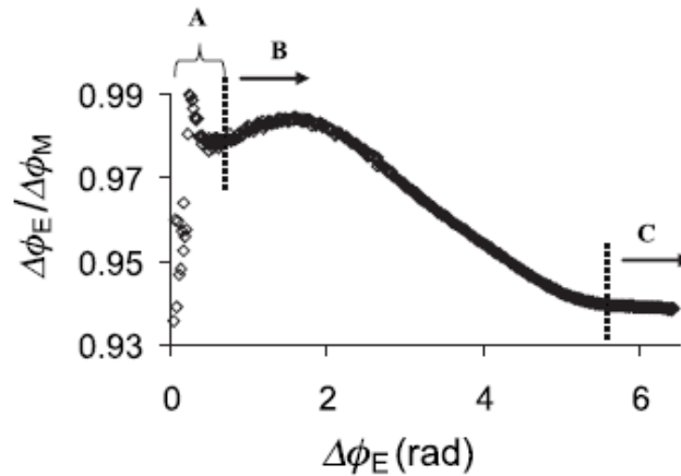
Figure 2.19 – Evolution of the phase change ratio as the amount of deposited material increases (i.e. increase of the phase change) [32].
