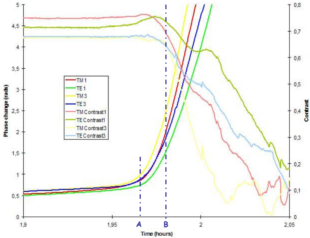
Figure 5.3 – Sudden phases increase (event A) and contrasts drop (event B) observed for the water test in high RH (Section 4.1.2.2).
