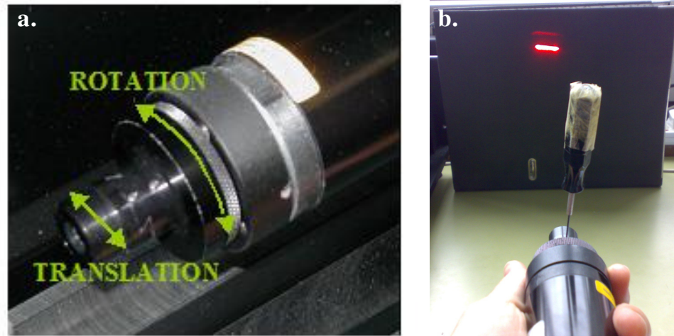
Figure 3.1 – (a) Degrees of freedom for Powell lens adjustment. (b) Optical power repartition on the laser line checked by pointing the laser toward a wall.
