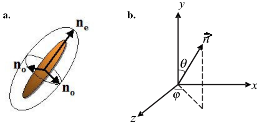
Figure 2.17 – (a) Intrinsic index ellipsoid of a liquid crystal molecule pointing toward the director of the nematic phase. (b) Description of the director in the chip frame.
