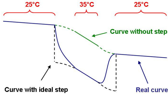
Figure 5.7 – Model for the birefringence evolution when the chip temperature changes between 25 °C and 35 °C.
