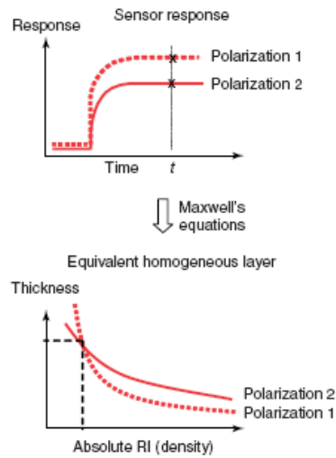
Figure 2.2 – Resolving the 2 measurements from orthogonal polarizations can converge on a unique solution for thickness and RI of an isotropic adlayer [11].
