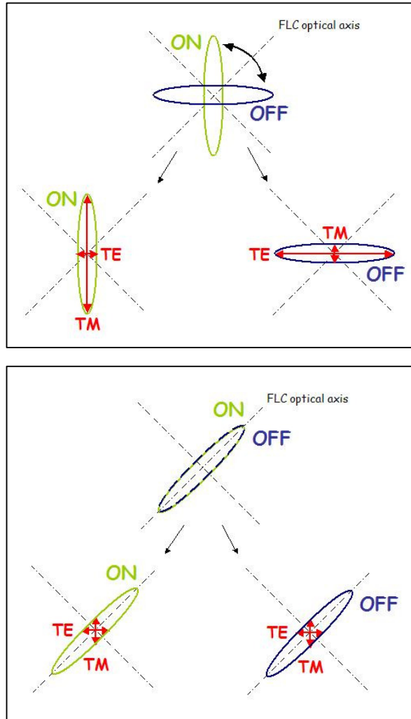
Figure 3.4 – Schematics representing the modes coupled into the chip (red arrows) according to the orientation of the laser with regards to the FLC axis: on the upper picture the laser is well-oriented, whereas it is not on the lower picture.
