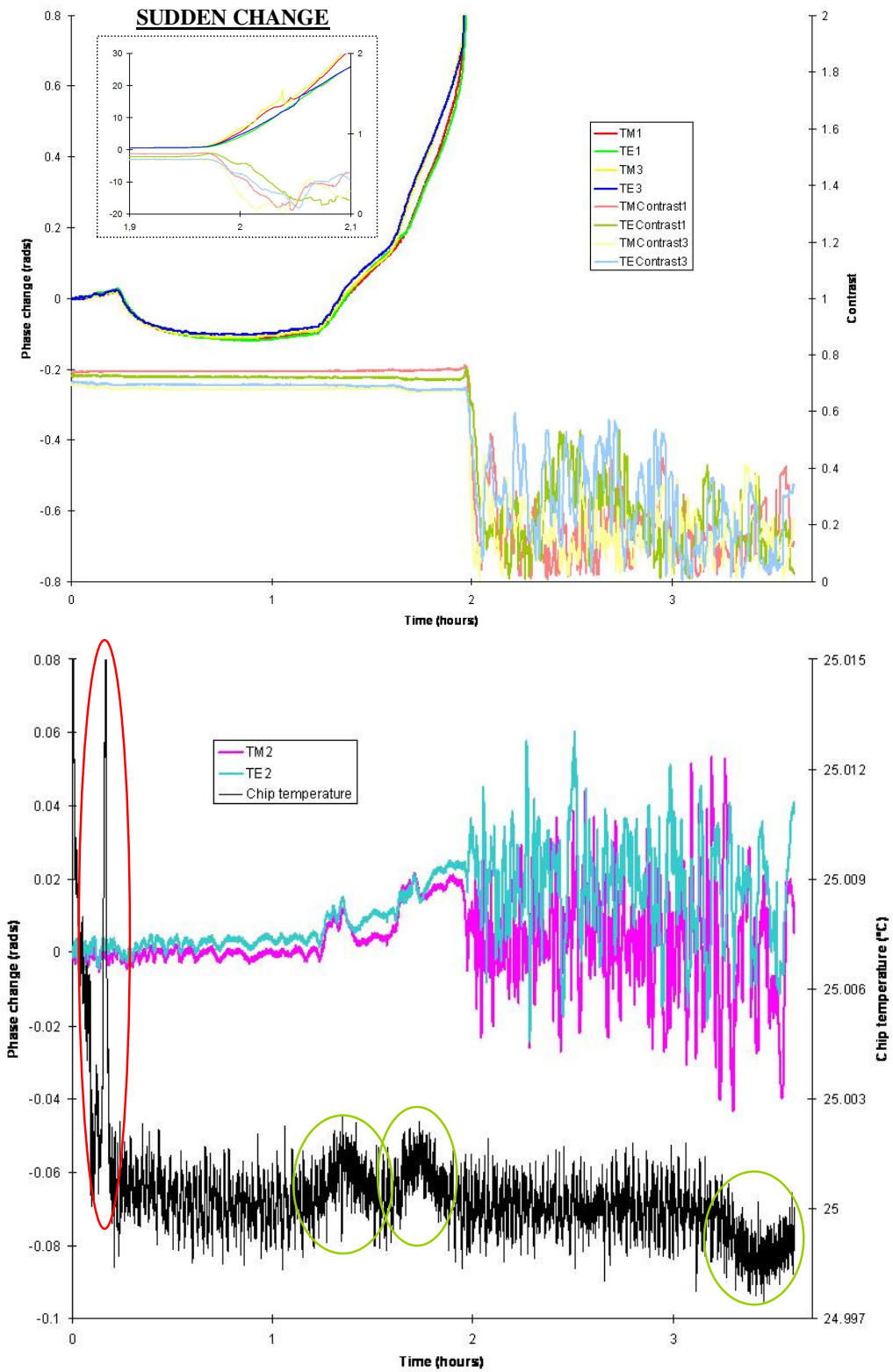
Figure 4.3 – Desorption of water molecules, and re-adsorption for the chip exposed to high RH.
