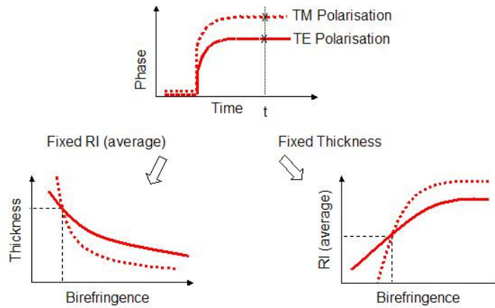
Figure 2.3 – For anisotropic adlayers, it is required to fix one parameter to get the 2 others from the 2 experimental measurements.
