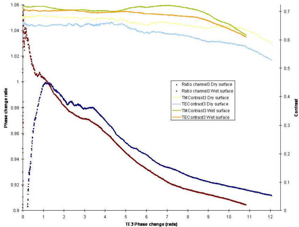
Figure 5.4 – Phase change ratios for LC deposition on dry and wet surface, with associated TE and TM contrasts.
