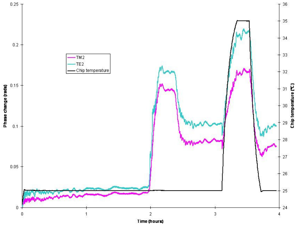
Figure 4.8 – Reference test associated to LC experiment on nitrogen dried surface.
