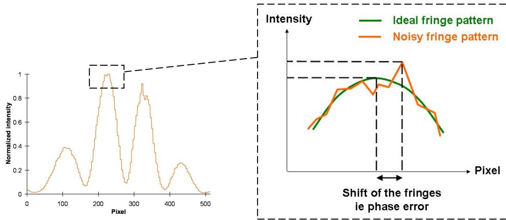
Figure 2.8 – Schematic showing how the optical noise causes an error during the phase calculation.
