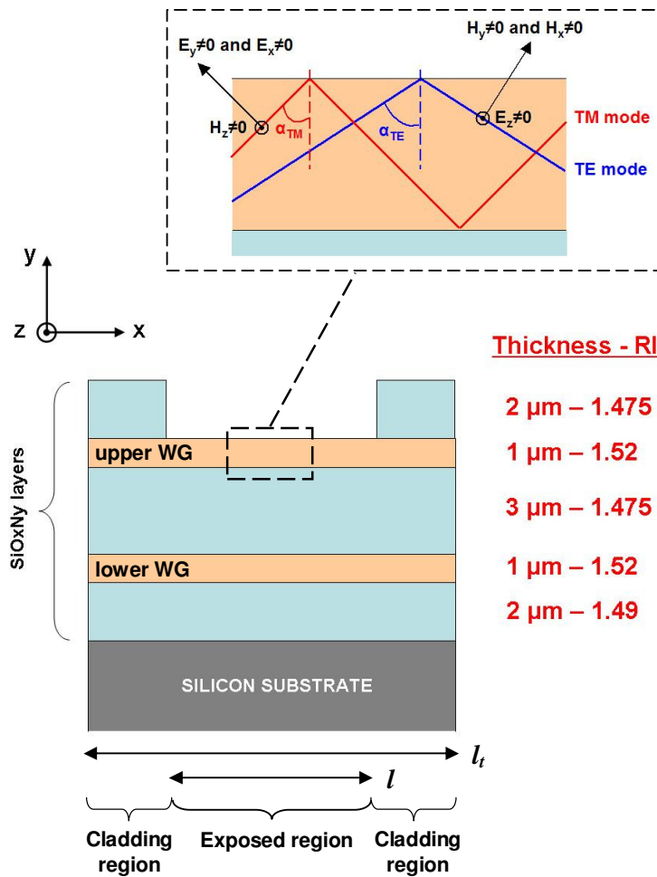
Figure 2.4 – Ideal chip structure with conventions (bottom), and fundamental differences between TE and TM modes (top).
