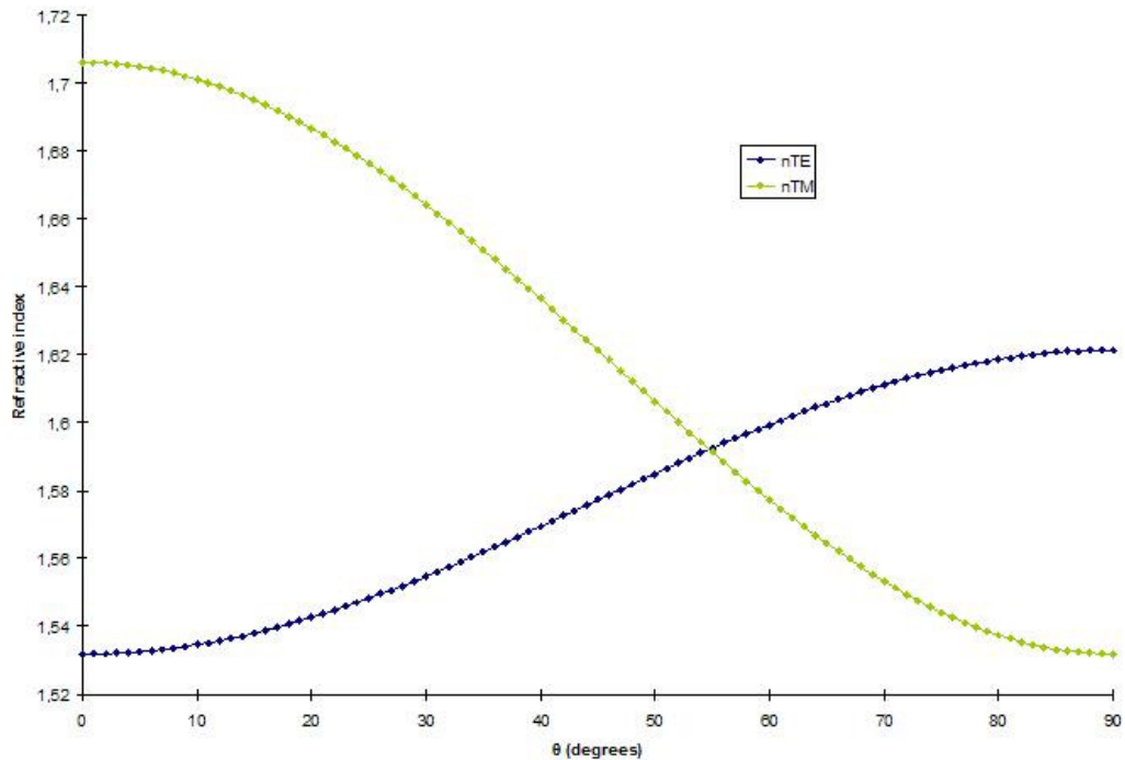
Figure 3.10 – Simulation of the evolution of the adlayer RIs sensed by TE and TM polarizations according to the polar angle.
