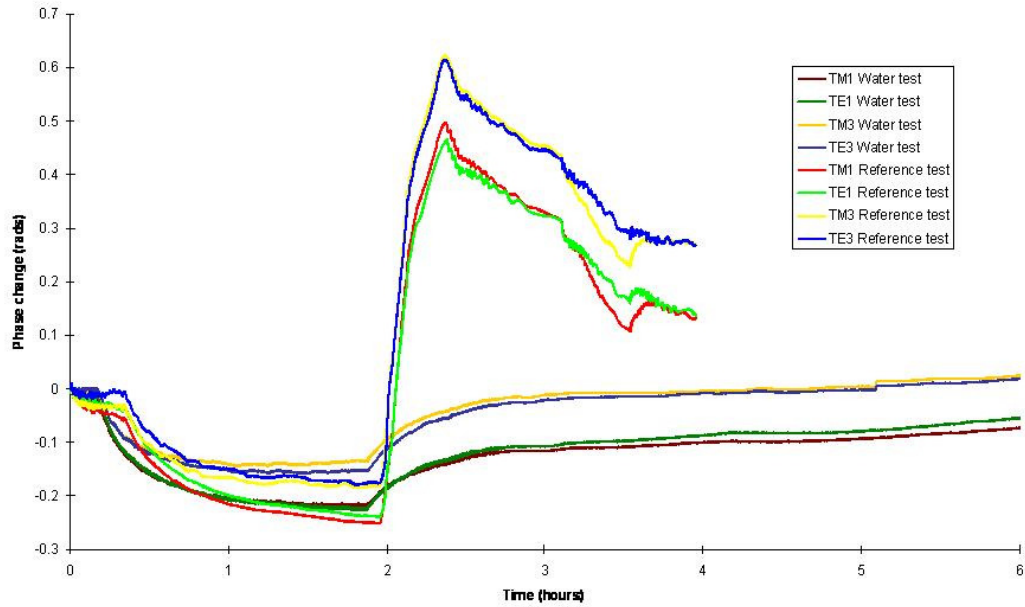
Figure 5.2 – Comparison between the reference test associated to LC experiment on nitrogen dried surface ( Figure 4.8 ) and the water test for the chip exposed to ambient RH ( Figure 4.2 ).
