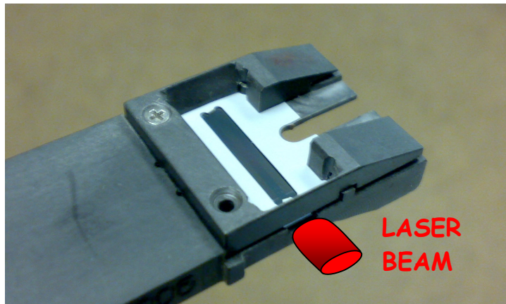
Figure 3.5 – Unmodified INEX FB80 chip in its carrier, with a gasket on it which leaves channels 1 to 3 opened to their environment.
