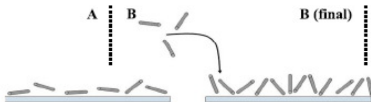
Figure 2.20 – Schematic diagram of molecular re-orientation driven by strong surface anchoring during layer densification (self-organization) [32].
