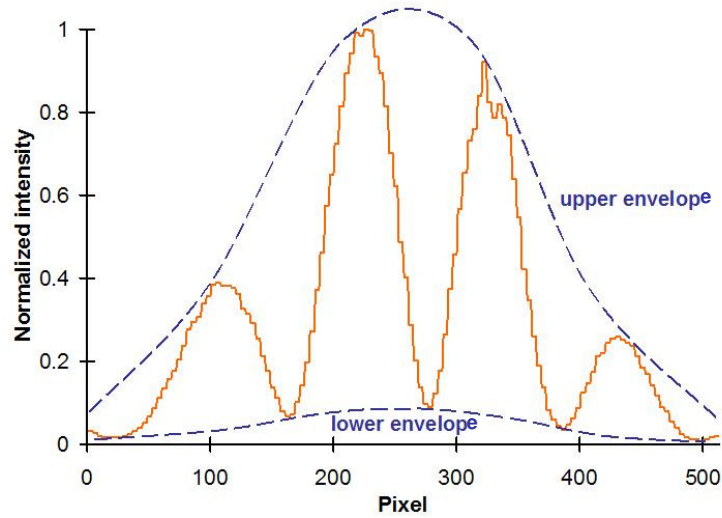
Figure 2.7 – Typical experimental fringe profile given by a software from the image recorded by the CCD camera in the far field (for the chip used in this study).
