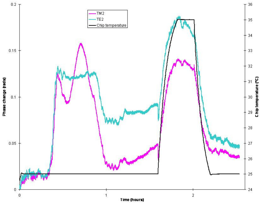
Figure 4.5 – Adsorption and desorption of LC molecules on wet surface (no drying process performed initially).
