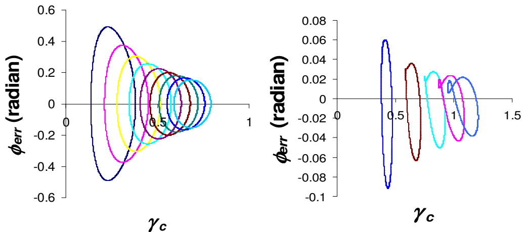
Figure 2.10 – Correlation between phase error and contrast of a noisy fringe pattern for a range of scattering loss coefficients (the higher the surface scattering loss, the lower the average contrast). (left) Correlation for a basic algorithm. (right) Correlation for an improved algorithm [14].
