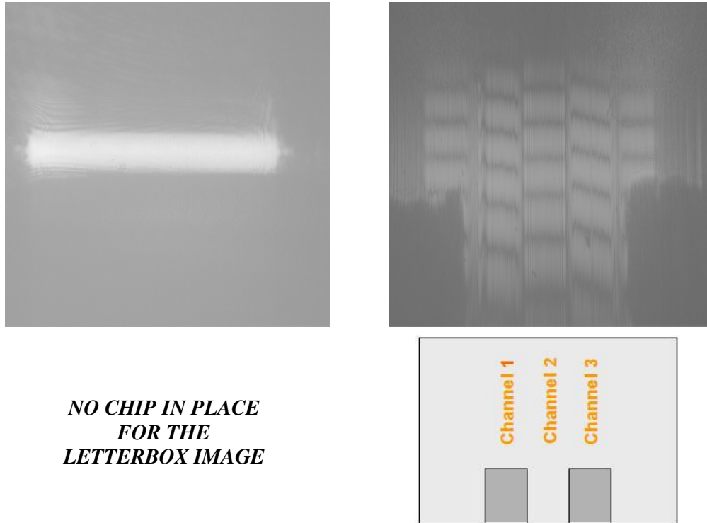
Figure 3.2 – (left) Letterbox image with no chip in place. (right) 5 sets of fringes from the chip in place corresponding to the 3 cladding regions intercalated with the 2 exposed regions.
