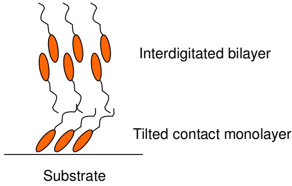
Figure 2.16 – Typical anchoring configuration of nCB on bare silica-like surfaces [14].
