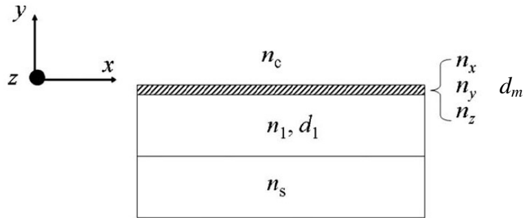
Figure B.1 – Structure defined in order to use the transfer matrix method knowing that n_s , n_1 , d_1 , and n_c are known, d_m is a variable, and n_x , n_y , and n_z can be calculated for a given polar angle [32].
