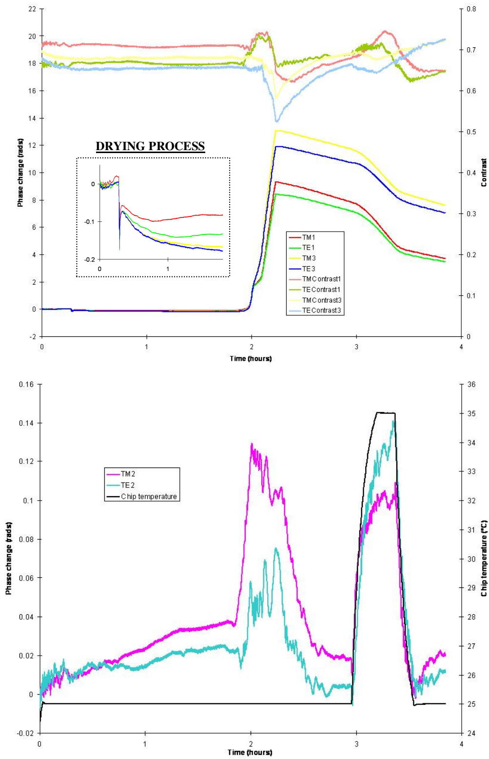
Figure 4.6 – Adsorption and desorption of LC molecules on nitrogen dried surface.
