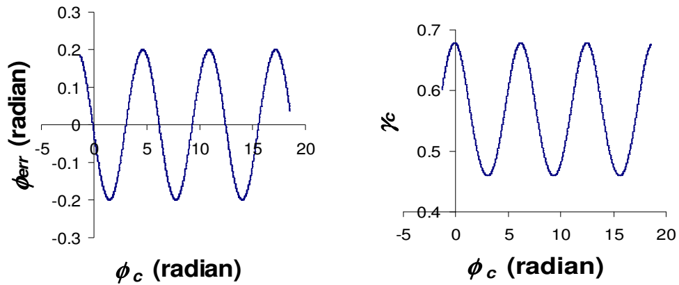
Figure 2.9 – Simulation showing the 2\pi -periodicity of the phase error (left) and contrast (right) plotted against phase for a noisy fringe pattern [14].
