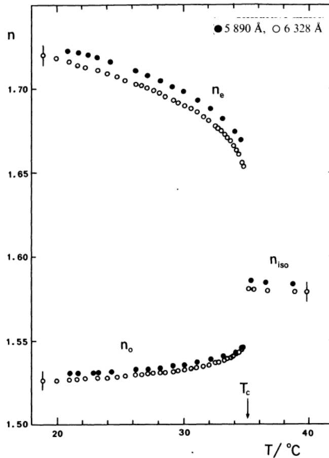
Figure 5.8 – RIs of 5CB as a function of temperature (2 sets according to the wavelength). T_c is the clearing temperature [45].
