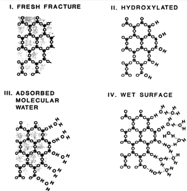
Figure 2.12 – Hydroxylation and adsorption of water on a freshly cleaved fragment of quartz in vacuum [22].
