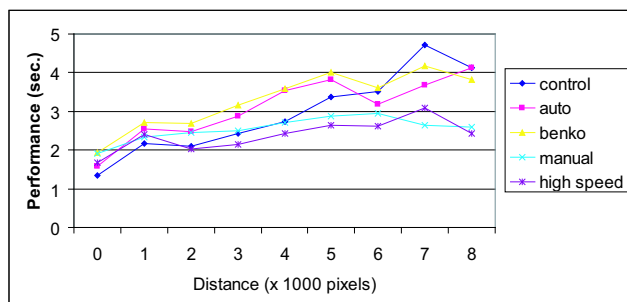
Figure 4. Chart showing how each cursor technique varied in performance as the distance to target increased from left to right for the clicking task. Control cursor is fastest for short range targets, but is overtaken by other techniques for long range targets. High-speed and manual cursors are fastest for long range targets.
