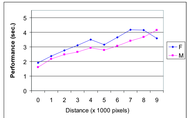
Figure 7. Chart showing the differences in performance for the two genders as the distance to target increased from left to right for the simple drag and drop task. In general, men outperform women by 12%.
