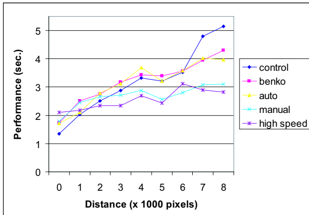
Figure 6. Chart showing how each cursor technique varied in performance as the distance to target increased from left to right for the simple drag and drop task.
