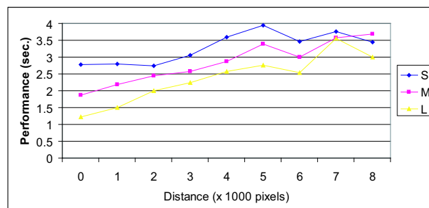
Figure 5. Chart showing the relationship of distance to targets and target size for the clicking task. Performance time increases with distance to target.
