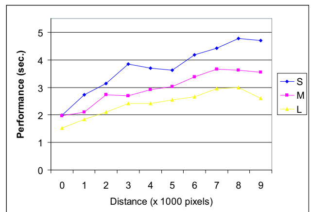
Figure 8. Chart showing the relationship of distance to targets and target size for the simple drag and drop task.
