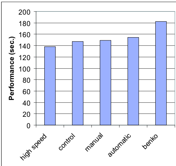
Figure 9. Bar chart showing average performance time of the different cursor techniques used in the complex drag and drop task.
