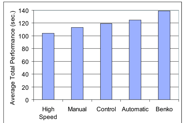
Figure 3. A chart showing the summary results of all three tasks. The high-speed cursor (DSS 1) was significantly faster than the Benko technique.
