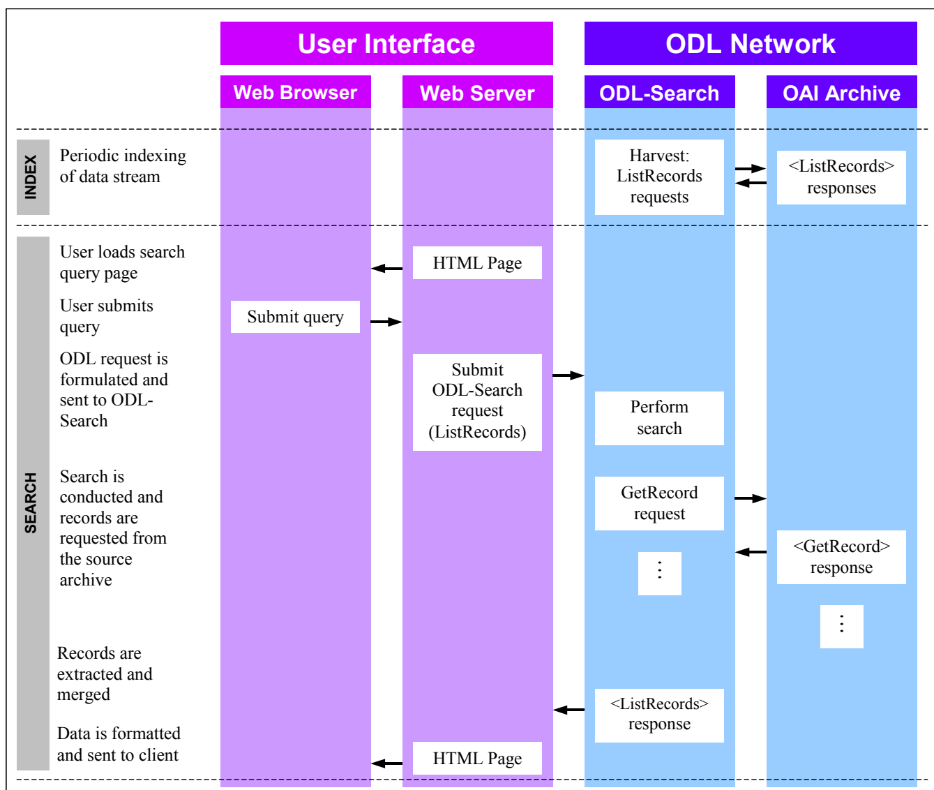
Figure 6. Interface and component interaction during indexing and search operations
