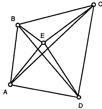
Case 2 : 4 points on the convex hull.
