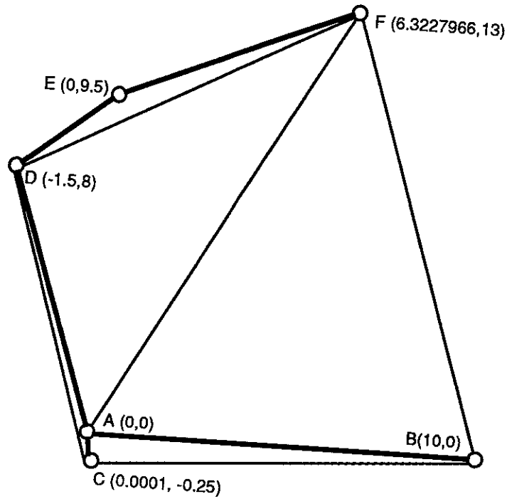
Greedy triangulation
