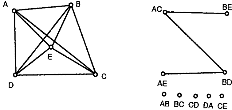
Figure 10: A complete straight line graph and its crossing graph.
