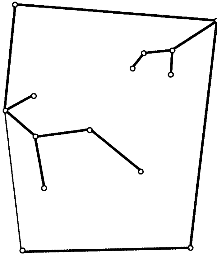
Figure 5: A simple polygon created at the end of step 2 in the MST-T algorithm.
