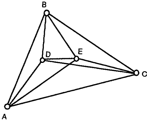
Case 1 : 3 points on the convex hull.
