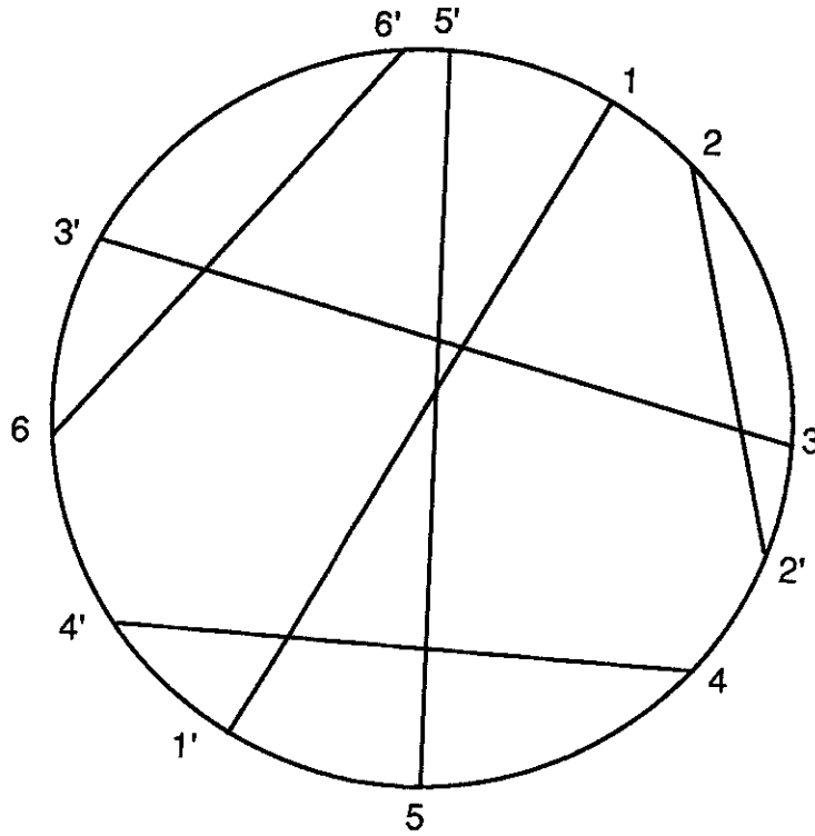
Figure 11: The labeling of the endpoints of the chords of a circle.
