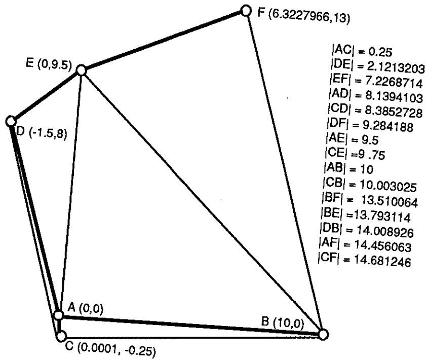
G-ST-T
