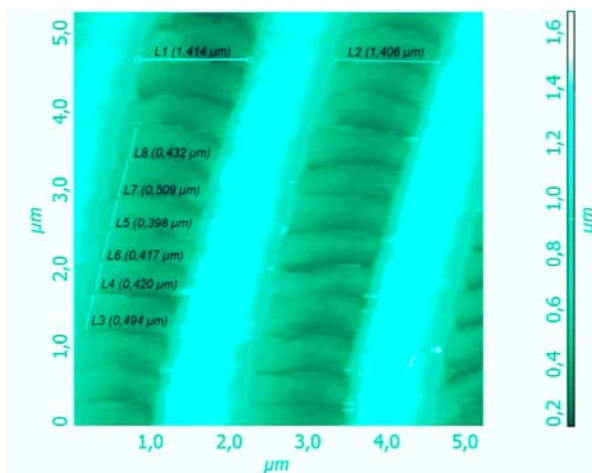
Fig. 10: Morphology of the wing at 70 °C. Average roughness is of 328,742 nm.
