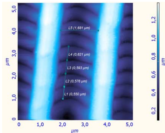
Fig. 9: Morphology of the wing at 40 °C. Average roughness is of 335,513 nm.
