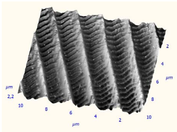
Fig. 2: Morphology of the black area of the wing laminae.
